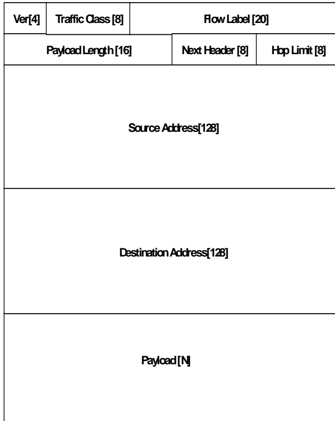
Figure 1 IPv6 Header
