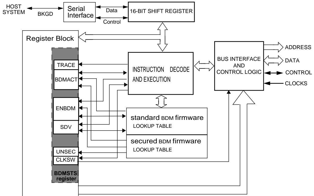
Figure 1-1 BDM Block Diagram
