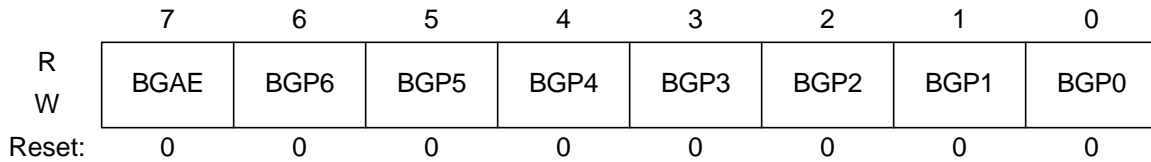
Figure 3-4 BDM Global Page Register (BDMGPR)
