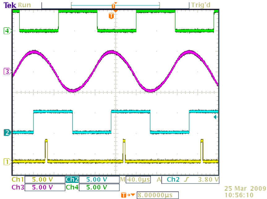
Figure 12 Electrical Signals in Data Synchronization Example
