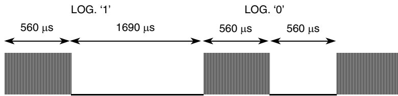
Figure 11. Pulse Distance Protocol, Bit Encoding
