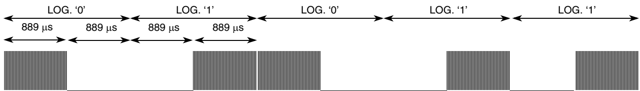
Figure 19. RC5 Protocol, Bit Encoding
