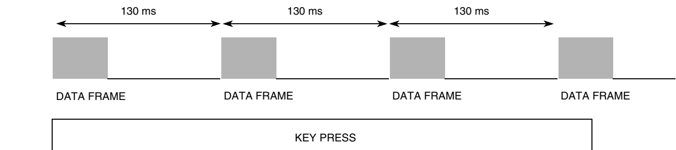
Figure 25. Flash Protocol, Full Sequence Structure
