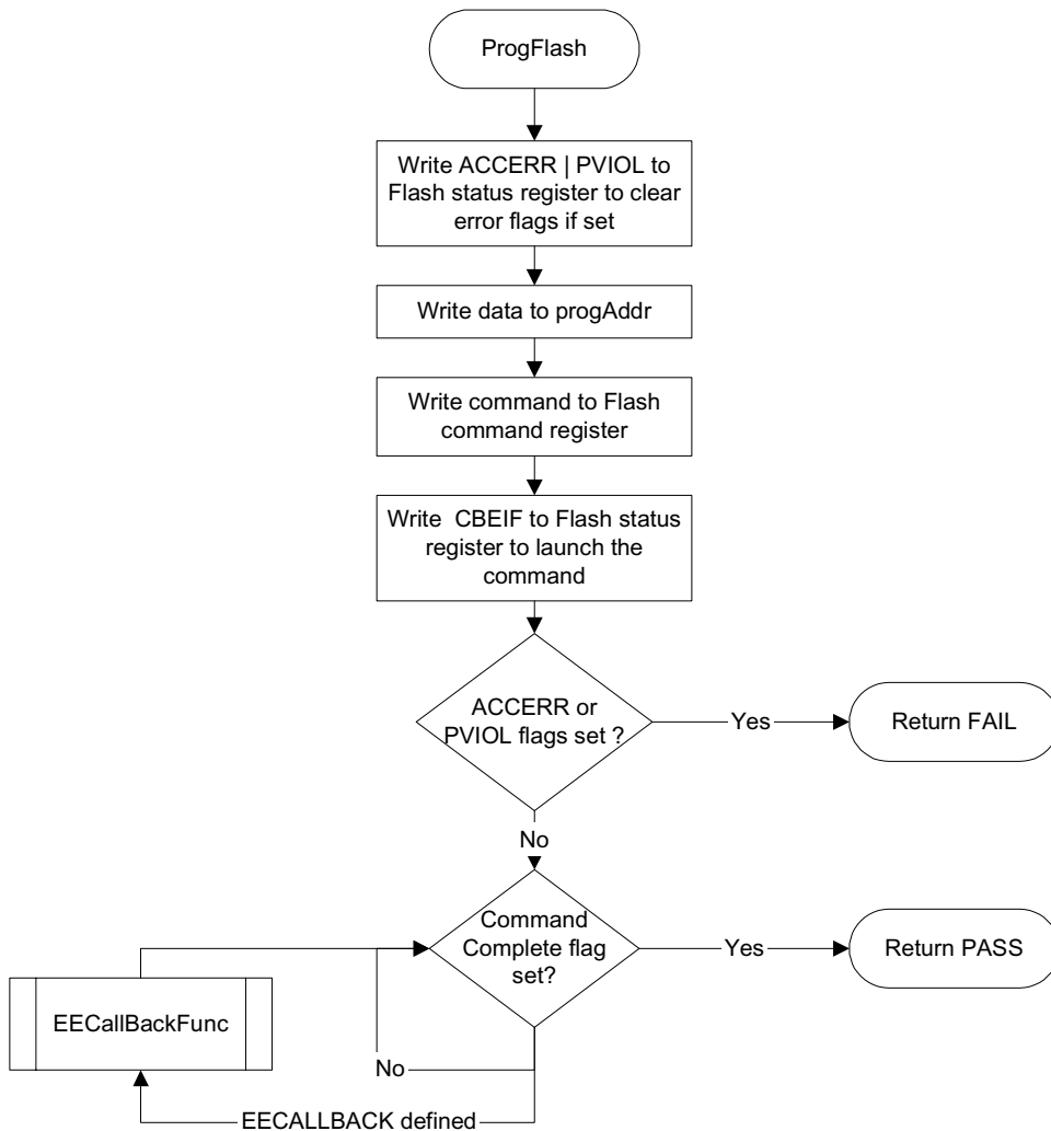
Figure 13. ProgFlash Flow Diagram
