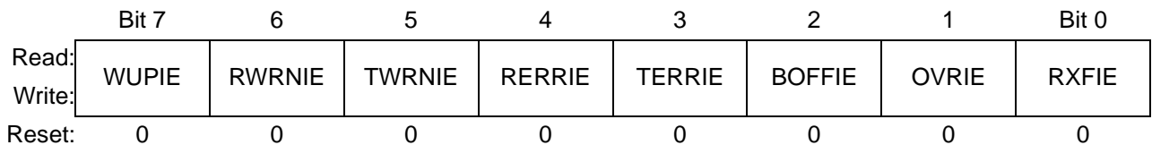
Figure 9. Rev 0.11 Receiver Interrupt Enable Register (CRIER)
