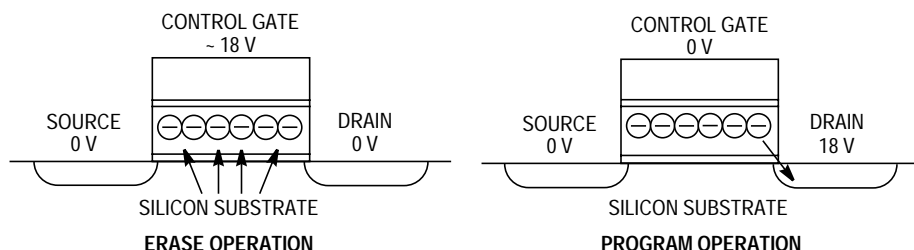
Figure 11. Fowler-Nordheim Tunneling in an EEPROM Bitcell
