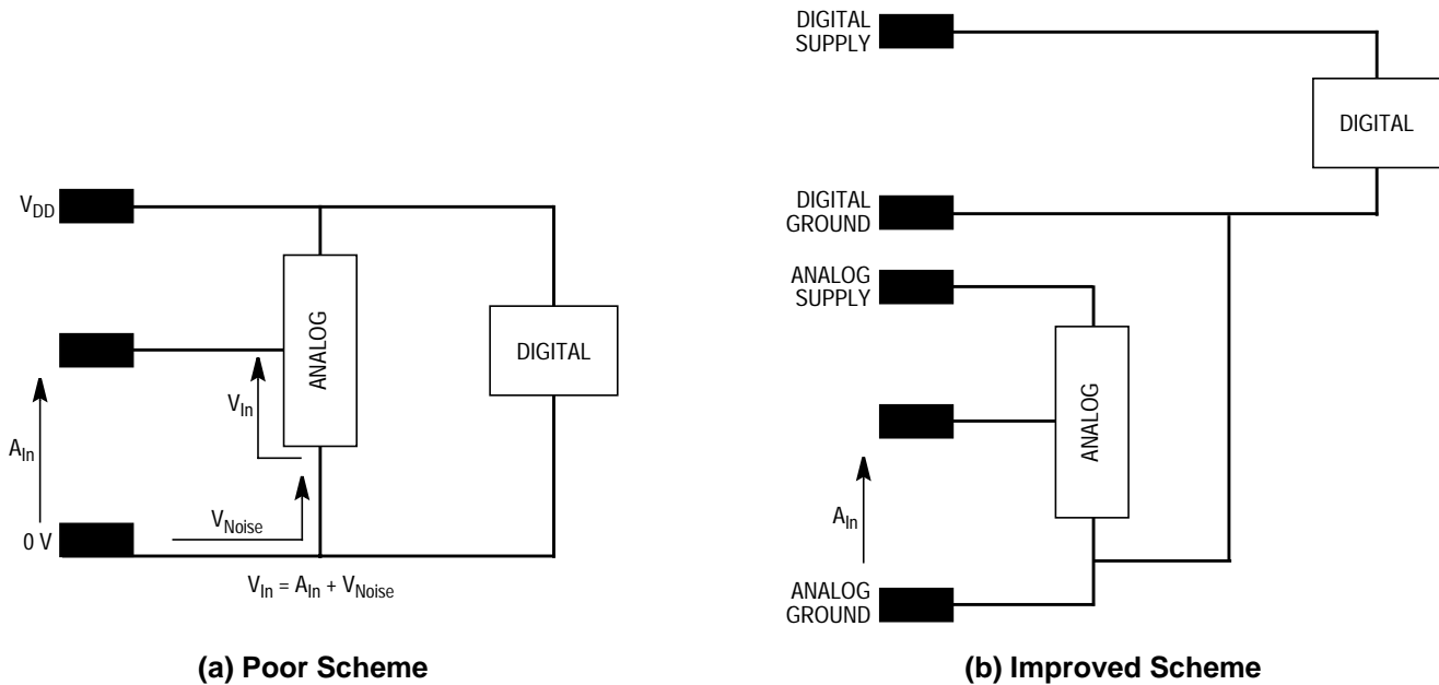
Figure 5. Analog Circuit Grounding
