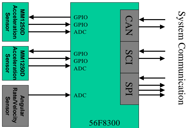
Figure 2-9. Intelligent Inertial Sensor with Three Variables
