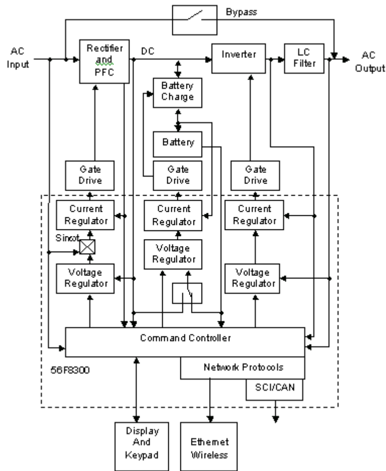
Figure 2-2. UPS Functional Block Diagram
