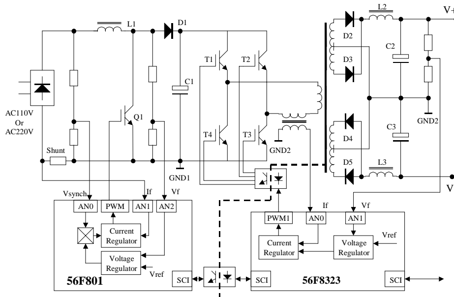
Figure 2-3. Example Digital SMPS
