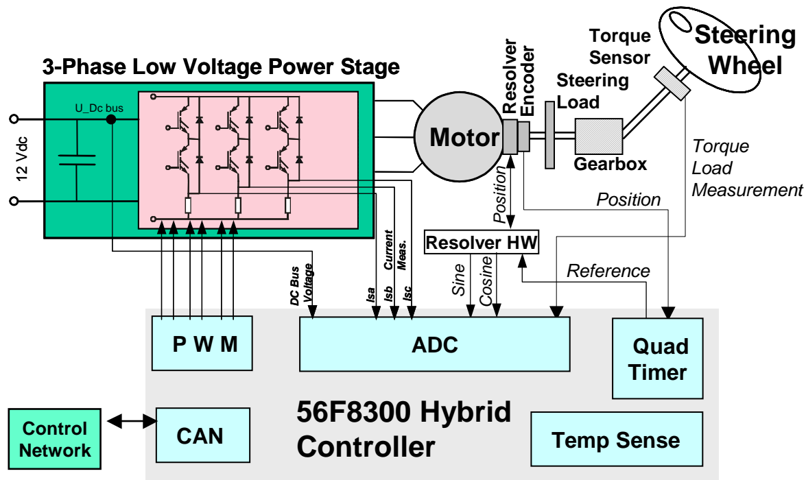
Figure 2-4. Digital Electric Power-Assisted Steering
