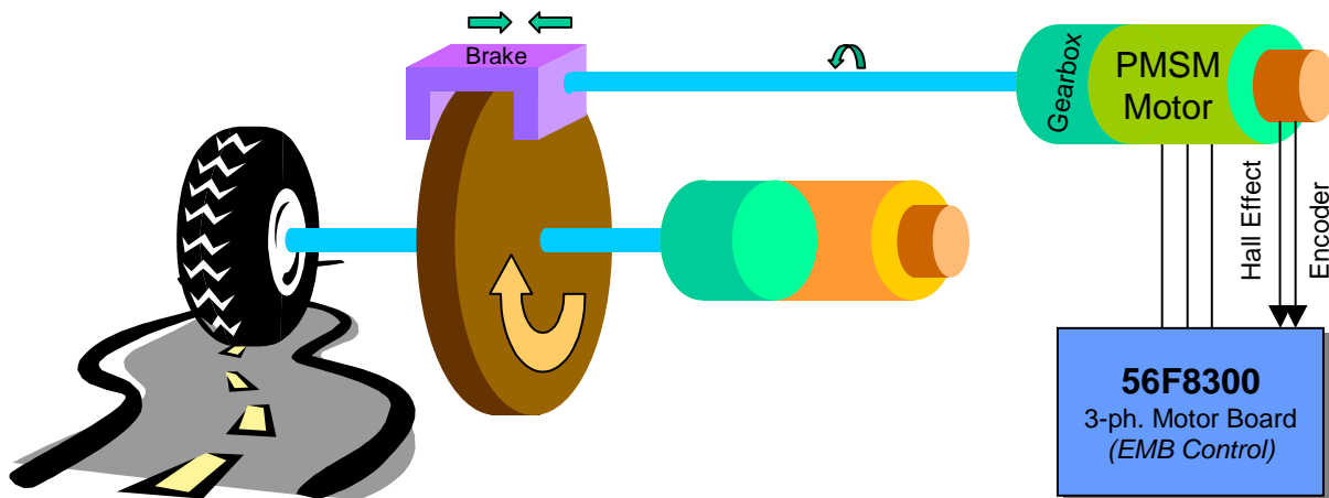
Figure 2-7. EMB Unit detail
