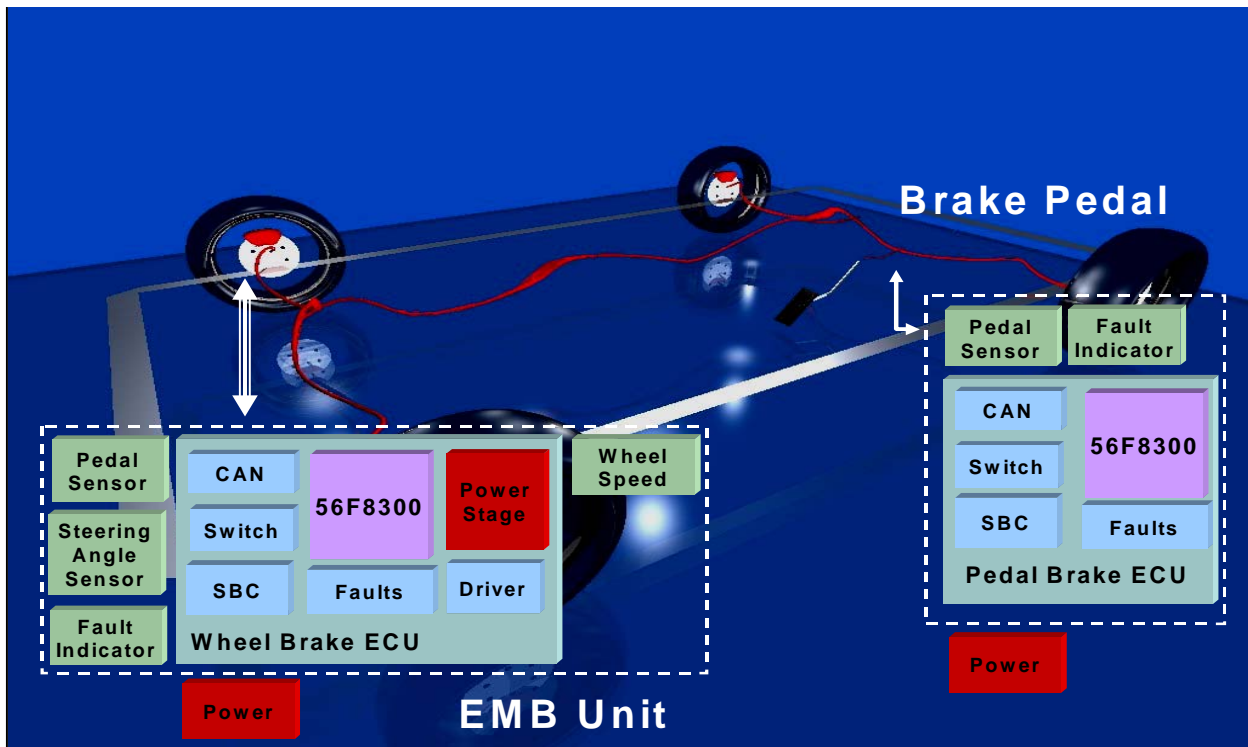
Figure 2-6. EMB System
