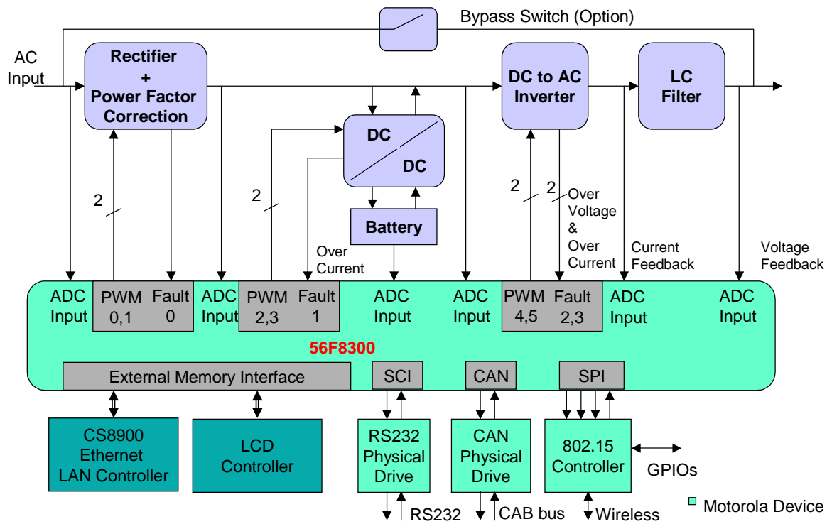
Figure 2-1. Network-enabled UPS Hardware Diagram
