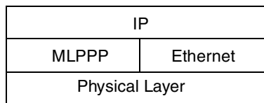
Figure 6. Release 5 Iub Transport Protocol Stack
