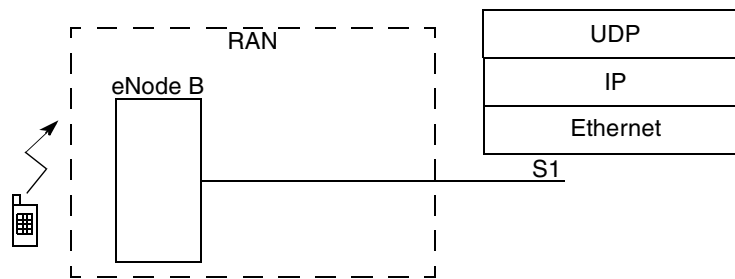
Figure 13. LTE RAN Architecture
