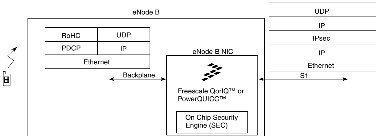
Figure 14. LTE eNode B Transport Solution
