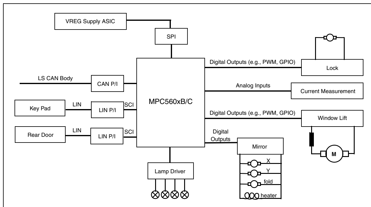
Figure 3. Door controller application example
