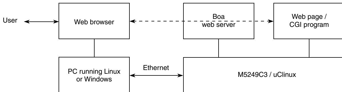
Figure 1. System Setup
