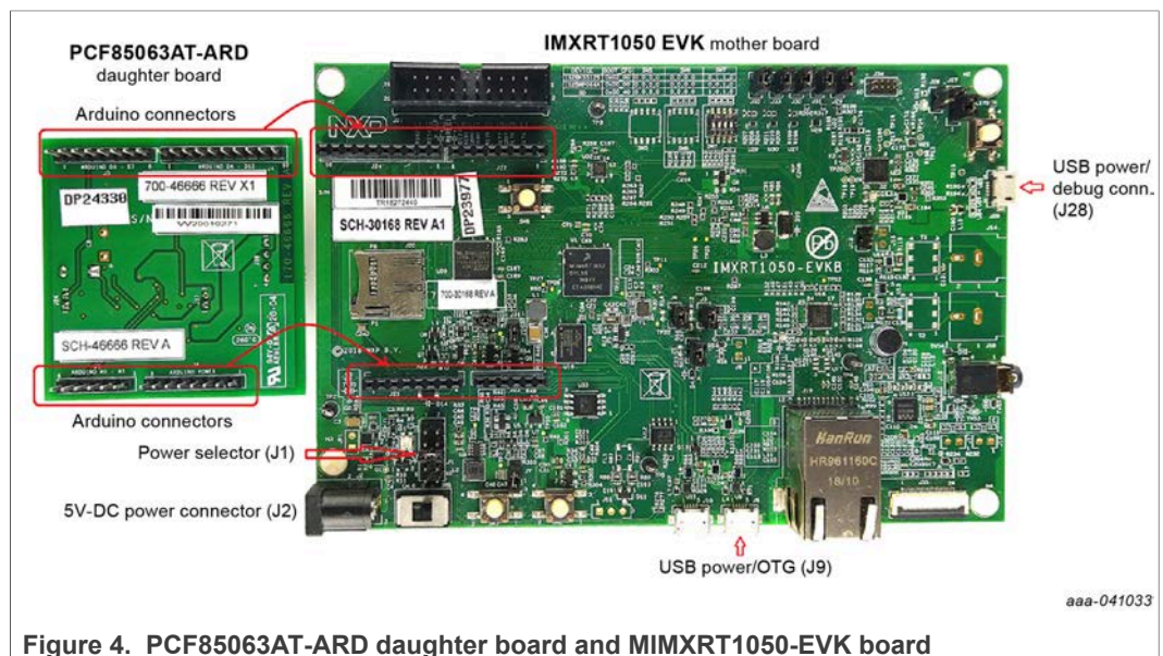
Figure 4. PCF85063AT-ARD daughter board and MIMXRT1050-EVK board
