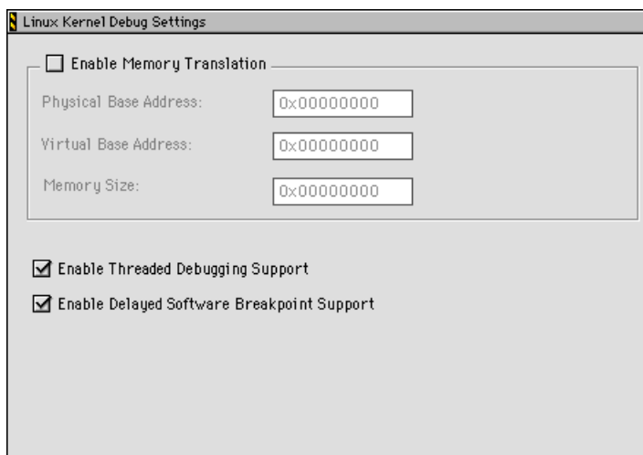
Figure 4.5 Linux Kernel Debug Settings
