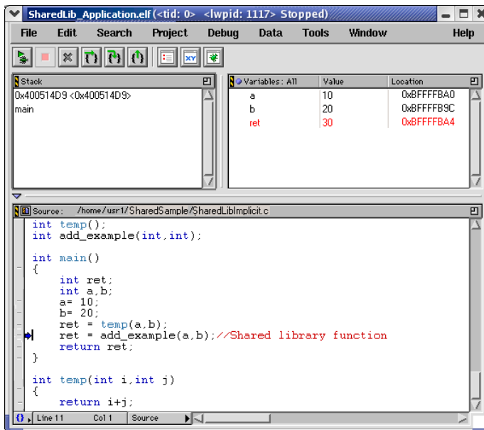
Figure 3.20 Debugger Window
