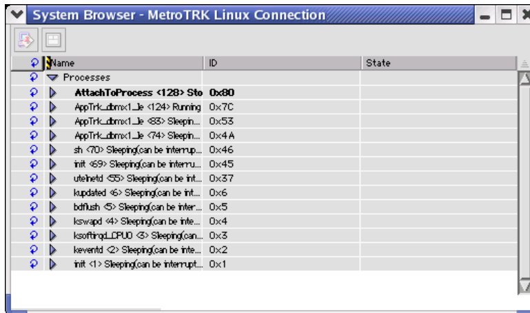
Figure 3.45 Processes Window
