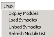
Figure 4.13 Linux Menu
