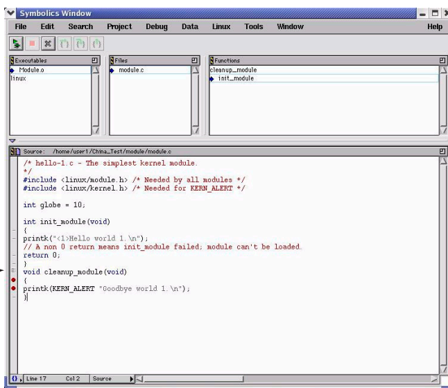
Figure 4.12 Symbolics Window - Symbolics for the Loaded Kernel Module
