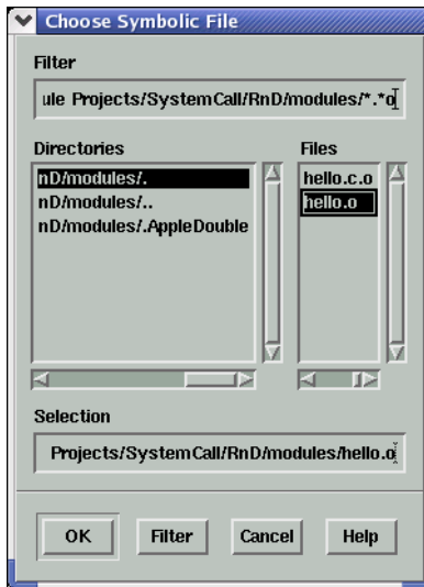
Figure 4.11 Choose File Dialog Box
