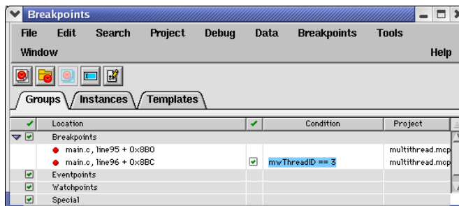
Figure 3.27 Breakpoints Window
