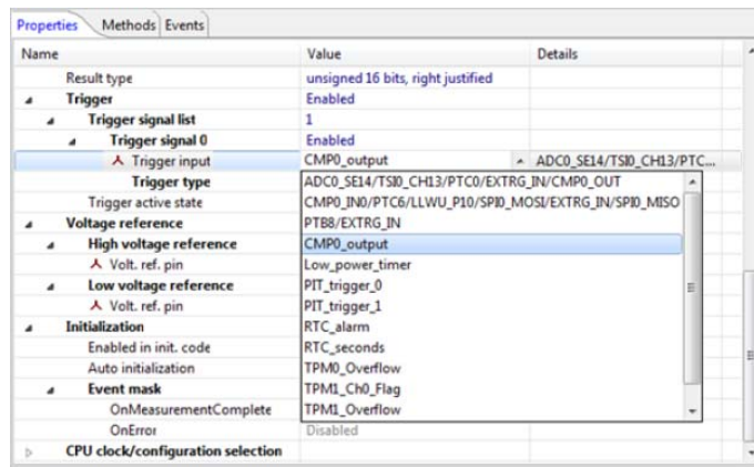
Figure 3.32 A/D converter trigger selection in ADC_LDD
