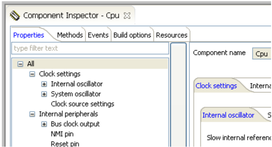
Figure 2.10 Tabs View
