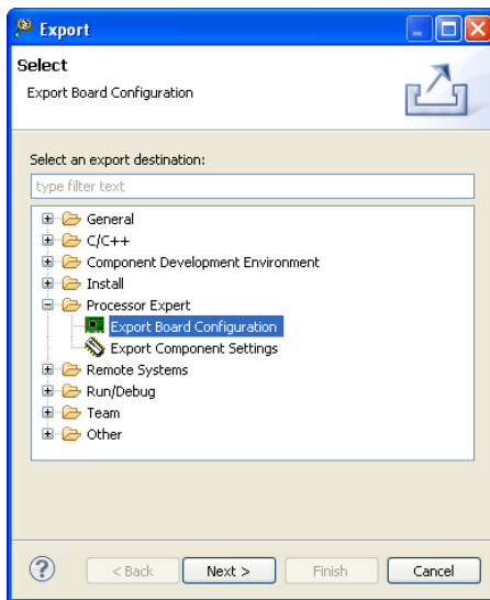
Figure 3.20 Export Wizard
