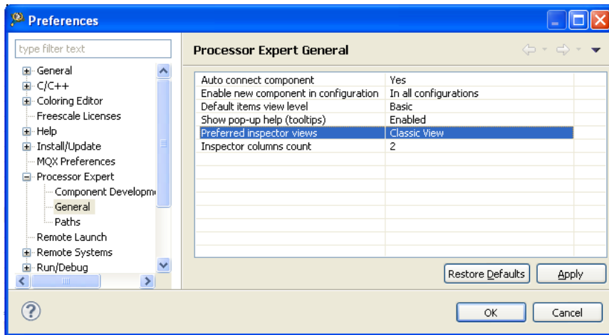
Figure 2.2 Preferences Dialog
