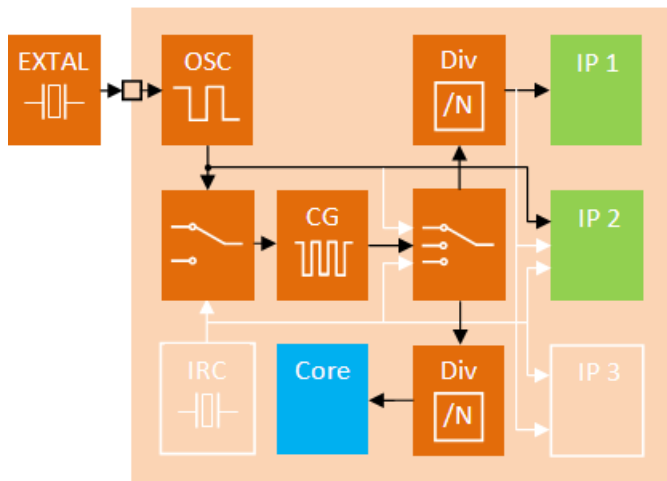
Figure 3.7 Clock configuration example in application run state
