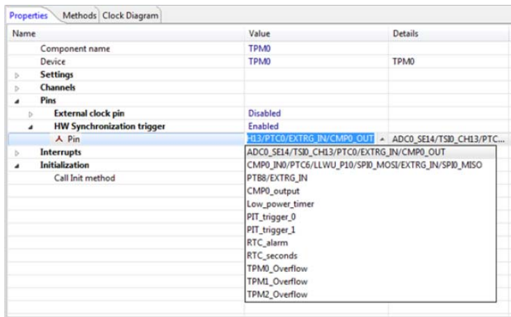
Figure 3.33 Timer synchronization trigger selection in Init_TPM
