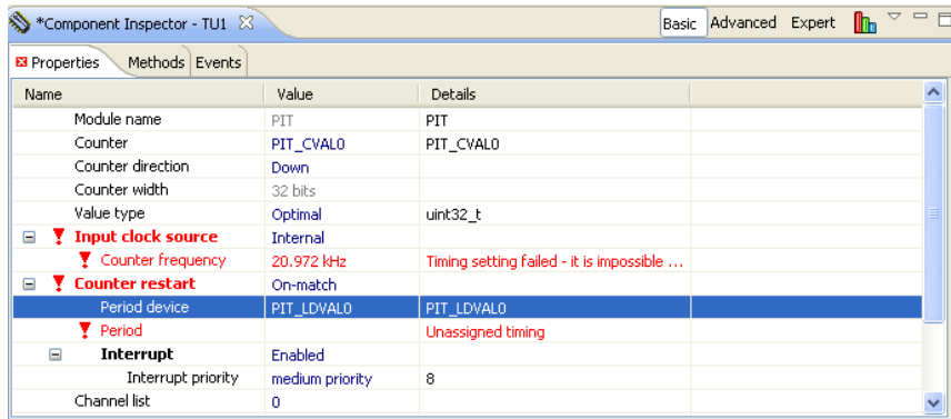
Figure 4.3 Component Inspector — Enabled Interrupt
