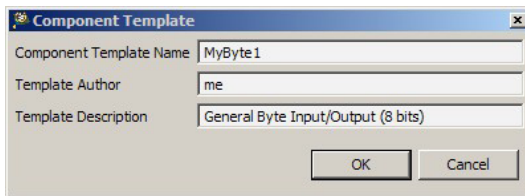
Figure 3.11 Component Template
