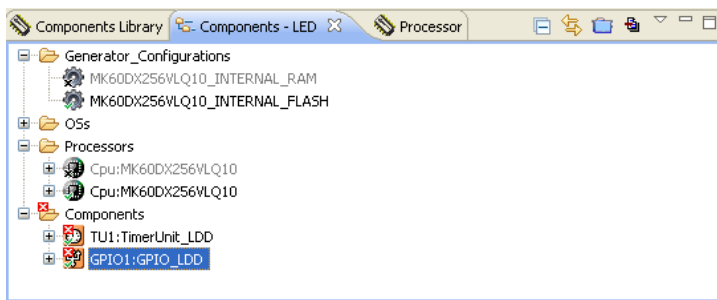
Figure 4.1 Component View
