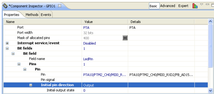
Figure 4.2 Component Inspector
