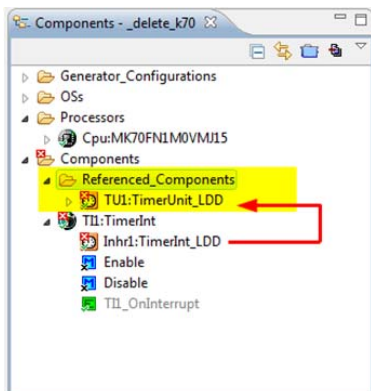
Figure 2.5 Referenced Components
