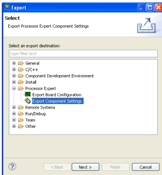
Figure 3.18 Export Wizard
