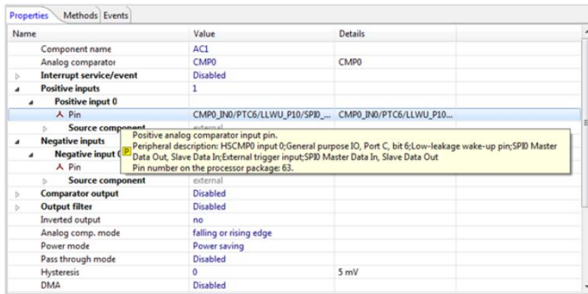
Figure 3.35 Pin selection
