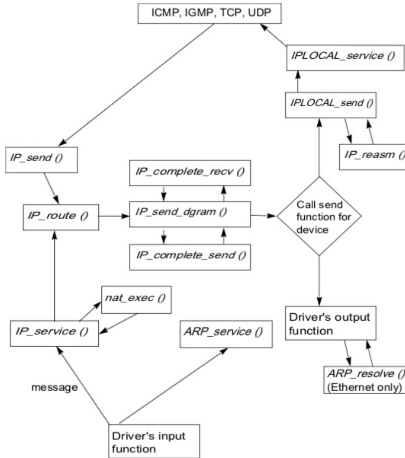
Figure 5-1. Typical RTCS packet-processing paths
