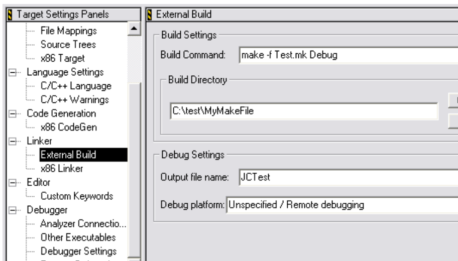
Figure 17.4 External Build Target panel
