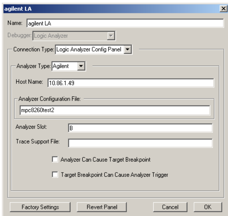
Figure 22.13 Editing a logic analyzer connection
