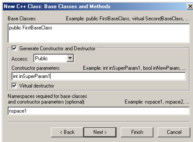
Figure 16.2 New Class wizard—Base Class and Methods
