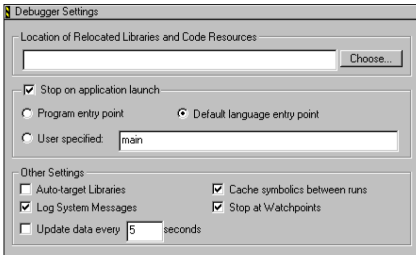
Figure 27.10 Debugger Settings panel
