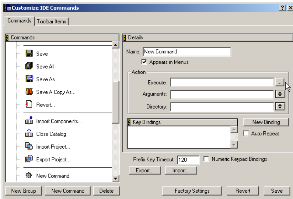
Figure 25.2 Command action fields
