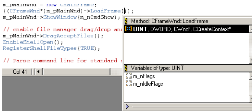
Figure 10.4 Code Completion for Parameter Lists
