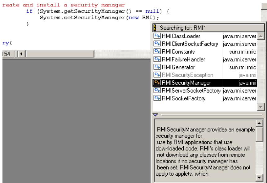
Figure 10.3 Code Completion List of Data Types
