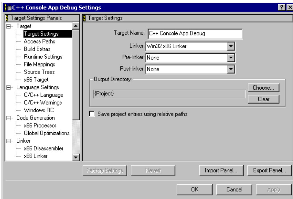
Figure 27.1 Target Settings window
