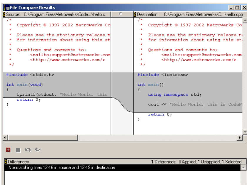
Figure 12.10 File Compare Results window
