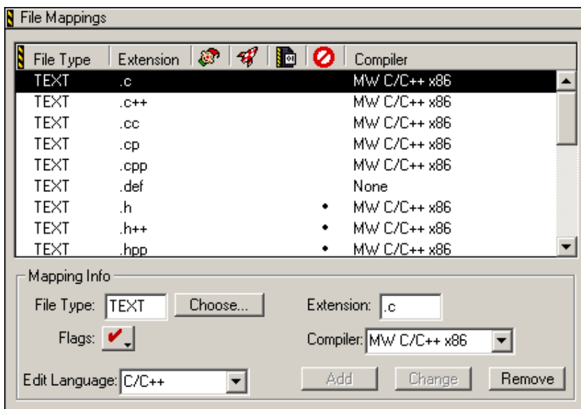
Figure 27.6 File Mappings settings panel
