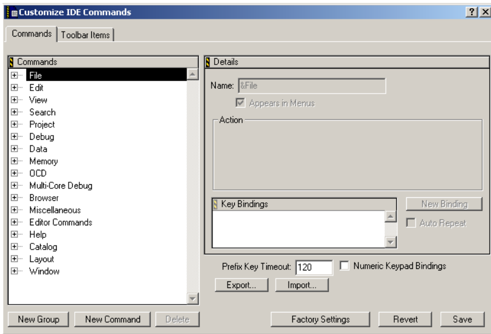
Figure 25.1 Customize IDE Commands window
