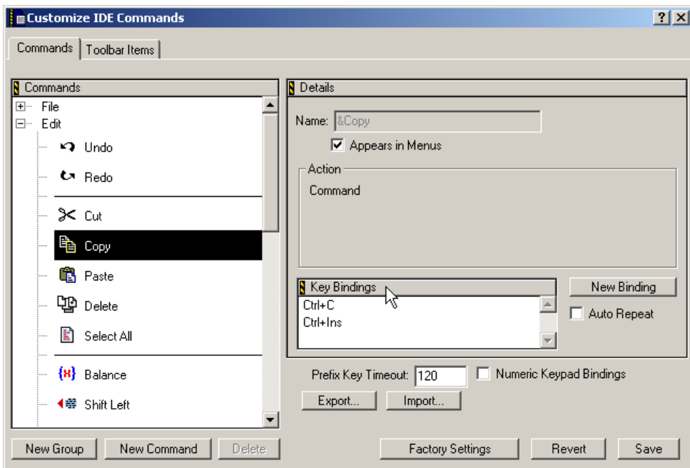
Figure 25.8 Customize IDE Commands—Key Bindings
