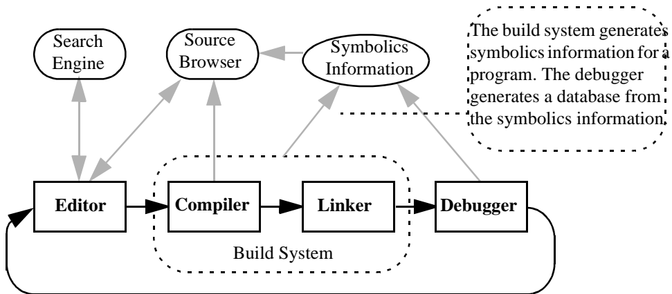
Figure 3.1 Project Manager
