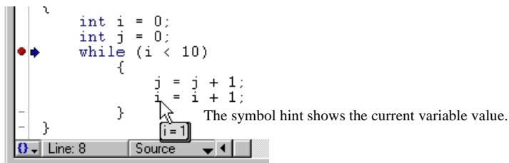
Figure 17.2 Symbol hint
