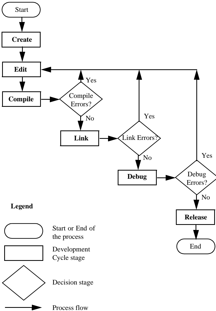
Figure 2.1 The Development Cycle diagram
