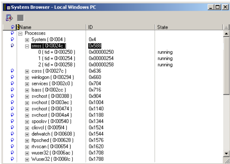
Figure 21.2 System Browser window
