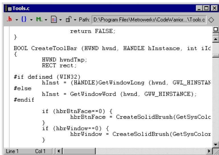
Figure 9.1 Editor window
