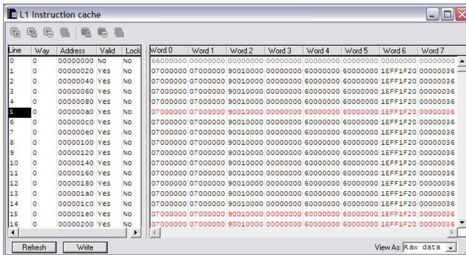
Figure 22.15 Cache window
