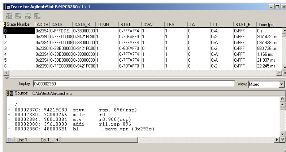
Figure 22.14 Trace window
