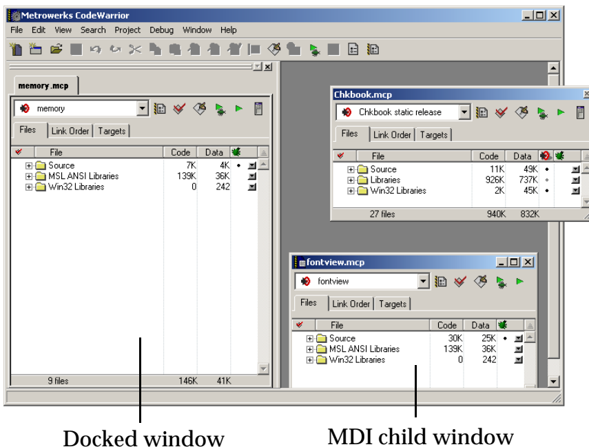
Figure 6.1 Window states
