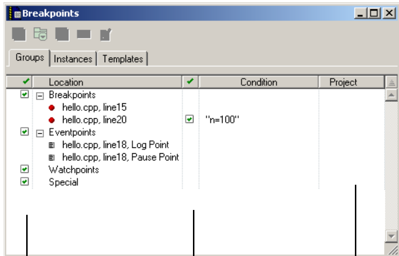
Figure 18.1 Breakpoints window
