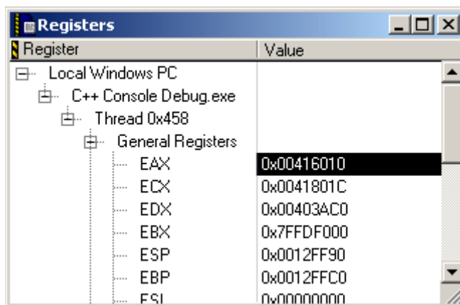
Figure 20.3 Registers Window
