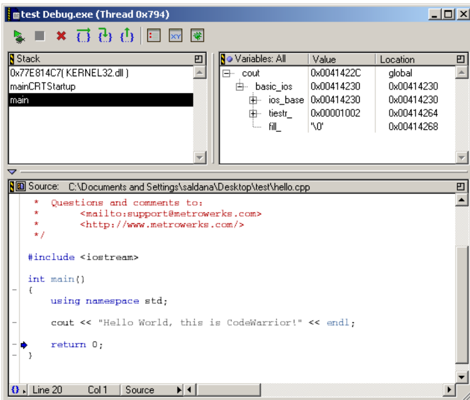
Figure 17.1 Thread window
