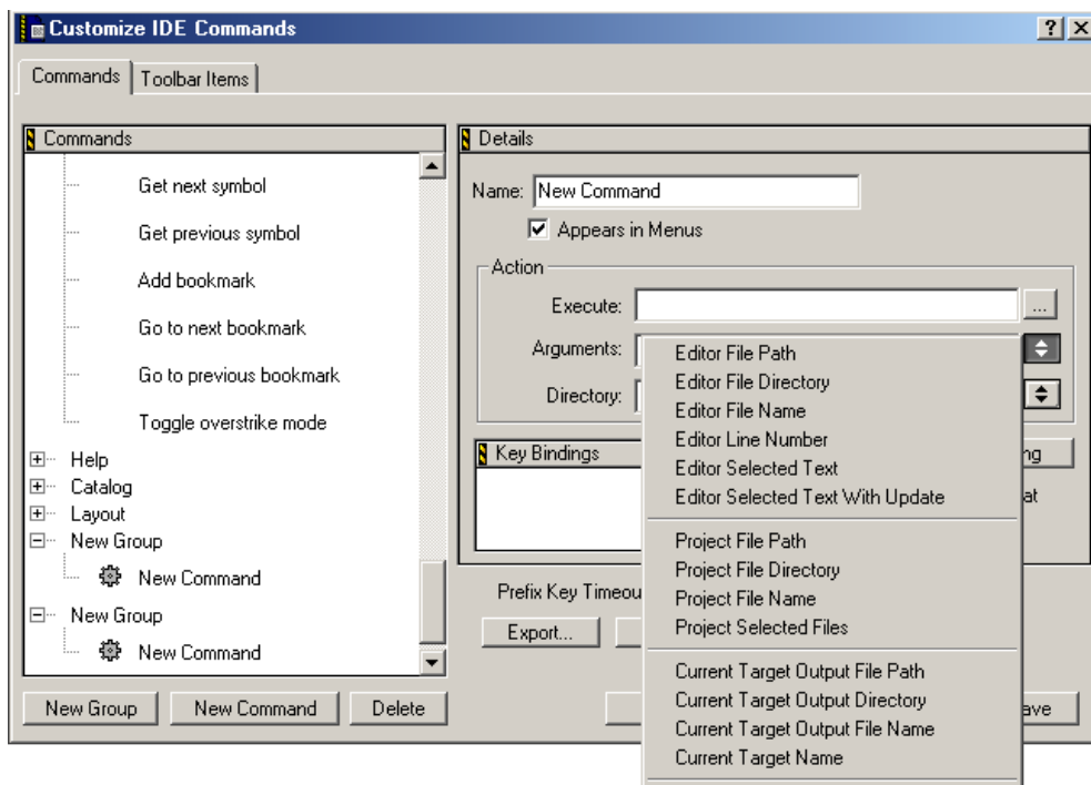
Figure 25.3 Pre-defined Arguments
