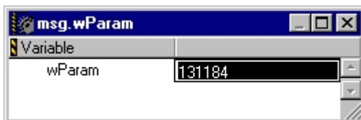
Figure 19.2 Variable window
