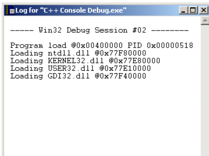
Figure 21.3 Log window
