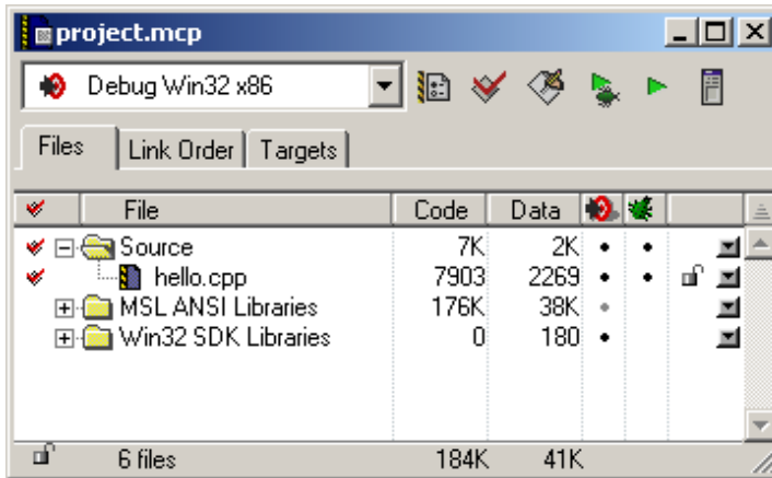
Figure 4.1 Project window
