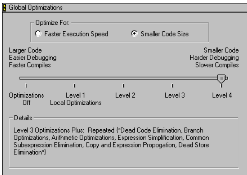
Figure 27.7 Global Optimizations settings panel
