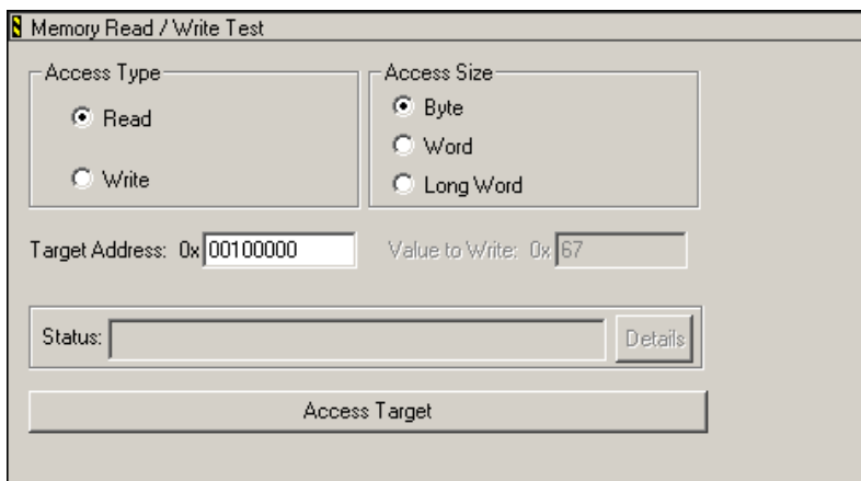
Figure 22.9 Memory Read / Write panel
