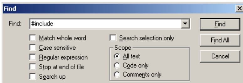
Figure 12.1 Find window
