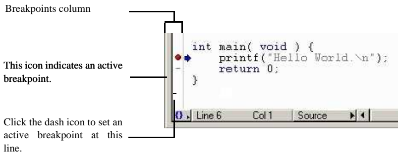
Figure 18.2 Setting Breakpoints
