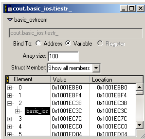
Figure 20.2 Array window
