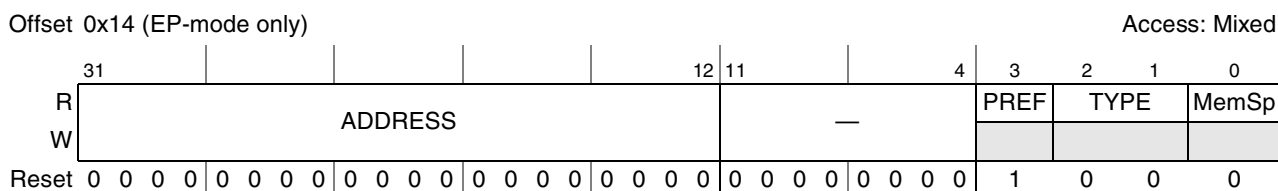
Figure 18-48. 32-Bit Memory Base Address Register (BAR1)
