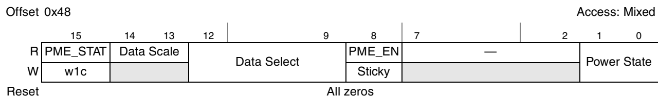
Figure 18-81. PCI Express Power Management Status and Control Register
