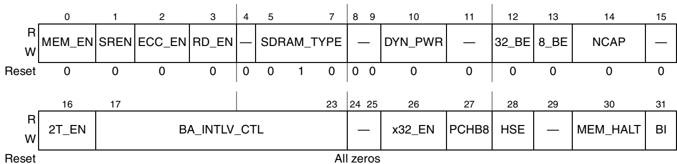
Figure 9-8. DDR SDRAM Control Configuration Register (DDR_SDRAM_CFG)
