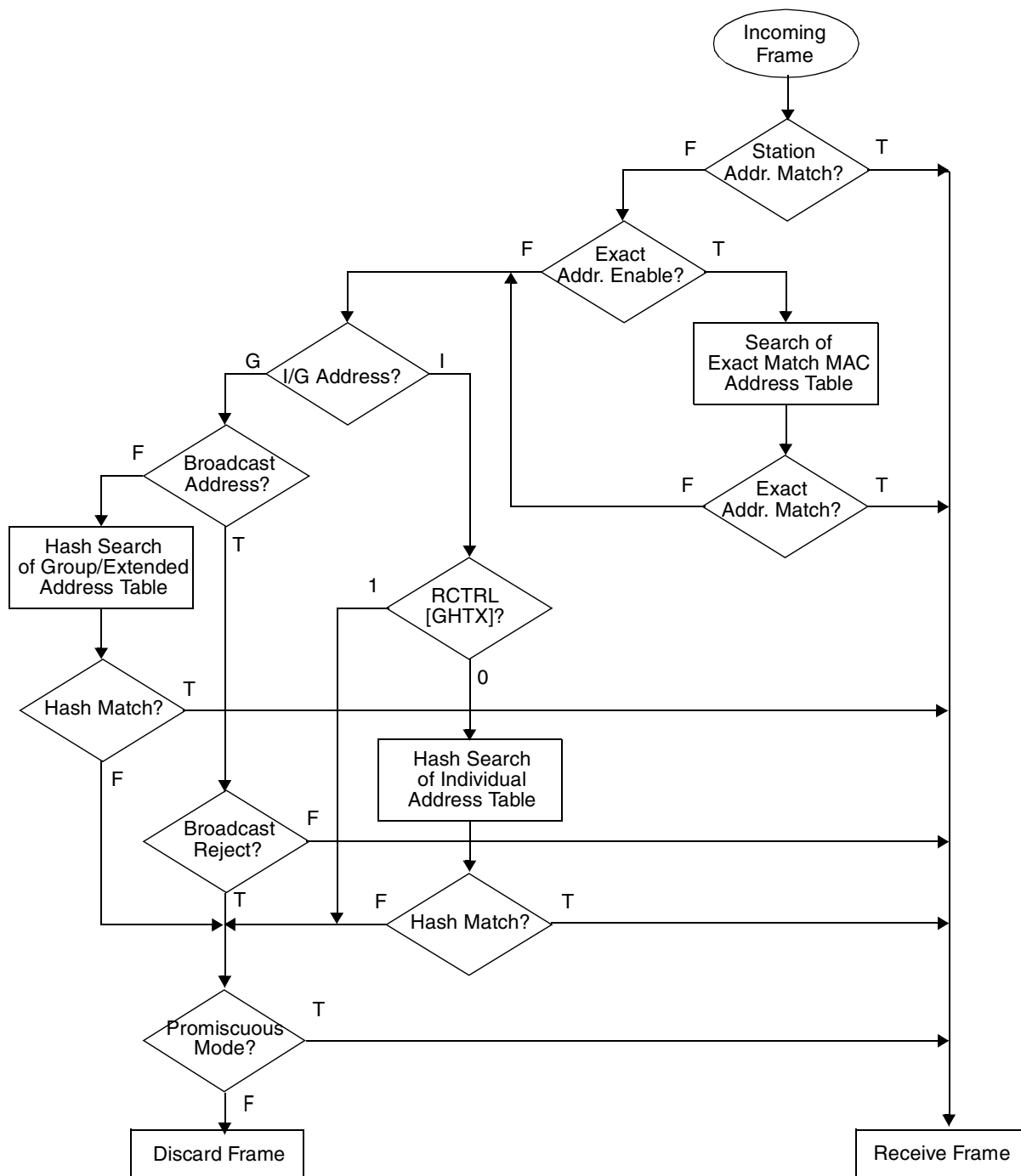
Figure 15-128. Ethernet Address Recognition Flowchart
