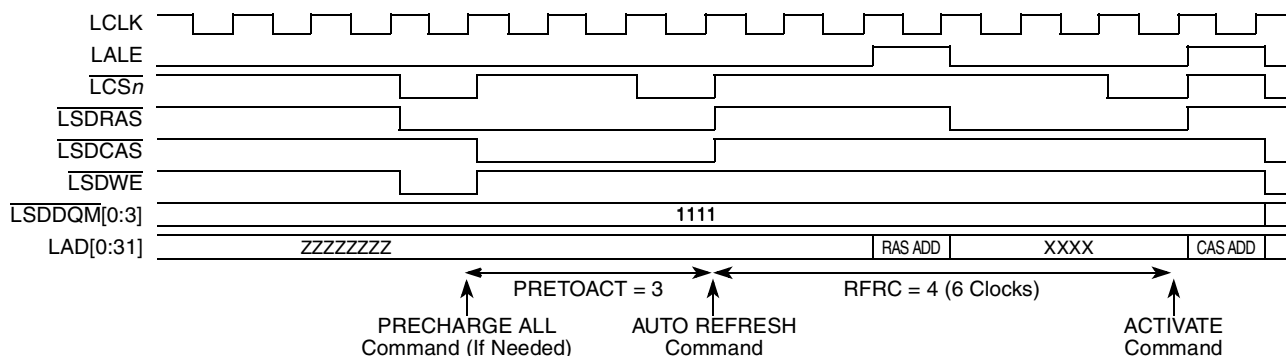
Figure 14-40. RFRC = 4 (6 Clock Cycles)
