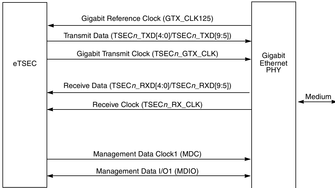
Figure 15-122. eTSEC-RTBI Connection
