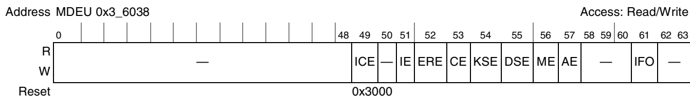
Figure 12-36. MDEU Interrupt Control Register
