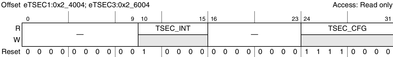
Figure 15-3. TSEC_ID2 Register
