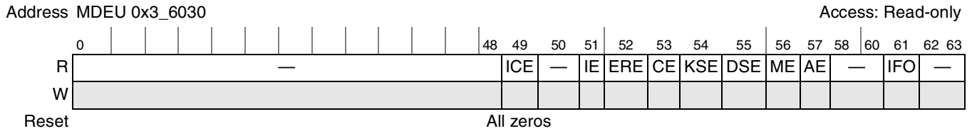
Figure 12-35. MDEU Interrupt Status Register
