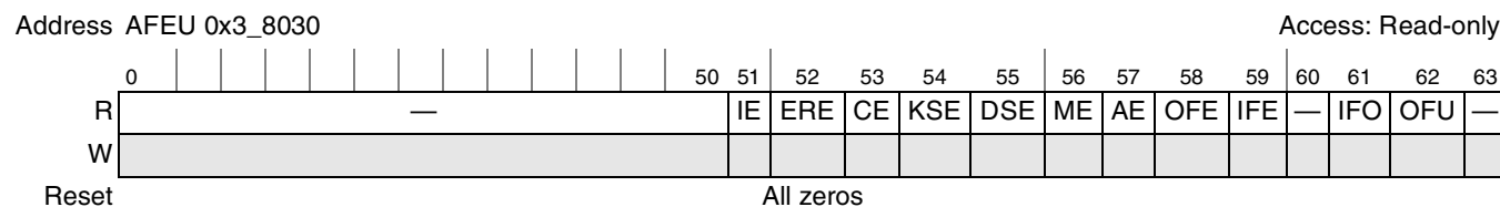
Figure 12-26. AFEU Interrupt Status Register
