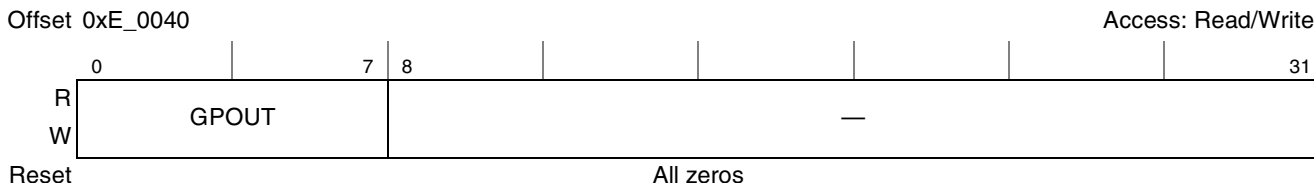
Figure 19-9. General-Purpose Output Data Register (GPOUTDR)
