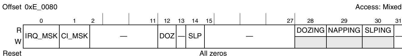
Figure 19-13. Power Management Control and Status Register (POWMGTCSR)
