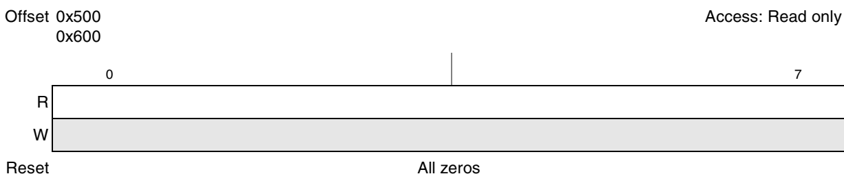
Figure 13-2. Receiver Buffer Registers (URBR0, URBR1)
