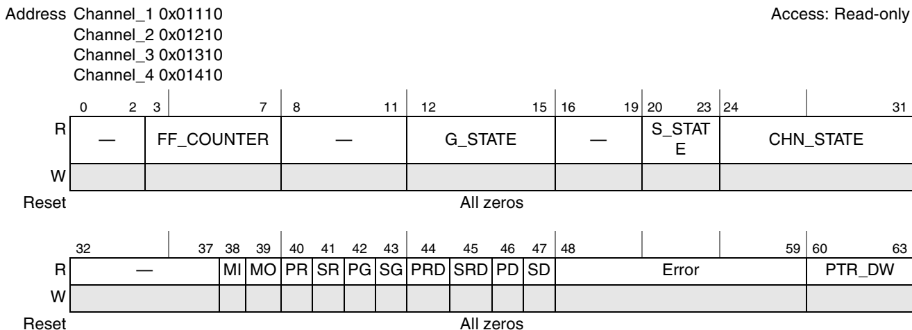
Figure 12-74. Crypto-Channel Pointer Status Register
