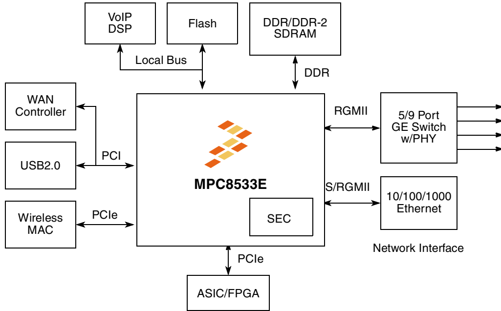
Figure 1-4. Multifunction Router Application Enabled by local bus, PCI Express, PCI, and Ethernet
