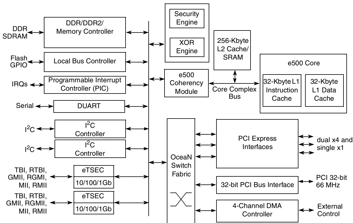
Figure 1-1. MPC8533E Block Diagram
