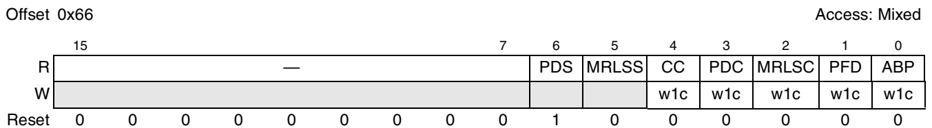
Figure 18-93. PCI Express Slot Status Register
