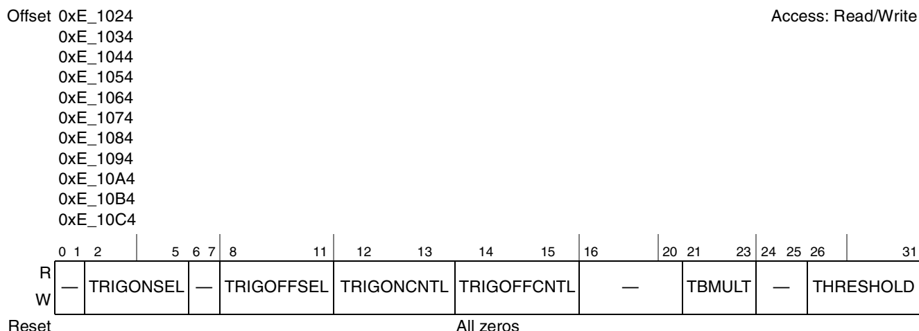
Figure 20-6. Performance Monitor Local Control Register B (PMLCB1–PMLCB9)
