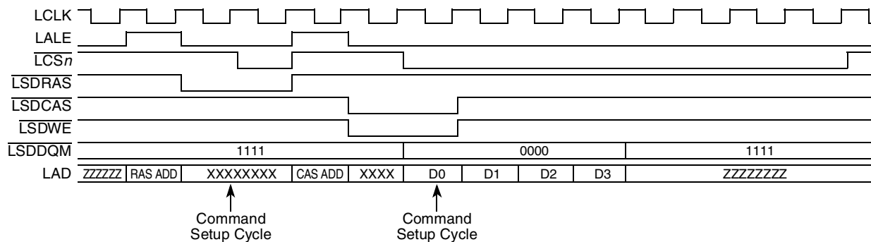
Figure 14-41. BUFCMD = 1, LCRR[BUFCMDC] = 2
