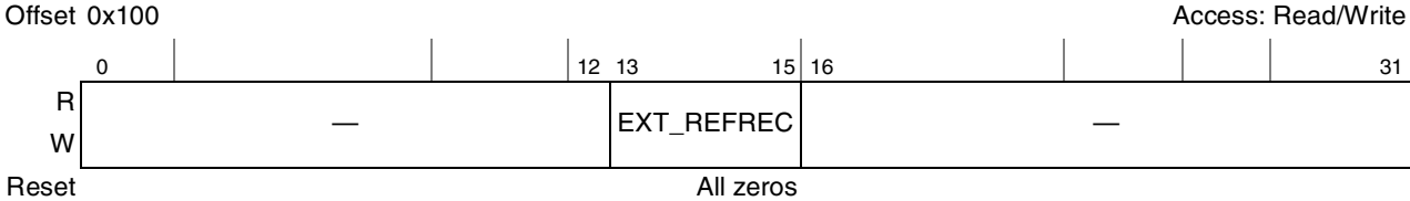
Figure 9-4. DDR SDRAM Timing Configuration 3 (TIMING_CFG_3)
