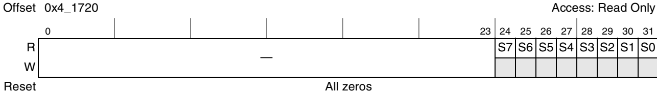
Figure 10-32. Shared Message Signaled Interrupt Status Register (MSISR)
