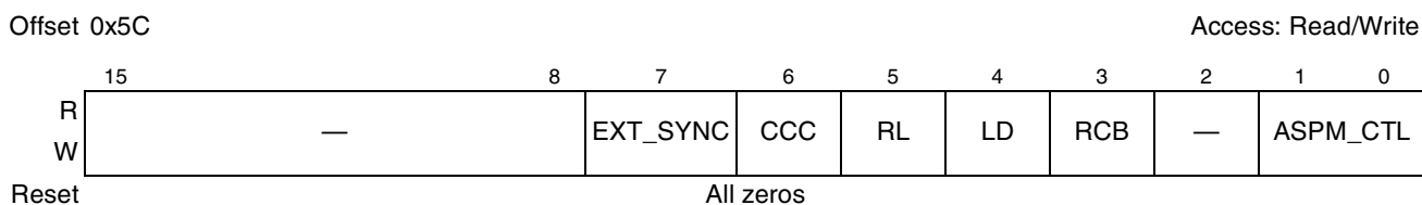
Figure 18-89. PCI Express Link Control Register
