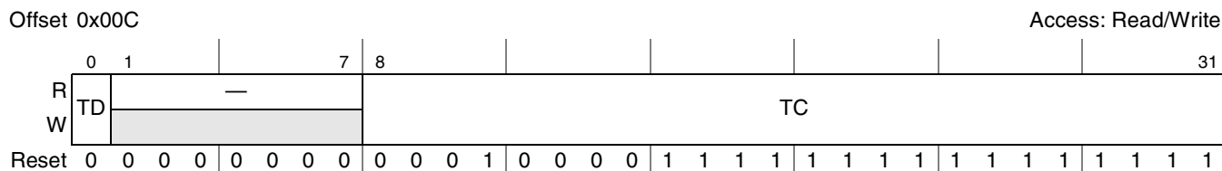
Figure 18-4. PCI Express Outbound Completion Timeout Register (PEX_OTB_CPL_TOR)
