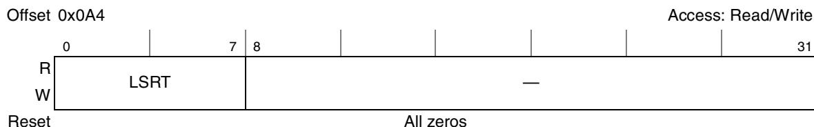
Figure 14-12. LSRT SDRAM Refresh Timer (LSRT)
