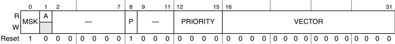
Figure 10-38. Internal Interrupt Vector/Priority Registers (IIVPRs)
