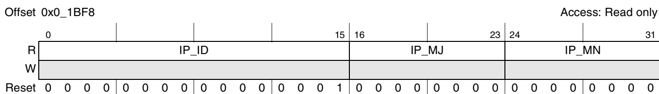
Figure 8-4. ECM IP Block Revision Register 1 (EIPBRR1)
