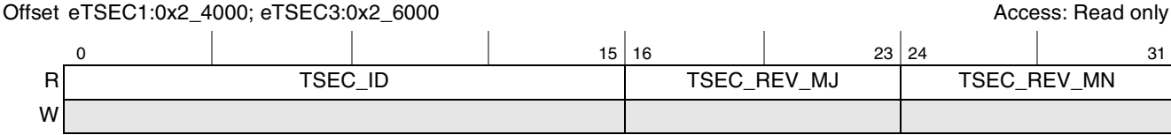
Figure 15-2. TSEC_ID Register
