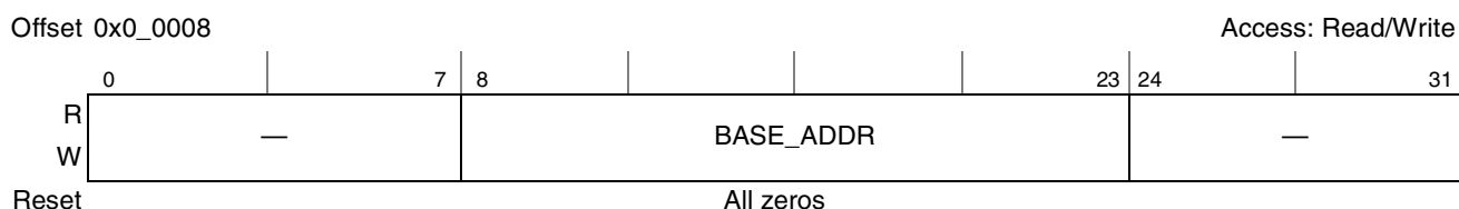
Figure 4-2. Alternate Configuration Base Address Register (ALTFCBAR)
