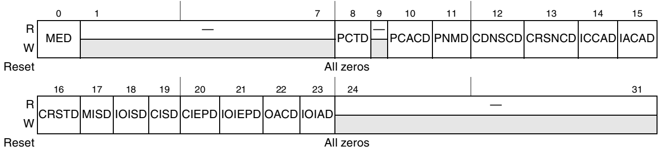
Figure 18-26. PCI Express Error Disable Register (PEX_ERR_DISR)
