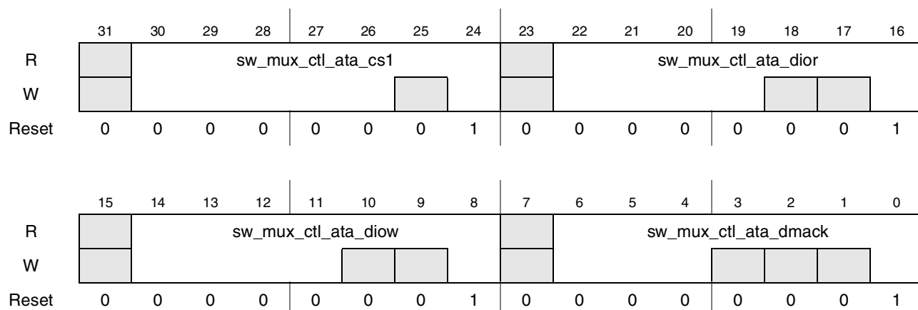
Figure 4-8. Register Description sw_mux_ctl_ata_cs1_ata_dior_ata_diow_ata_dmack
