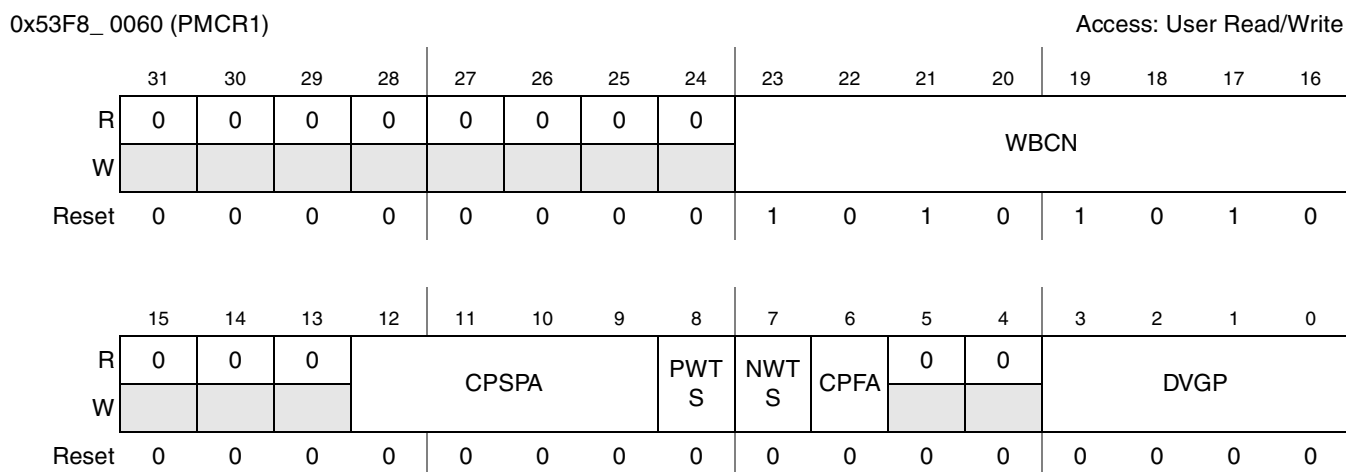
Figure 3-22. Power Management Control Register 1 (PMCR1)
