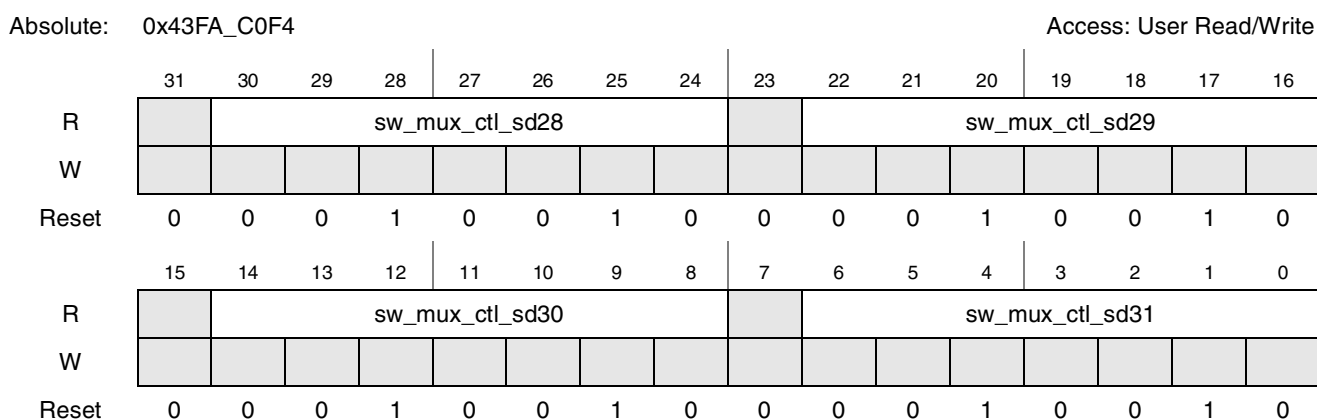
Figure 4-64. Register Description sw_mux_ctl_sd28_sd29_sd30_sd31
