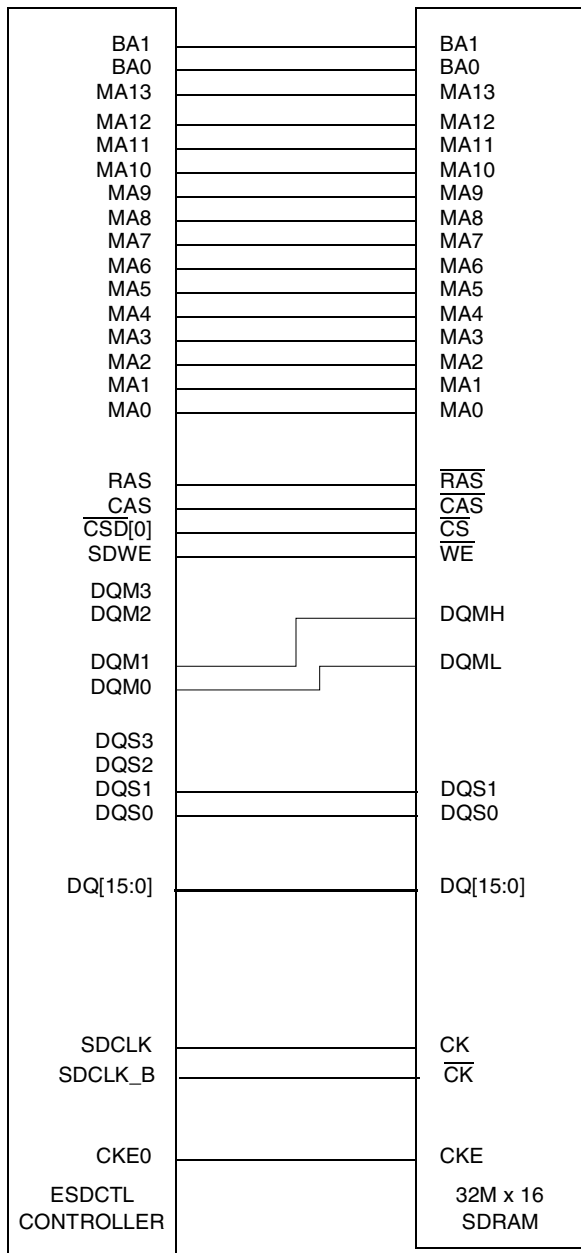
Figure 19-98. Single 512-Mbit (32Mx16) LPDDR SDRAM Connection Diagram
