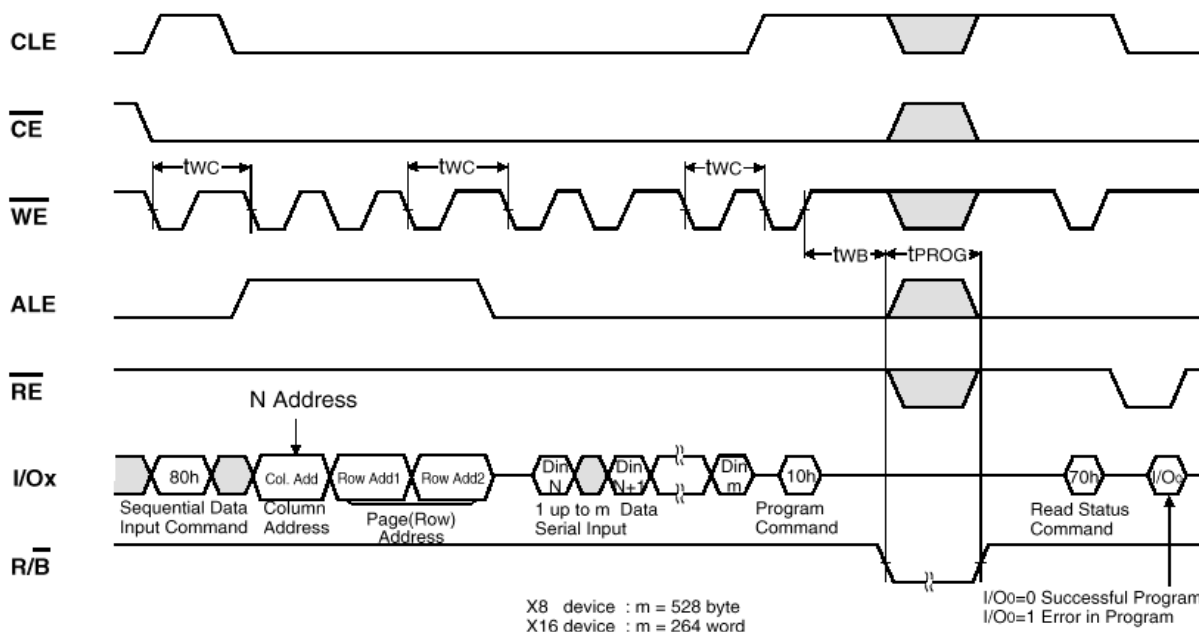
Figure 20-22. Program Operation
