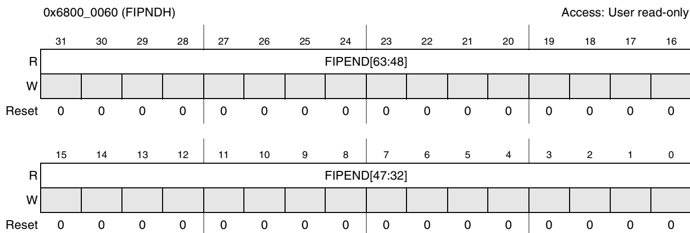
Figure 9-27. FIPNDH Register
