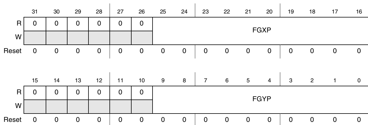
Figure 44-55. SDC Foreground Window Position Register (SDC_FG_POS)
