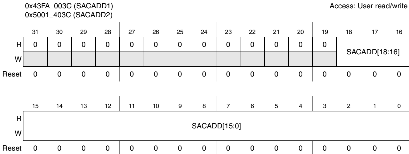
Figure 45-34. SSI AC97 Command Address Register
