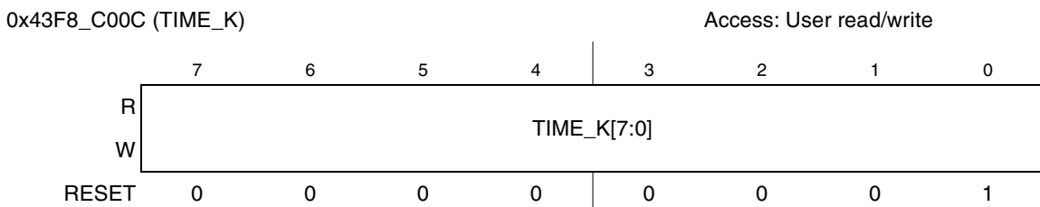
Figure 23-25. TIME_K Register
