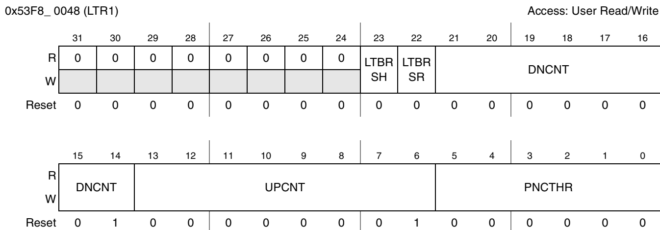
Figure 3-16. Load Tracking Register (LTR1)
