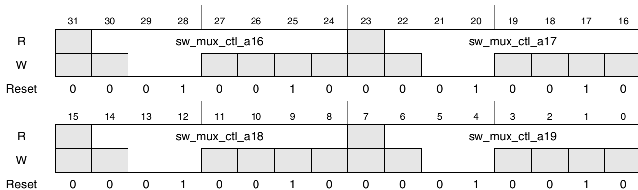
Figure 4-74. Register Description sw_mux_ctl_a16_a17_a18_a19
