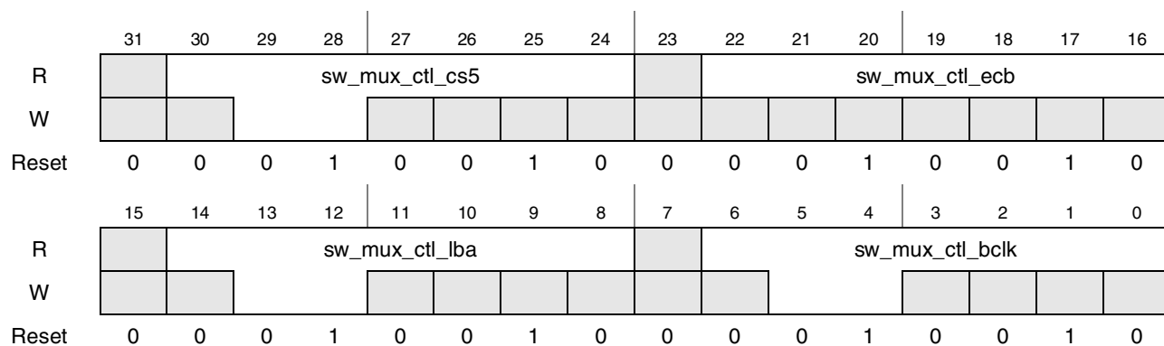
Figure 4-60. Register Description sw_mux_ctl_cs5_ecb_lba_bclk
