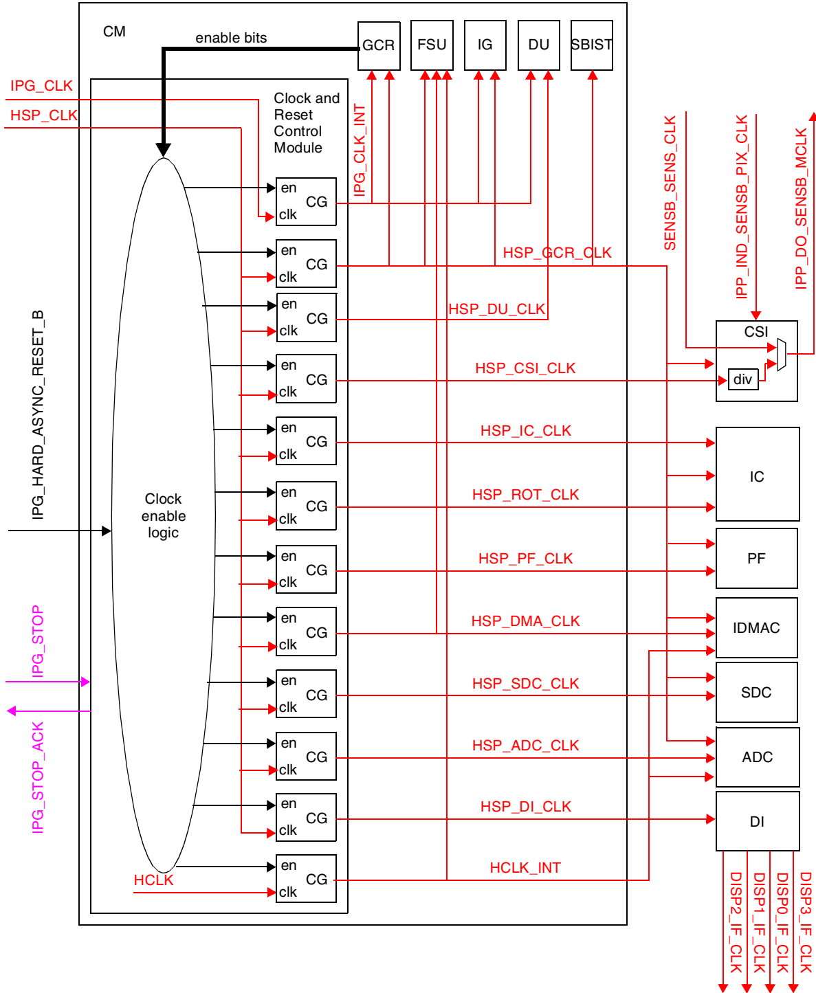
Figure 44-6. Clocking Microarchitecture in the IPU
