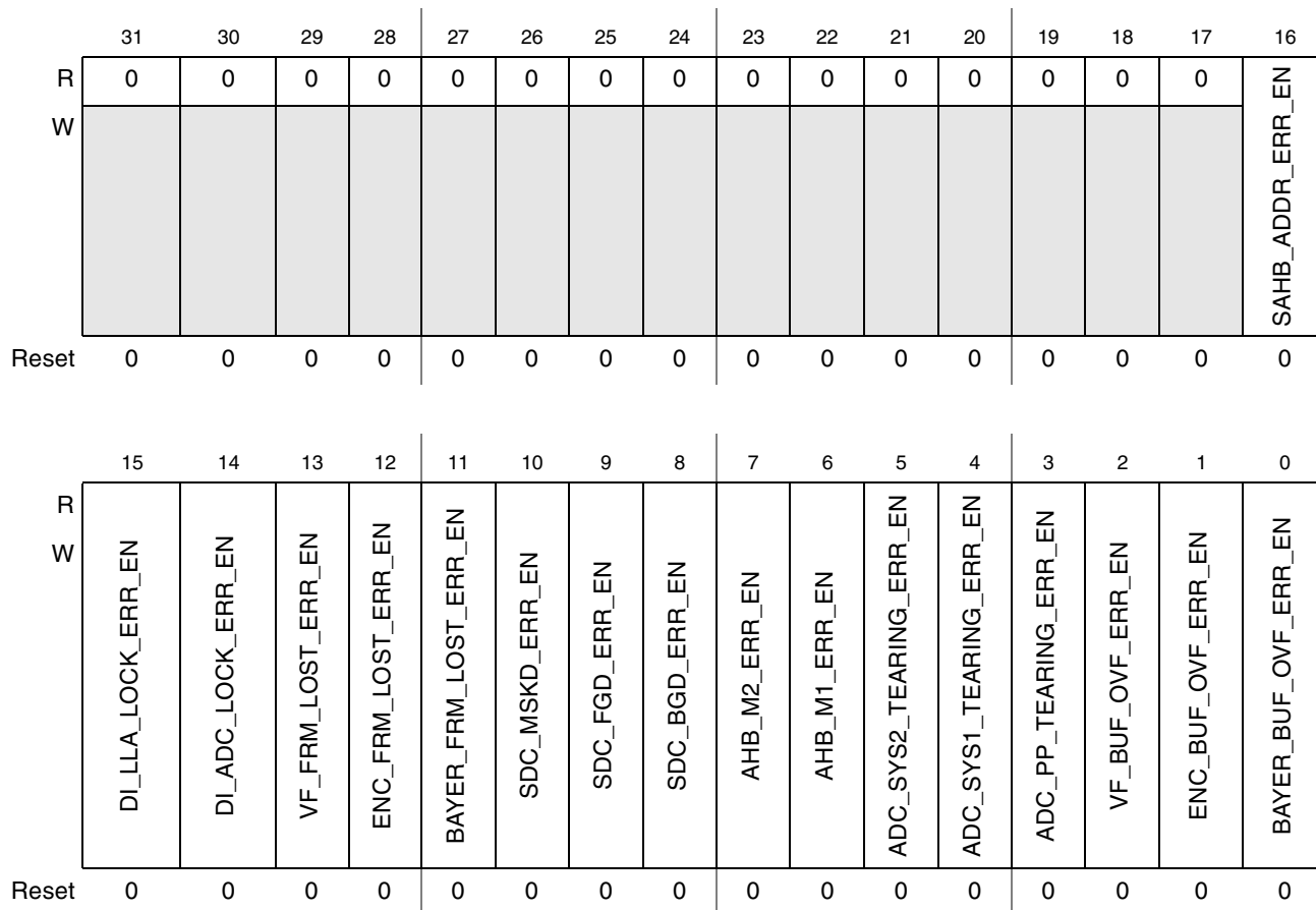
Figure 44-22. IPU Interrupt Control Register 5 (IPU_INT_CTRL_5)
