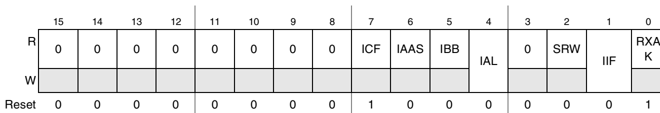
Figure 26-9. I 2 C Status Register
