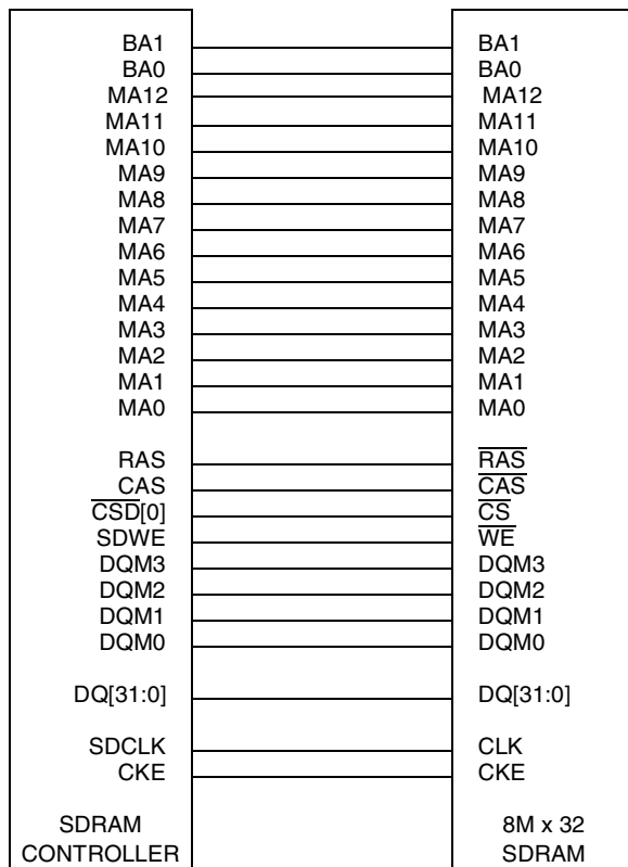
Figure 19-93. Single 256-MB (8Mx32) SDRAM Connection Diagram
