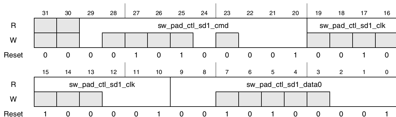
Figure 4-95. Register Description sw_pad_ctl_sd1_cmd_sd1_clk_sd1_data0
