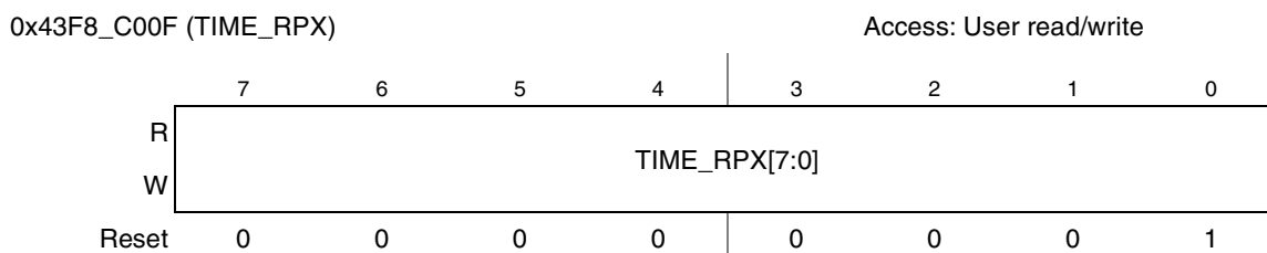
Figure 23-28. TIME_RPX Register
