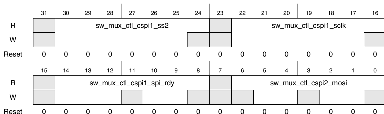
Figure 4-37. Register Description sw_mux_ctl_cspi1_ss2_cspi1_sclk_cspi1_spi_rdy_cspi2_mosi
