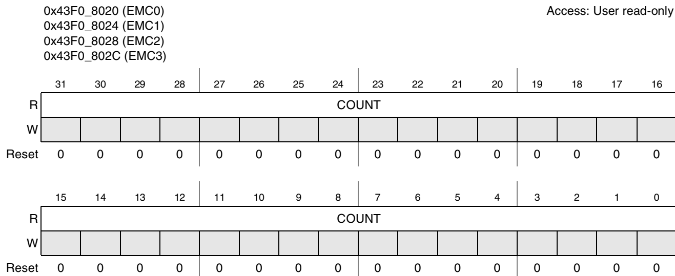
Figure 15-5. EMCx Registers
