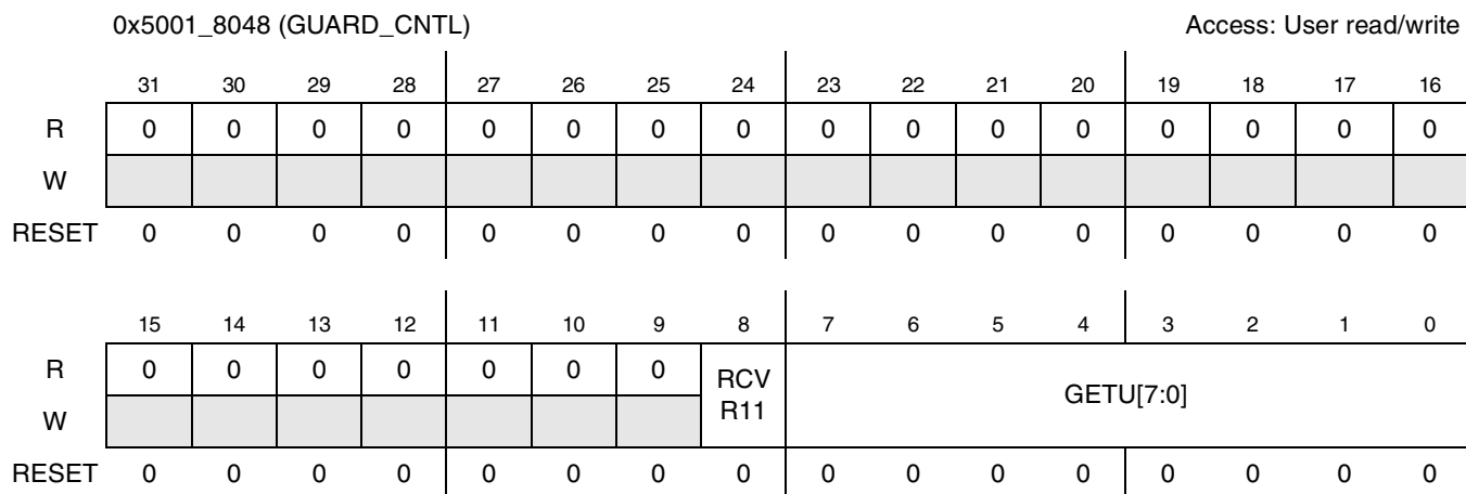
Figure 30-21. SIM Transmit Guard Control Register
