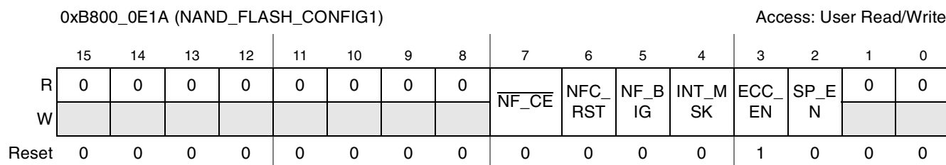
Figure 20-18. NAND_FLASH_CONFIG1 Register
