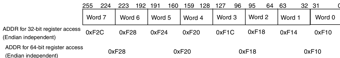
Figure 14-15. Word Order of L2 Cache Lines in Line Data Registers
