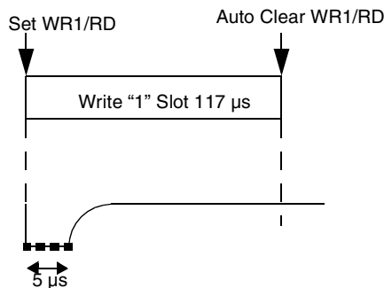
Figure 22-10. Write 1 Timing
