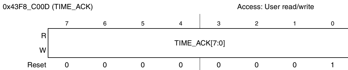
Figure 23-26. TIME_ACK Register
