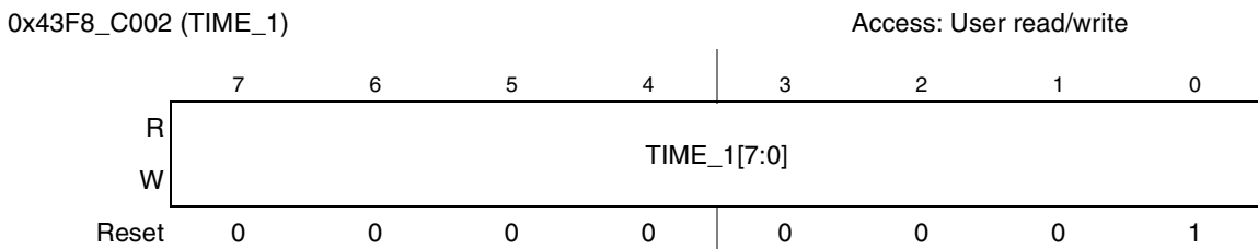
Figure 23-15. TIME_1 Register
