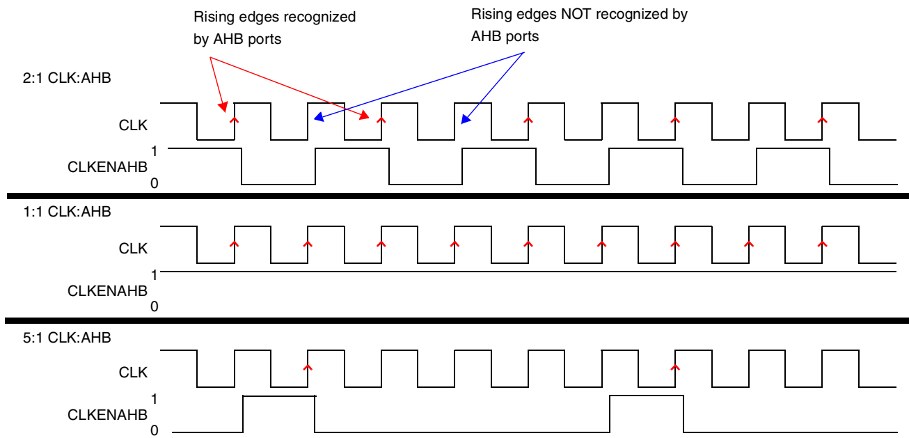
Figure 14-3. CLKENAHB Usage
