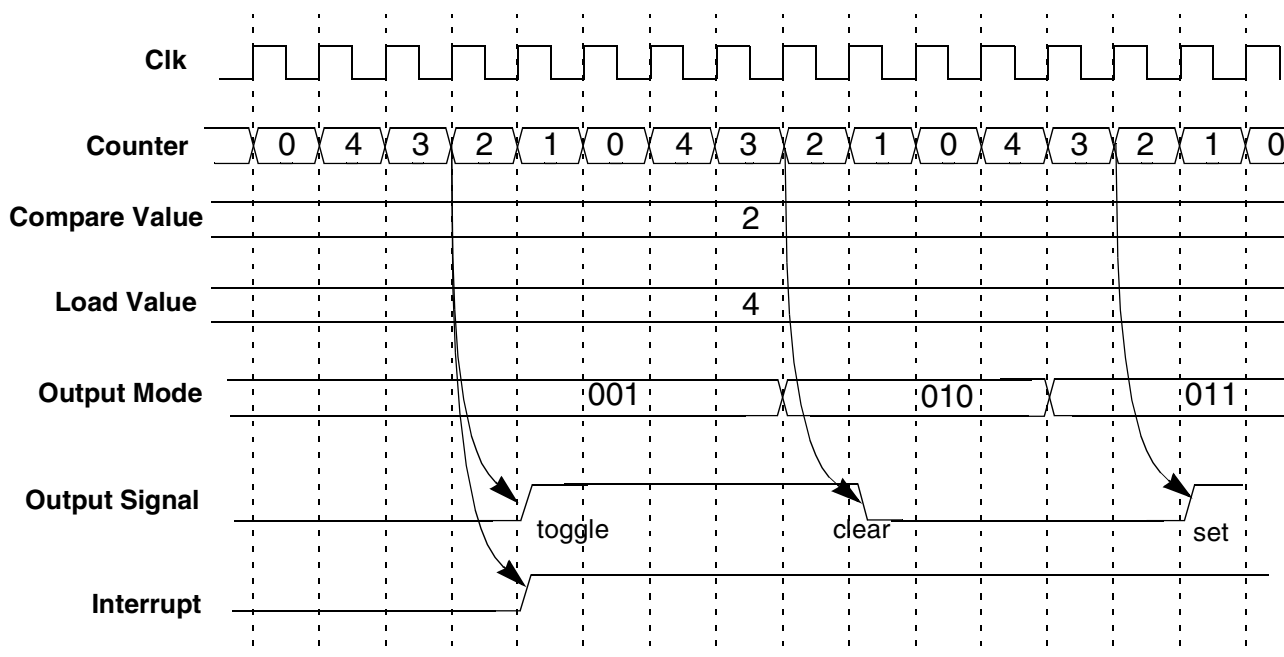
Figure 33-10. Compare Event and Interrupt Timing Diagram
