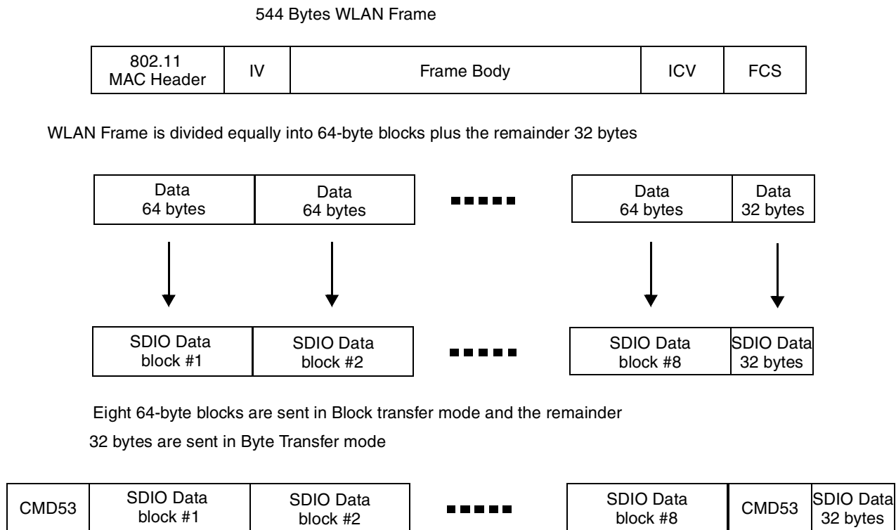
Figure 29-20. Example for Dividing Large Data Transfer
