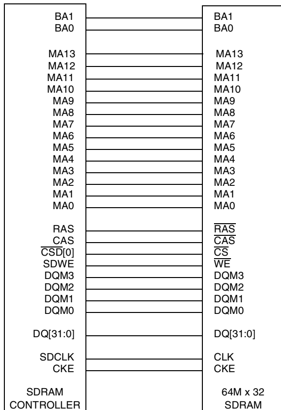
Figure 19-96. Single 2-Gbit (64Mx32) SDRAM Connection Diagram
