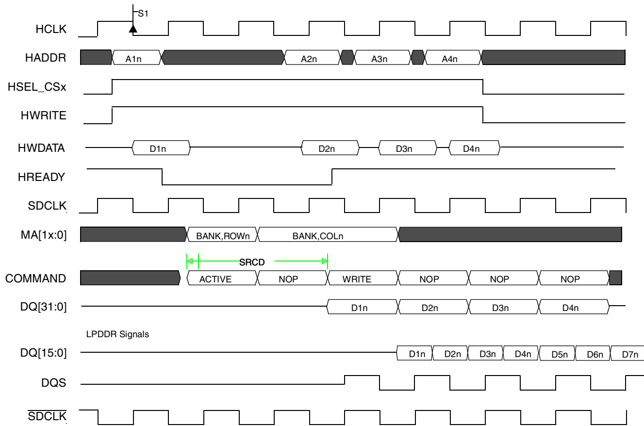
Figure 19-58. Off-Page Burst Write Timing Diagram (32-Bit Memory for SDR and 16-Bit for LPDDR)
