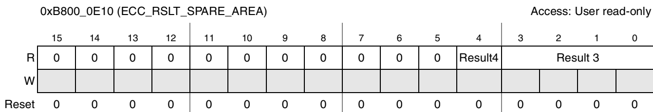
Figure 20-13. ECC_Rslt_Spare_Area Register
