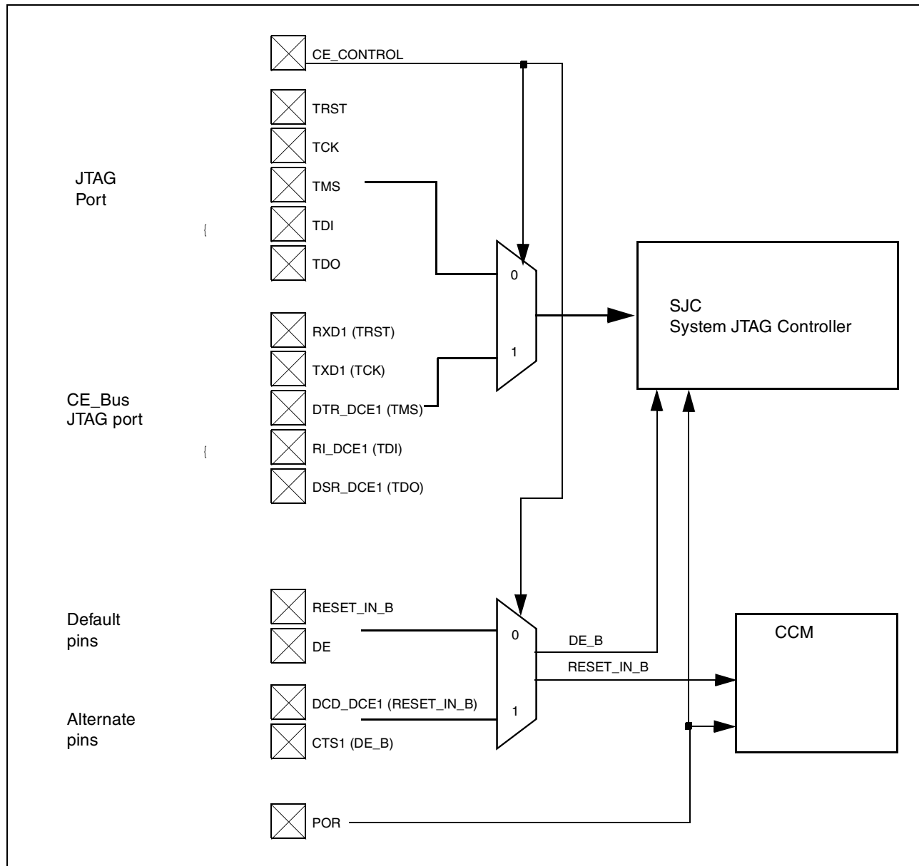
Figure 6-16. Bottom Connector/CE Supports
