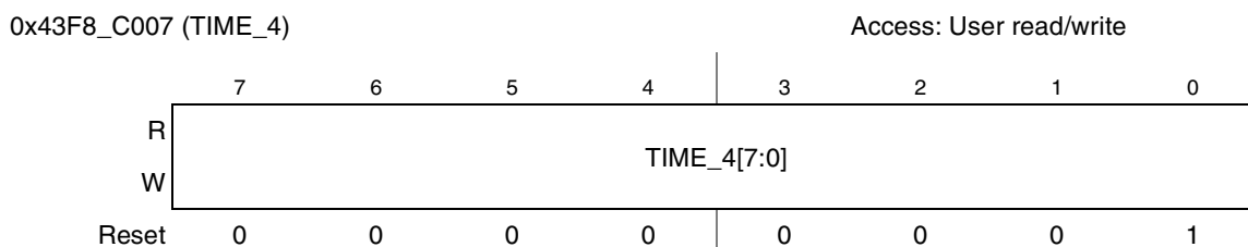
Figure 23-20. TIME_4 Register
