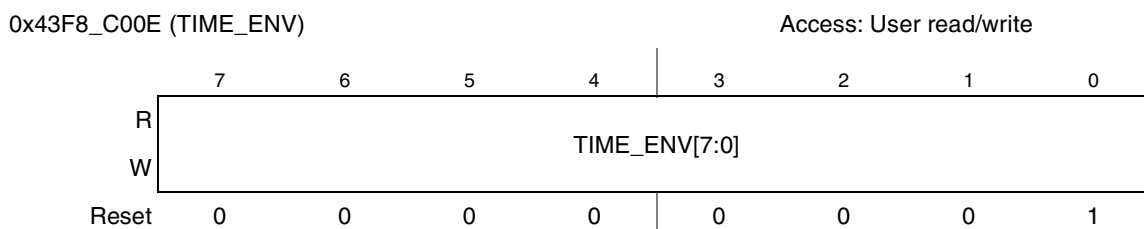
Figure 23-27. TIME_ENV Register
