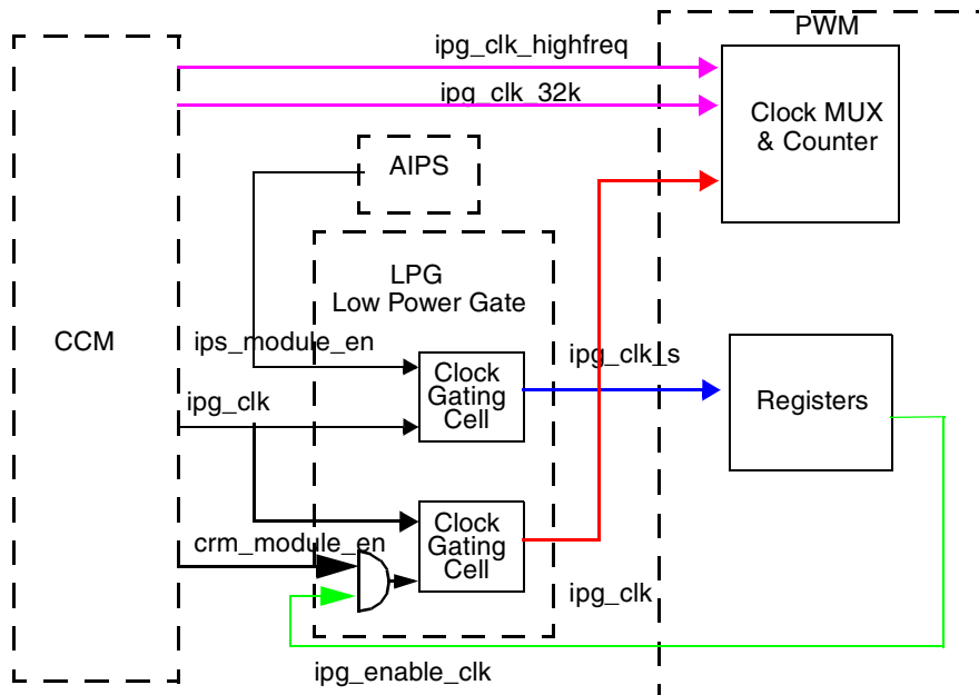
Figure 35-10. PWM Clocking
