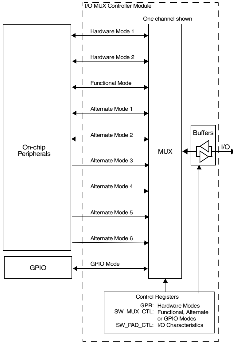
Figure 4-1. I/O Signal Multiplexing Block Diagram
