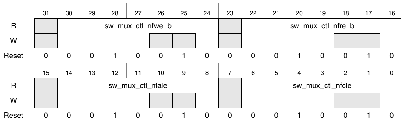
Figure 4-56. Register Description sw_mux_ctl_nfwe_b_nfre_b_nfale_nfcle
