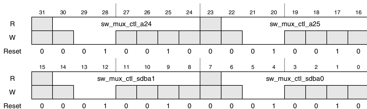
Figure 4-72. Register Description sw_mux_ctl_a24_a25_sdba1_sdba0
