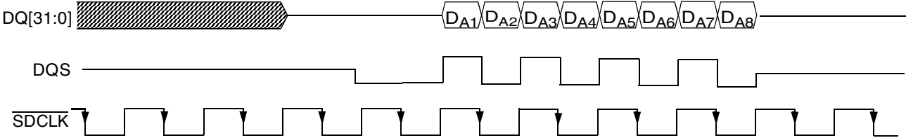
Figure 19-51. AHB 32-Bit Read from a LPDDR: Off-Page Burst Read Timing Diagram (32-Bit)
