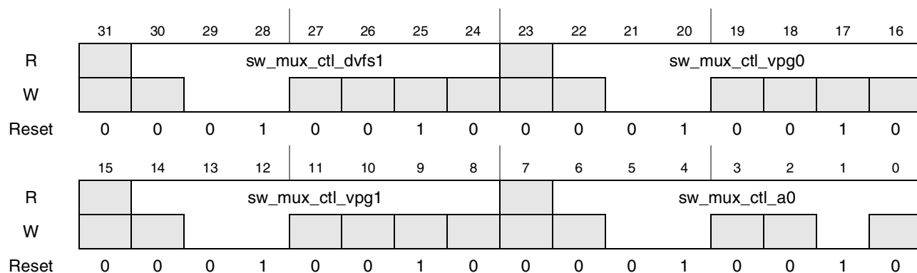
Figure 4-79. Register Description sw_mux_ctl_dvfs1_vpg0_vpg1_a0
