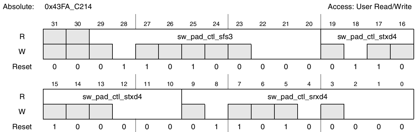
Figure 4-137. Register Description sw_pad_ctl_sfs3_stxd4_srx4
