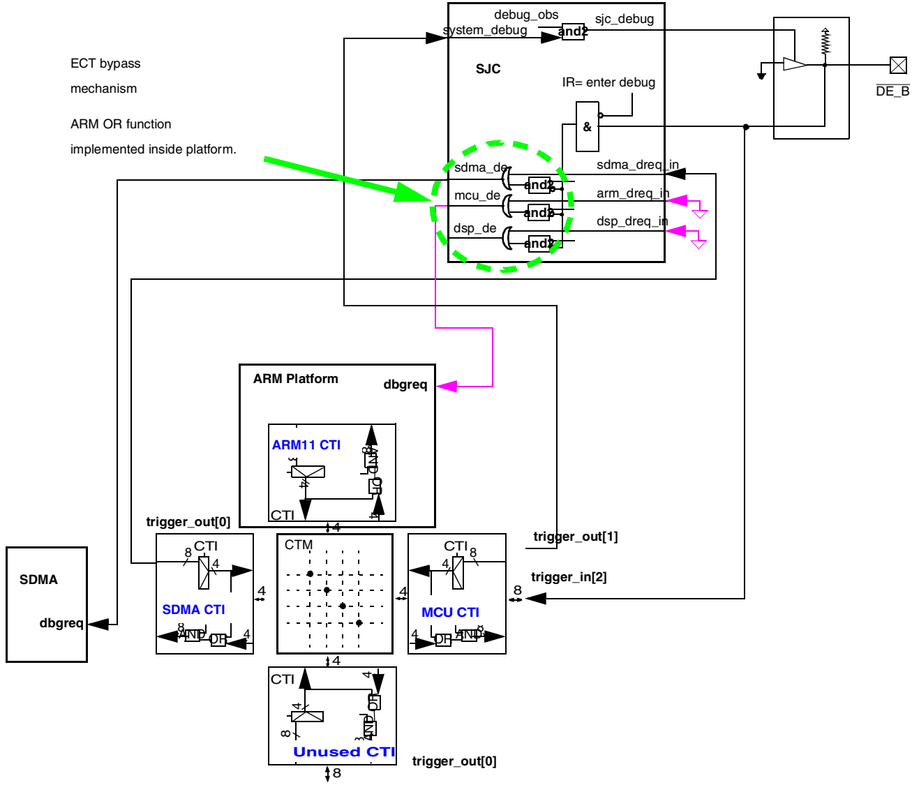
Figure 6-10. CTI-SJC Connectivity
