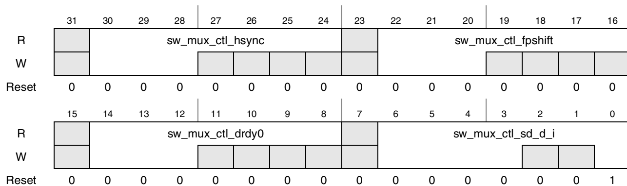
Figure 4-14. Register Description sw_mux_ctl_hsync_fpshift_drdy0_sd_d_i
