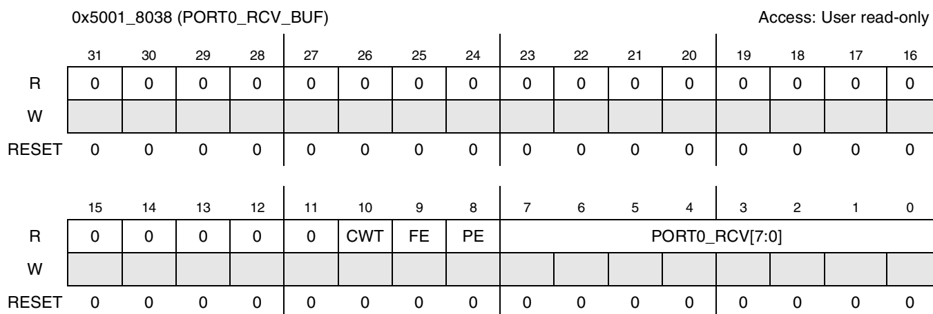
Figure 30-17. SIM Port0 Receive Buffer Register
