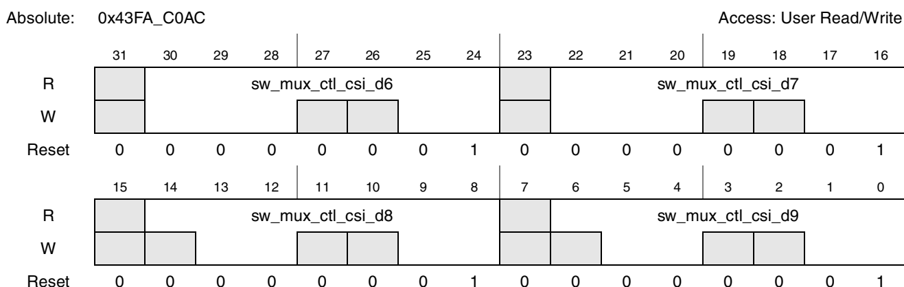
Figure 4-46. Register Description sw_mux_ctl_csi_d6_csi_d7_csi_d8_csi_d9
