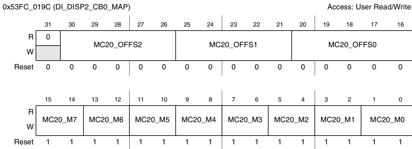
Figure 44-111. DI Display 2 Command Byte 0 Mapping Register (DI_DISP2_CB0_MAP)
