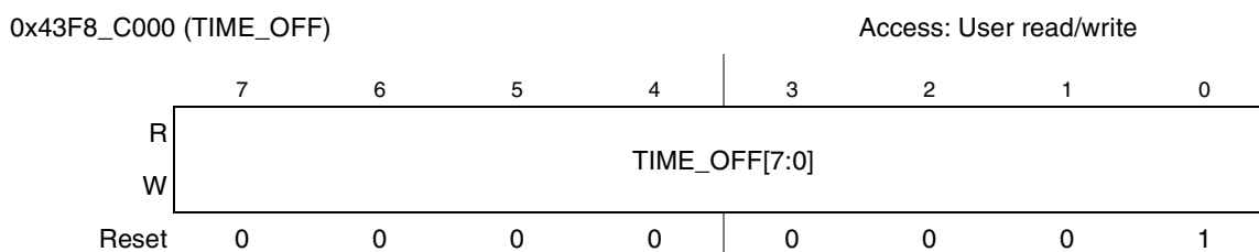
Figure 23-13. TIME_OFF Register
