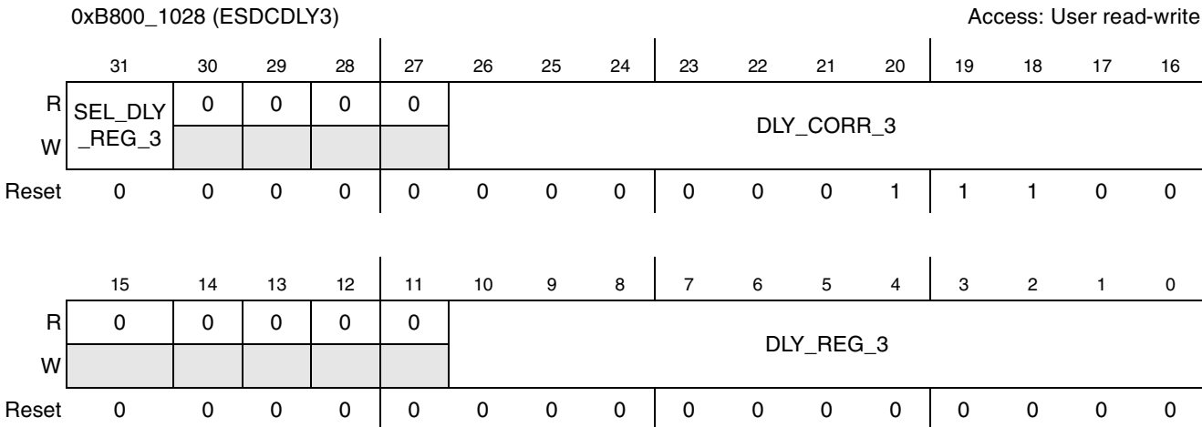
Figure 19-23. MDDR Delay Line 3 Configuration Debug Register
