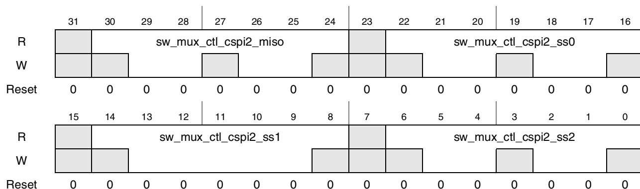
Figure 4-36. Register Description sw_mux_ctl_cspi2_miso_cspi2_ss0_cspi2_ss1_cspi2_ss2
