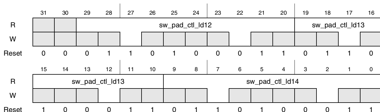
Figure 4-103. Register Description sw_pad_ctl_ld12_ld13_ld14
