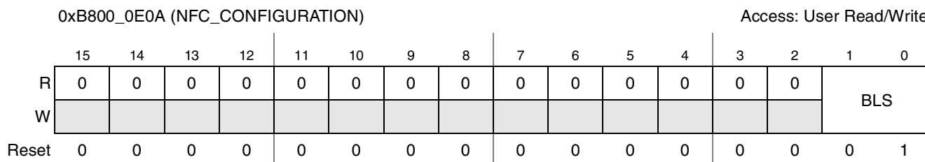
Figure 20-8. NFC_Configuration Register
