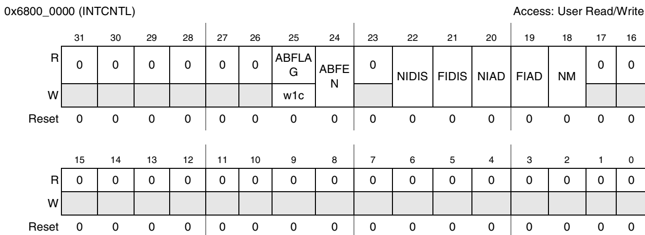
Figure 9-3. INTCNTL Register
