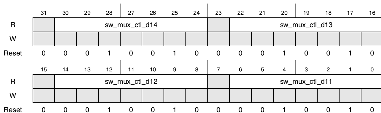
Figure 4-54. Register Description sw_mux_ctl_d14_d13_d12_d11
