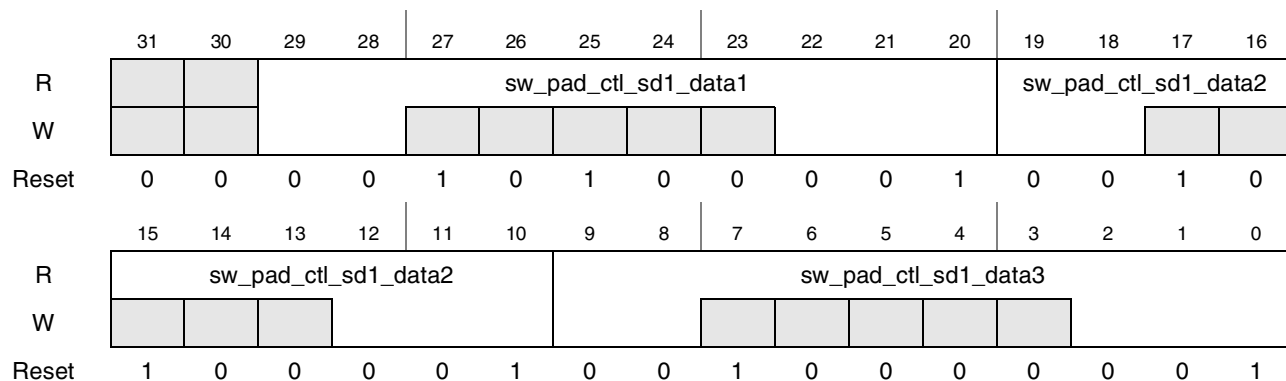
Figure 4-94. Register Description sw_pad_ctl_sd1_data1_sd1_data2_sd1_data3
