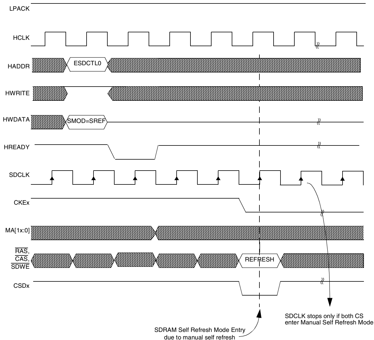
Figure 19-39. Manual Self Refresh Entry Timing Diagram
