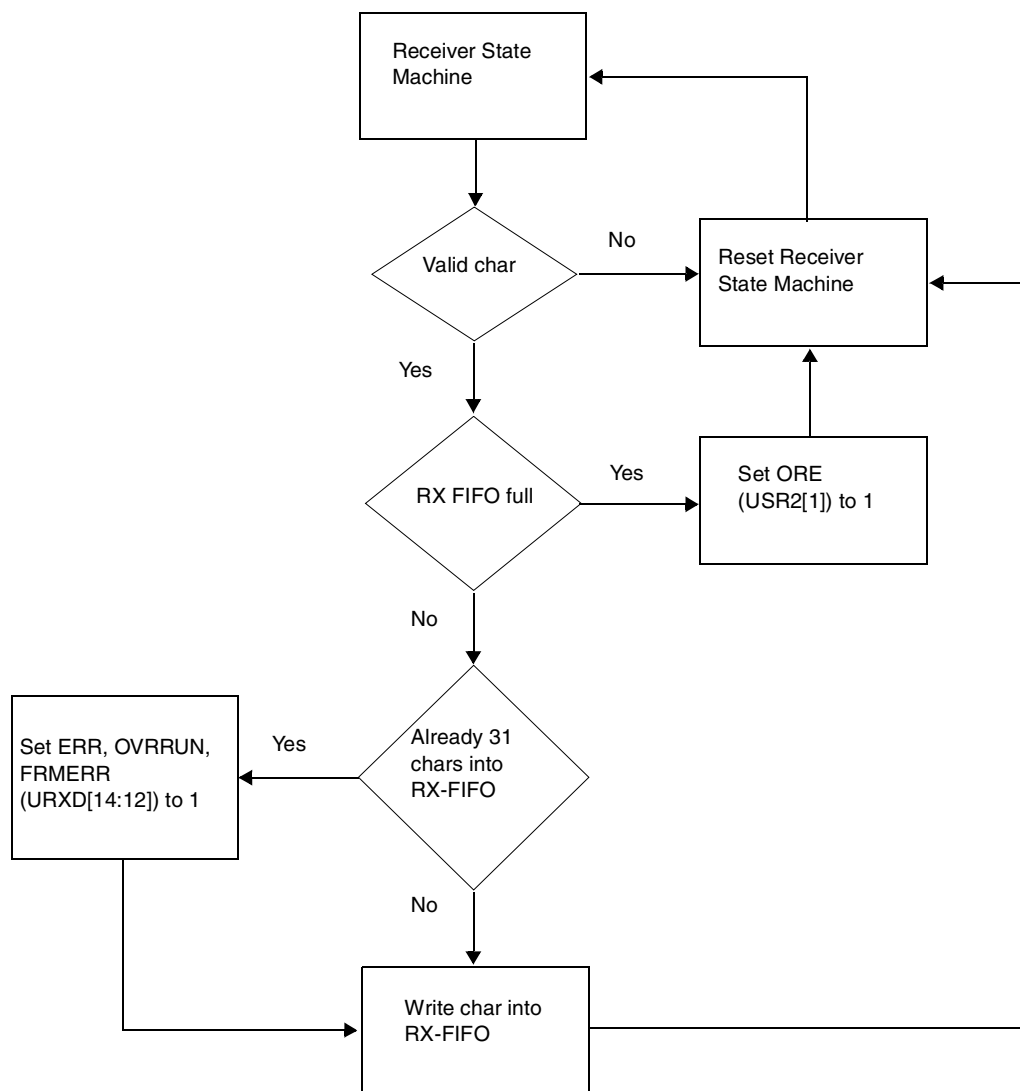
Figure 31-24. Receiver Flowchart
