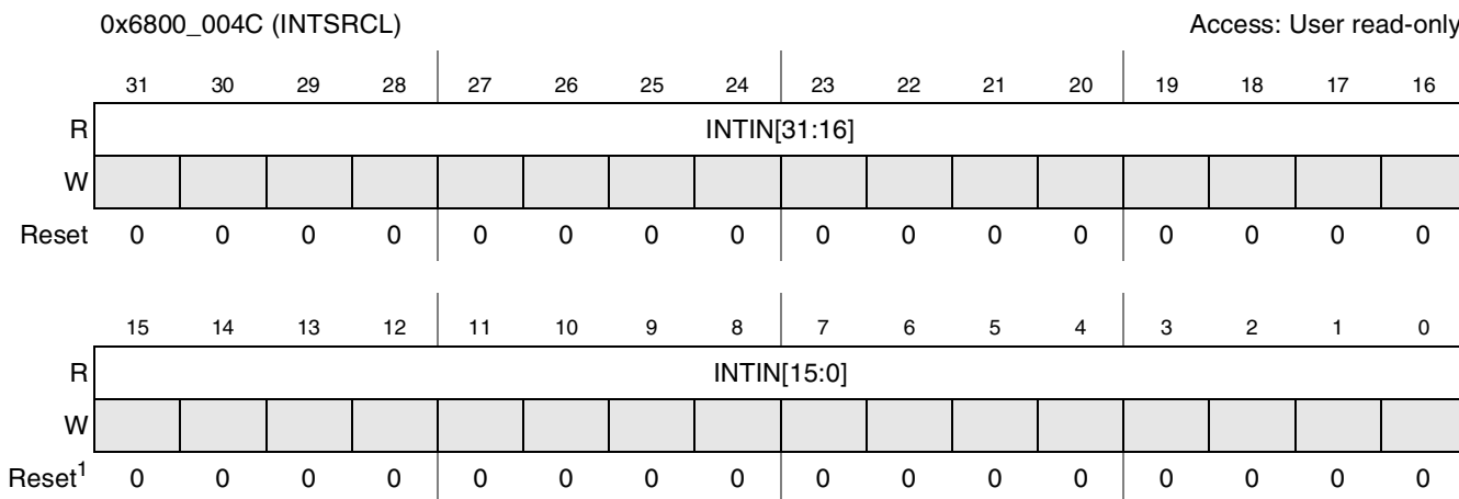
Figure 9-22. INTSRCL Register
