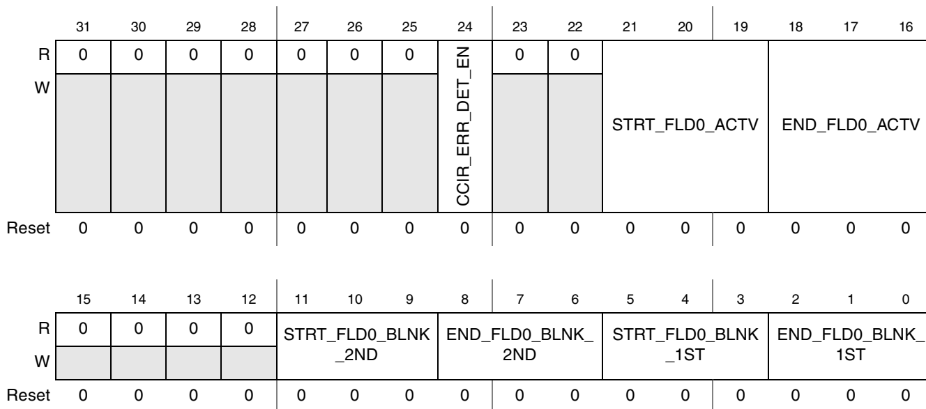
Figure 44-37. CSI CCIR Code Register 1 (CSI_CCIR_CODE_1)
