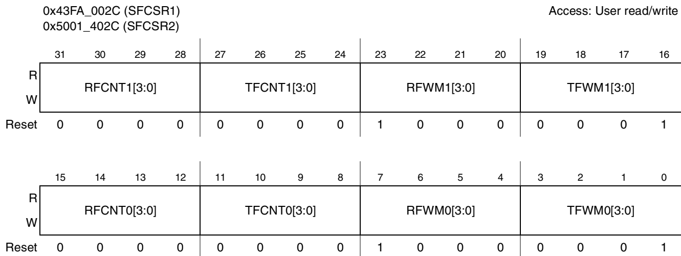
Figure 45-32. SSI FIFO Control/Status Register
