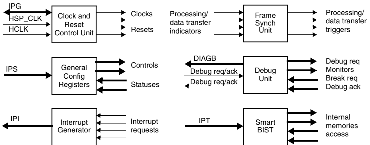
Figure 44-147. CM Block Diagram
