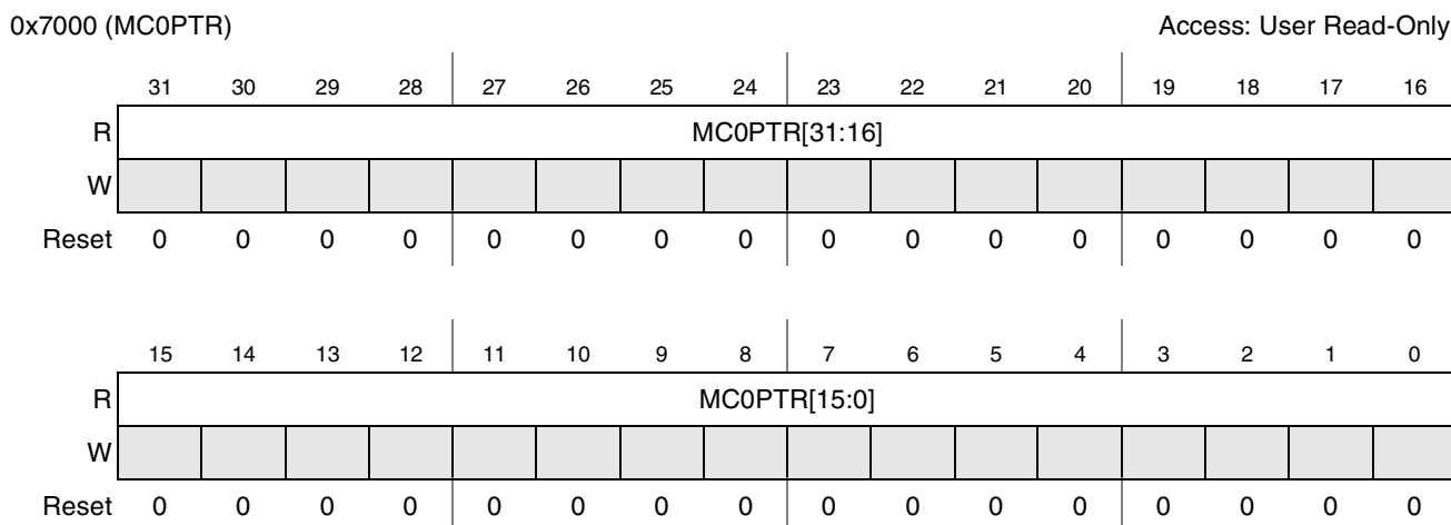
Figure 40-41. AP (MCU) Channel 0 Pointer (MCOPTR) Register
