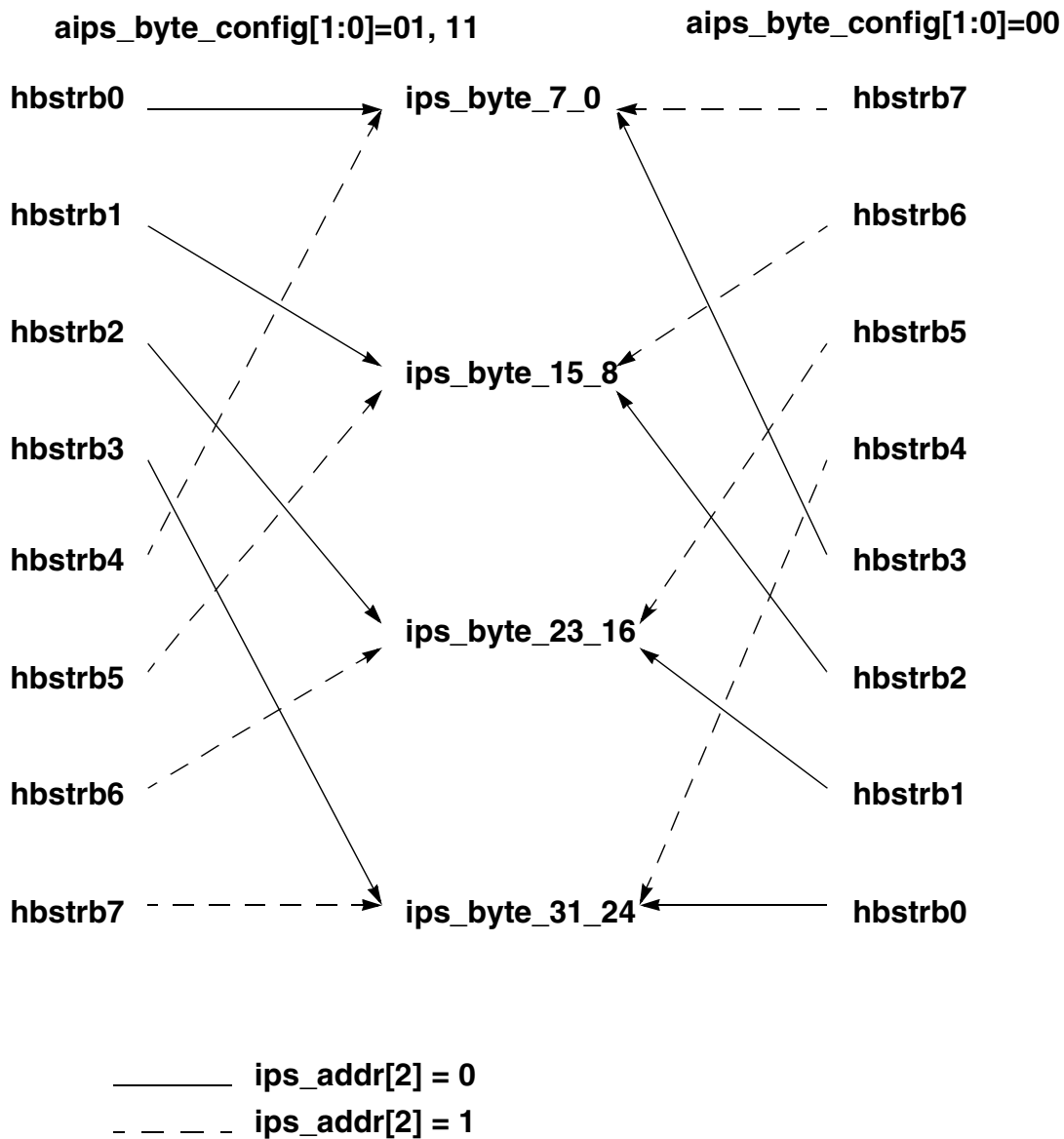
Figure 38-20. Mapping of 32-Bit Byte Strobes, 64-Bit System
