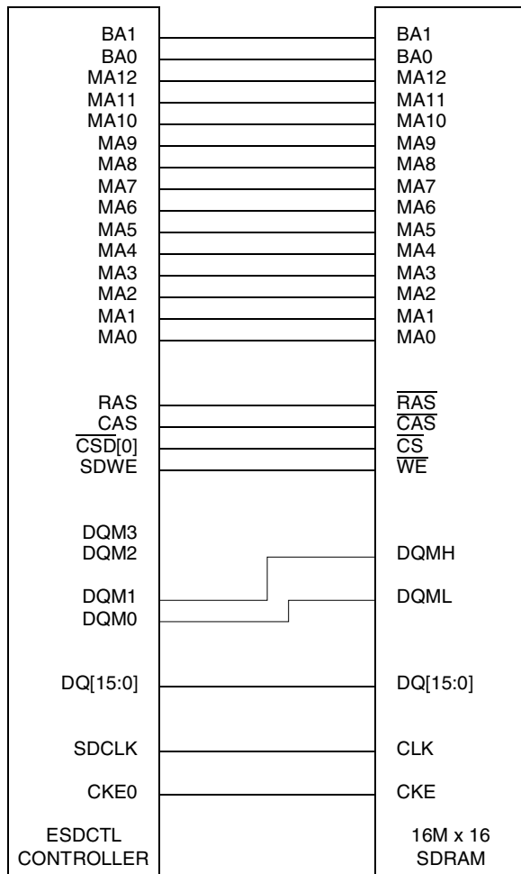
Figure 19-85. Single 256 Mbit (16M x 16) Connection Diagram
