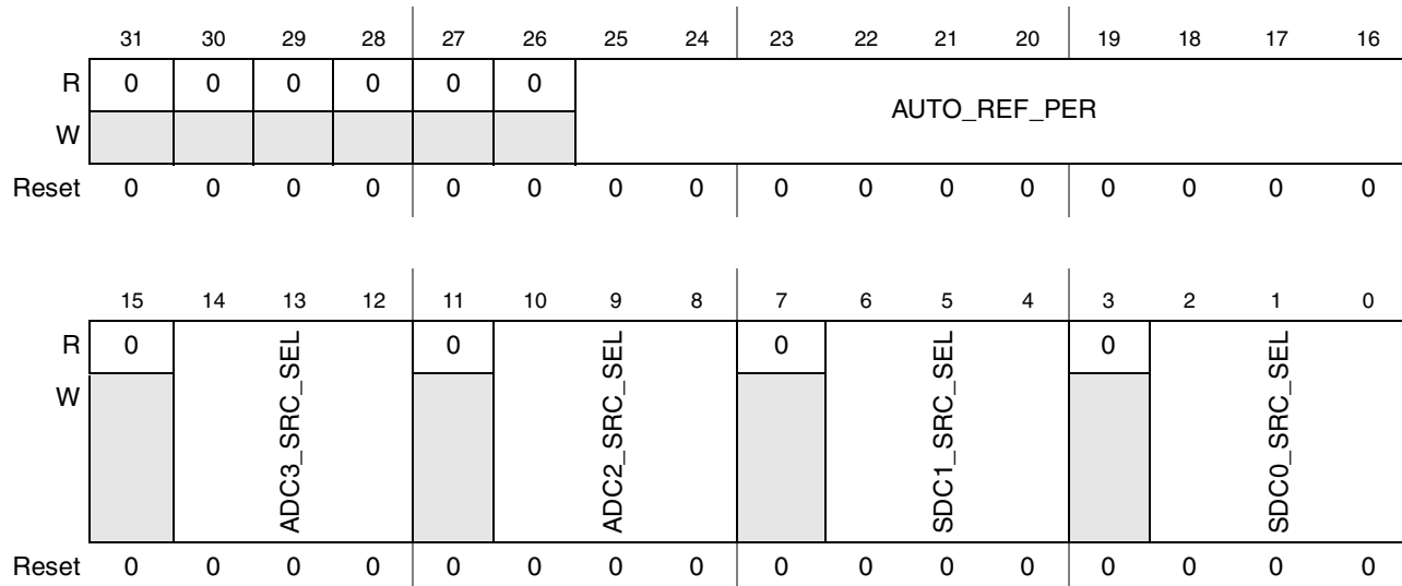
Figure 44-14. IPU Frame Synchronization Displaying Flow Register (IPU_FS_DISP_FLOW)
