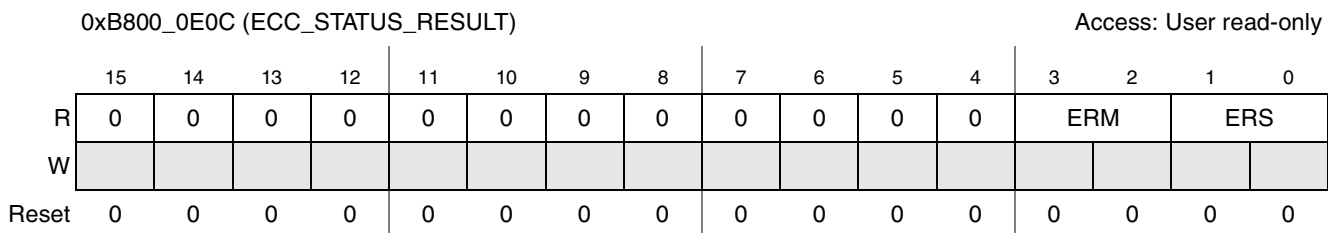
Figure 20-9. ECC_Status_Result
