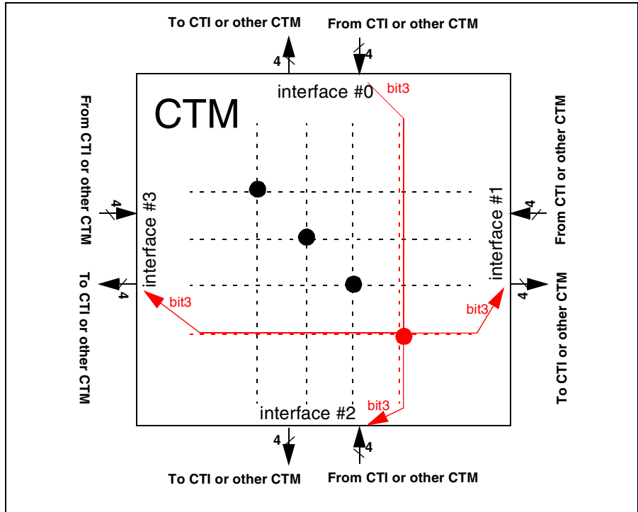
Figure 6-7. CTM Logic Bit Diagram
