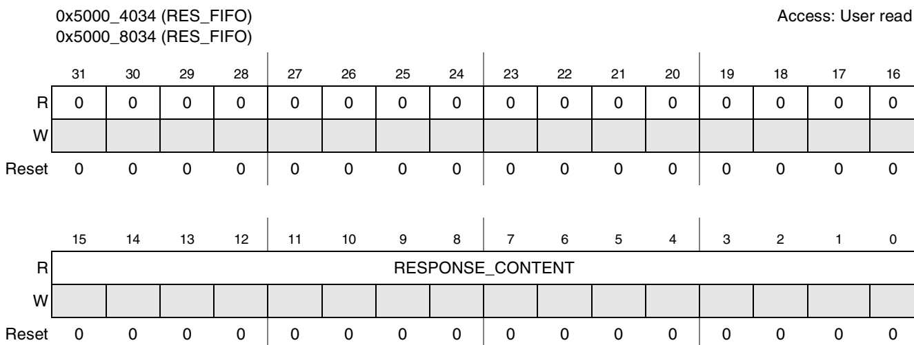
Figure 29-16. SDHC Response FIFO Register
