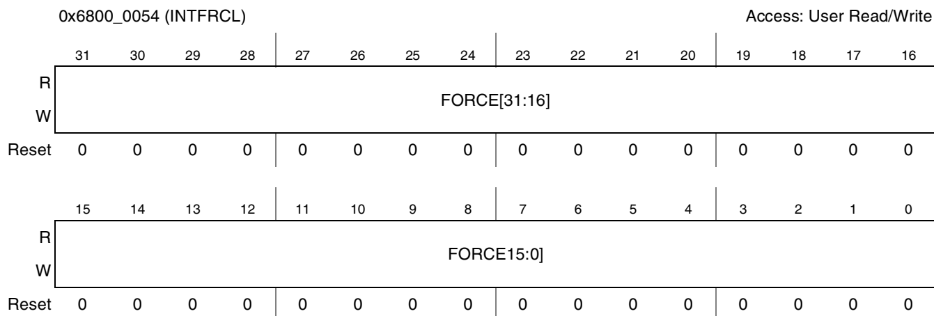
Figure 9-24. INTFRCL Register
