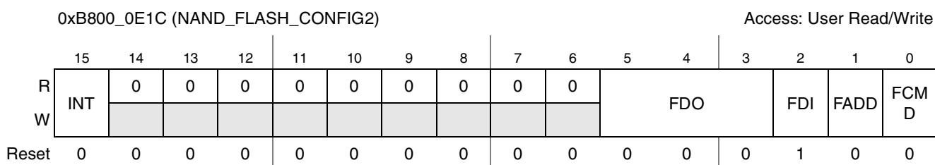
Figure 20-19. NAND_FLASH_CONFIG2 Register
