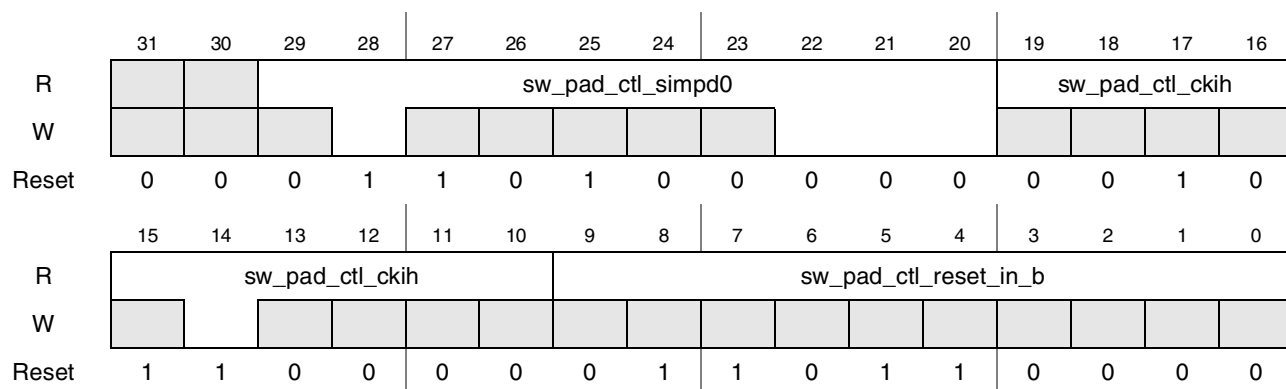
Figure 4-192. Register Description sw_pad_ctl_simpd0_ckih_reset_in_b
