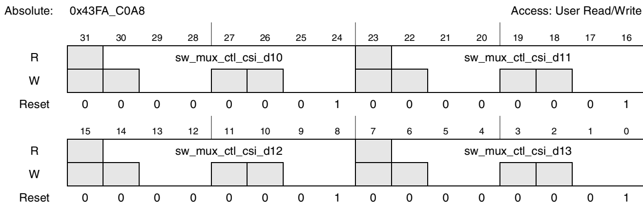
Figure 4-45. Register Description sw_mux_ctl_csi_d10_csi_d11_csi_d12_csi_d13
