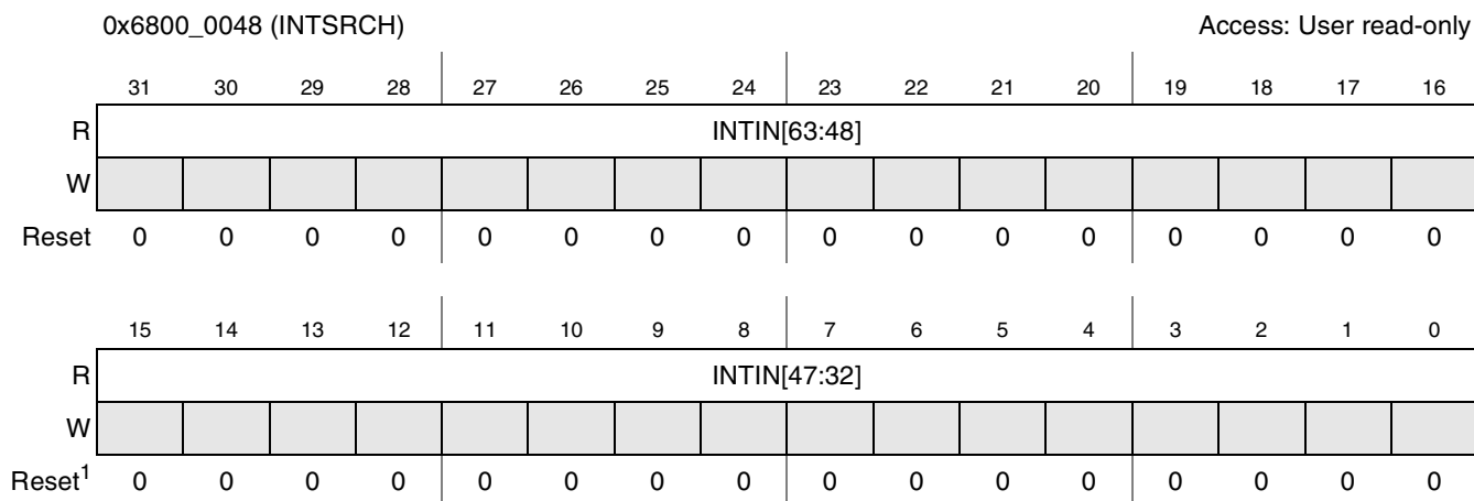
Figure 9-21. INTSRCH Register
