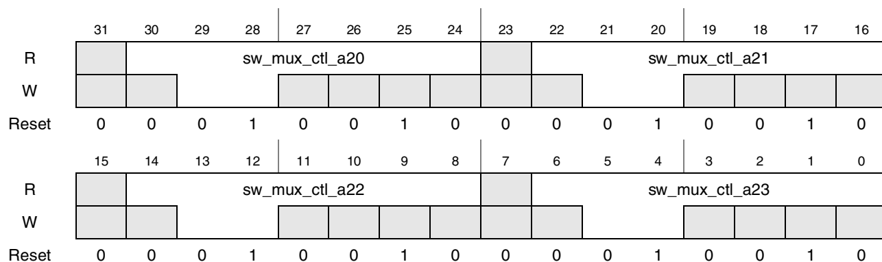
Figure 4-73. Register Description sw_mux_ctl_a20_a21_a22_a23
