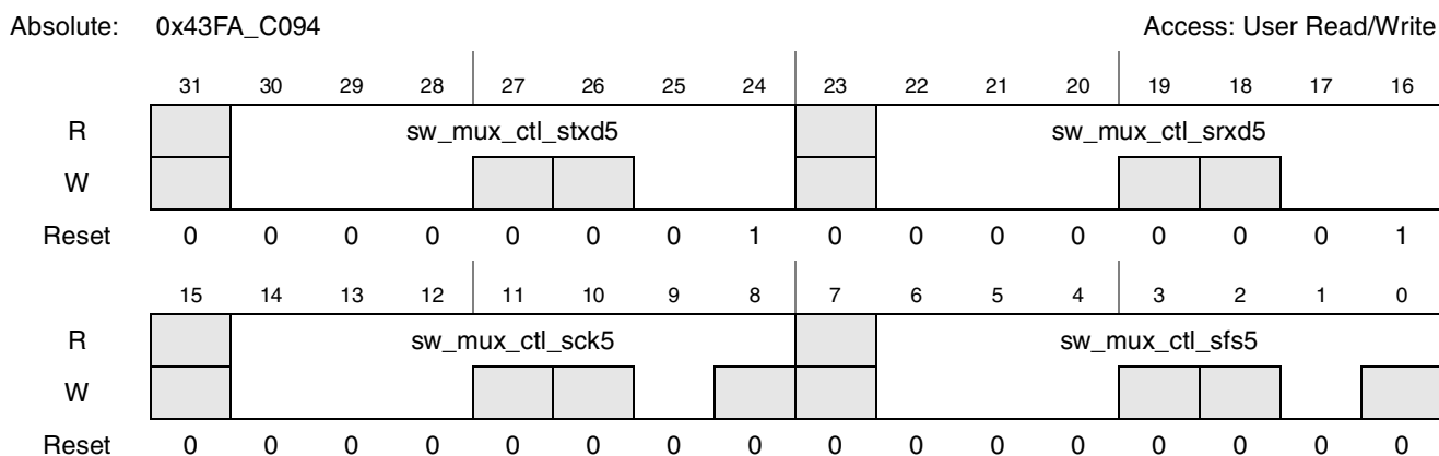
Figure 4-40. Register Description sw_mux_ctl_stxd5_srx5_sck5_sfs5
