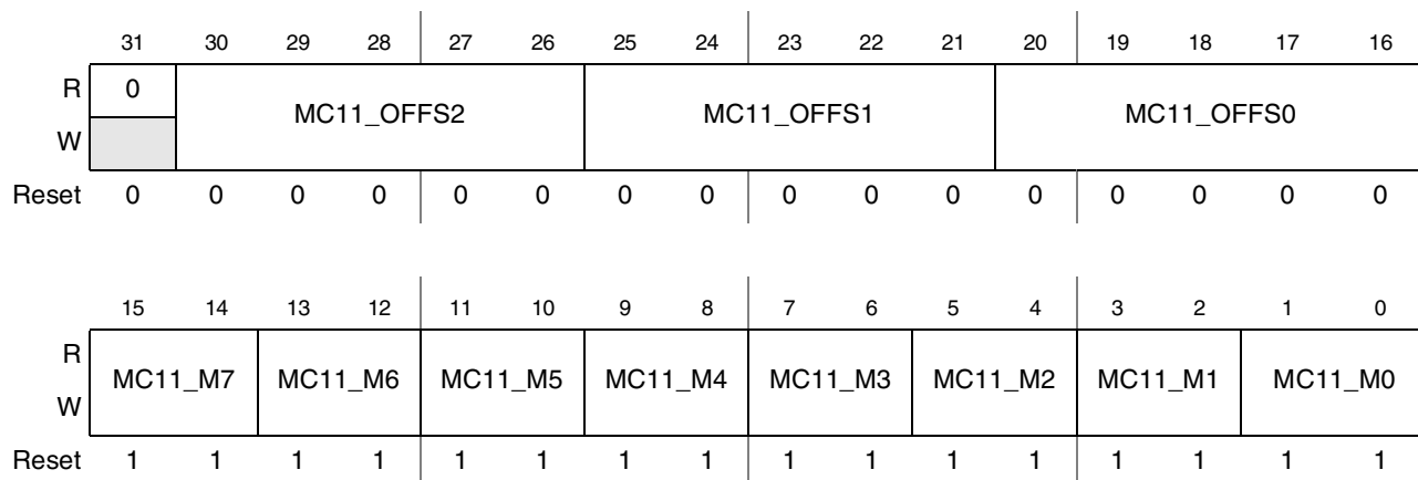
Figure 44-106. DI Display 1 Command Byte 1 Mapping Register (DI_DISP1_CB1_MAP)
