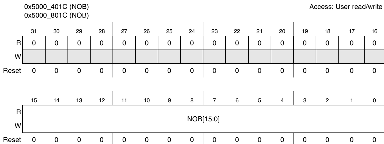
Figure 29-11. SDHC Number of Blocks Register
