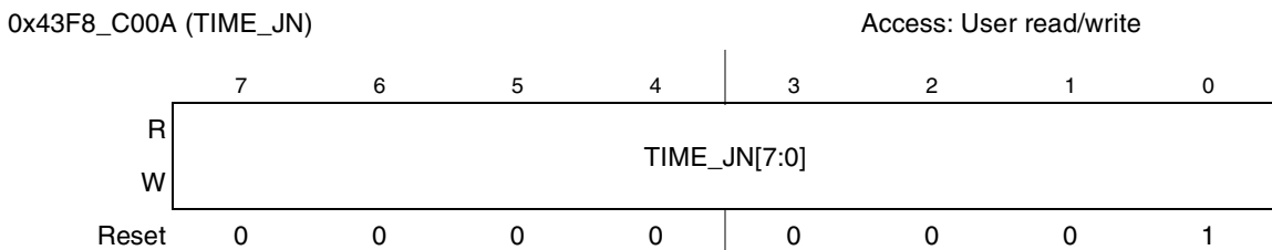
Figure 23-23. TIME_JN Register
