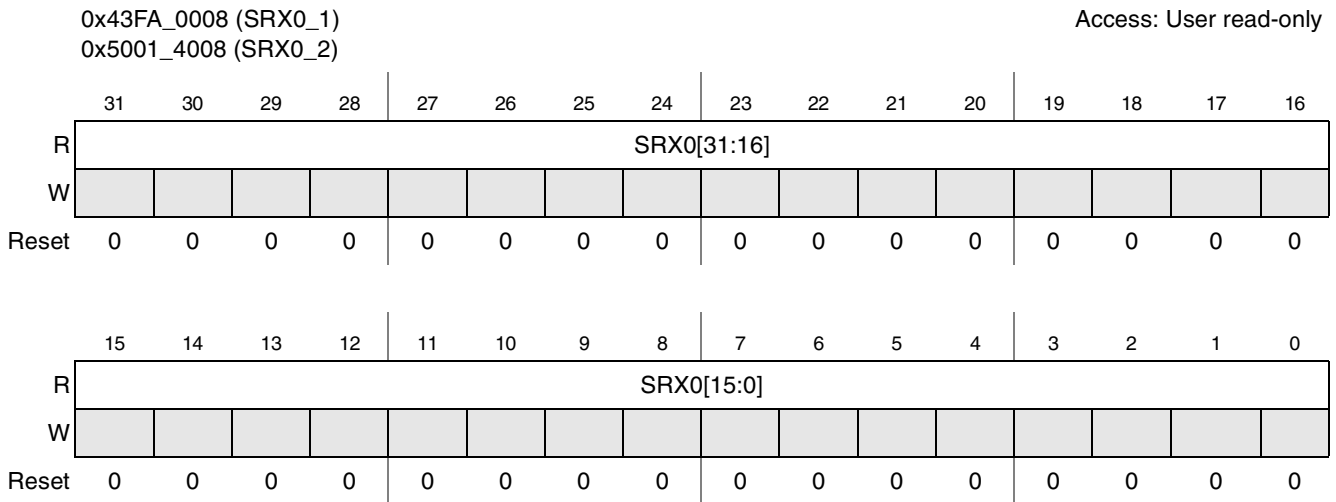
Figure 45-18. SSI0 Receive Data Register
