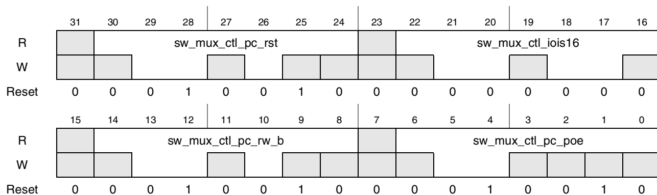
Figure 4-48. Register Description sw_mux_ctl_pc_rst_iois16_pc_rw_b_pc_poe
