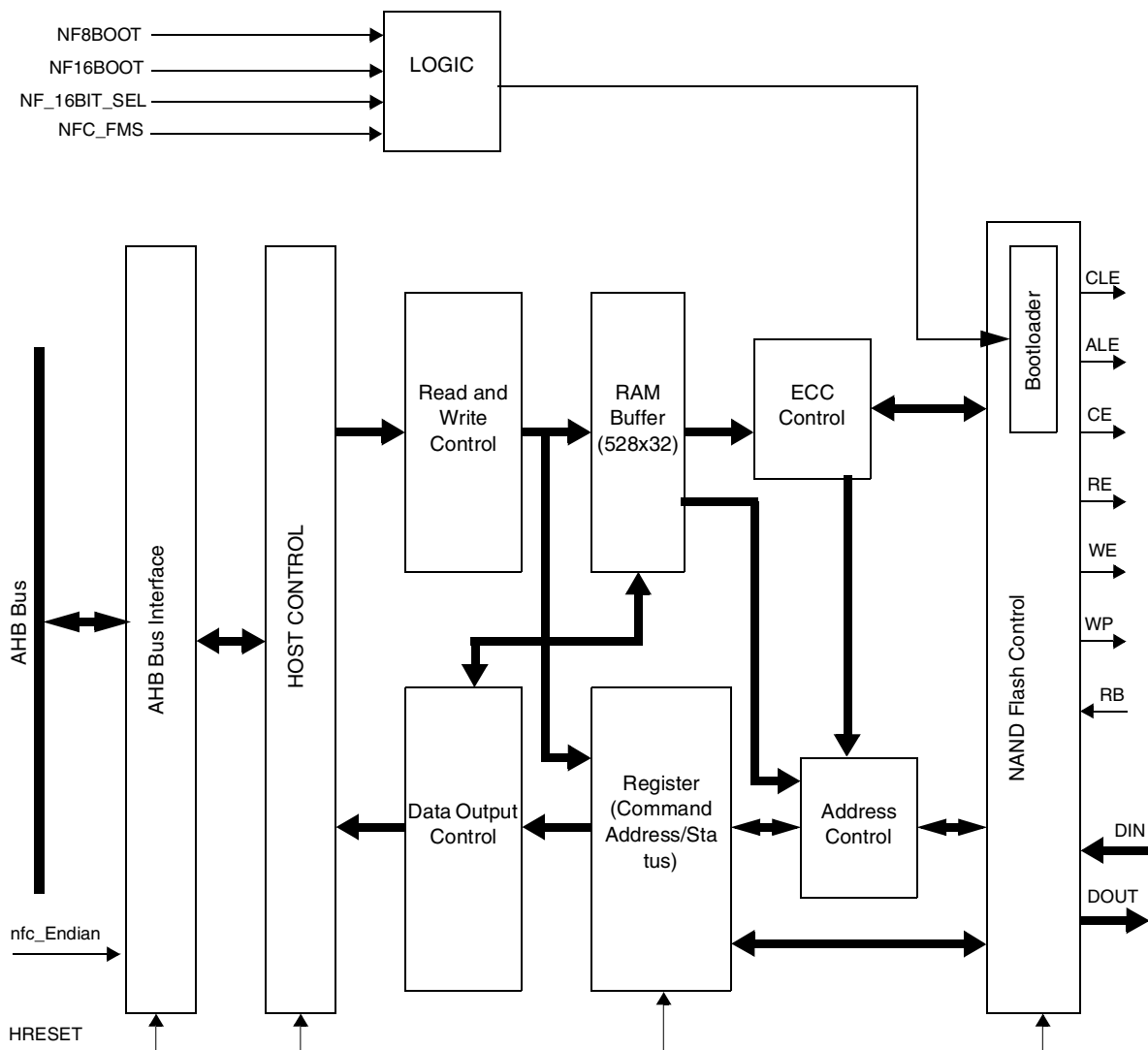
Figure 20-1. NAND Flash Controller Block Diagram
