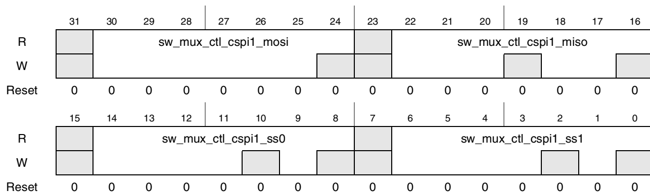
Figure 4-38. Register Description sw_mux_ctl_cspi1_mosi_cspi1_miso_cspi1_ss0_cspi1_ss1
