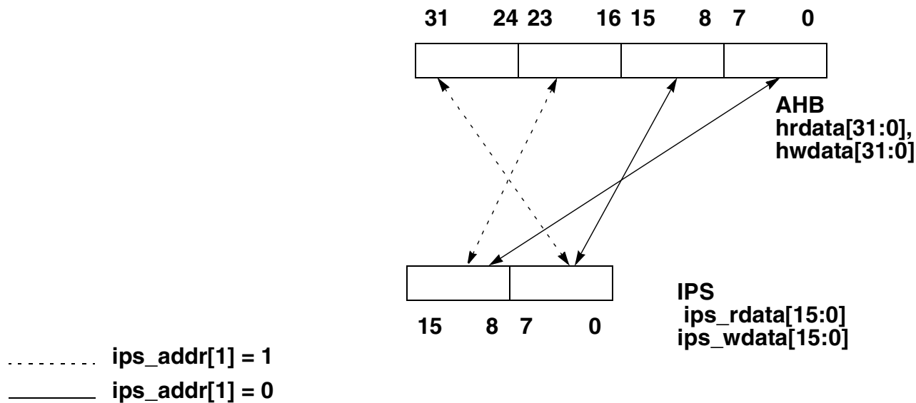
Figure 38-25. Data Bus Byte Lane Mapping for 16-Bit Peripherals, 32-Bit System, aips_byte_config[1:0] = 00
