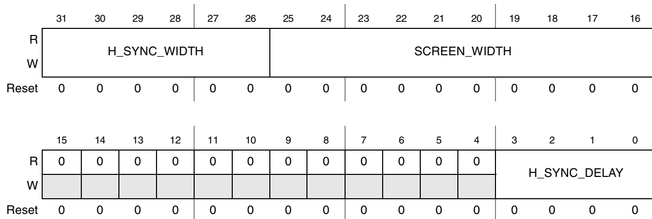
Figure 44-60. SDC Horizontal Configuration Register (SDC_HOR_CONF)
