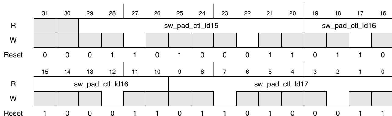
Figure 4-102. Register Description sw_pad_ctl_ld15_ld16_ld17
