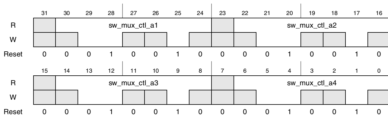
Figure 4-78. Register Description sw_mux_ctl_a1_a2_a3_a4
