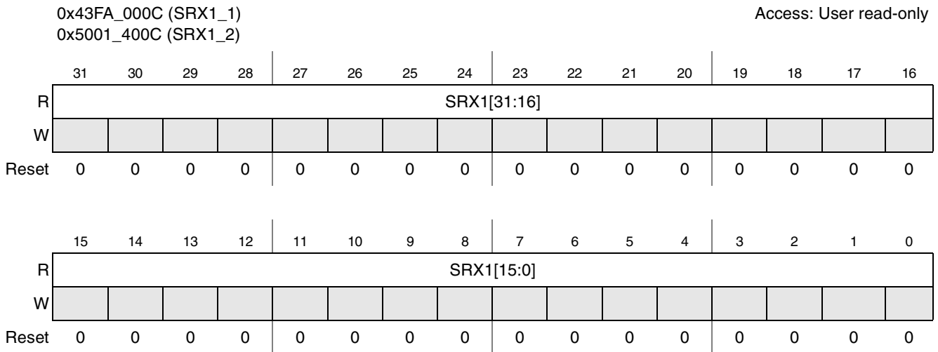
Figure 45-19. SSI1 Receive Data Register
