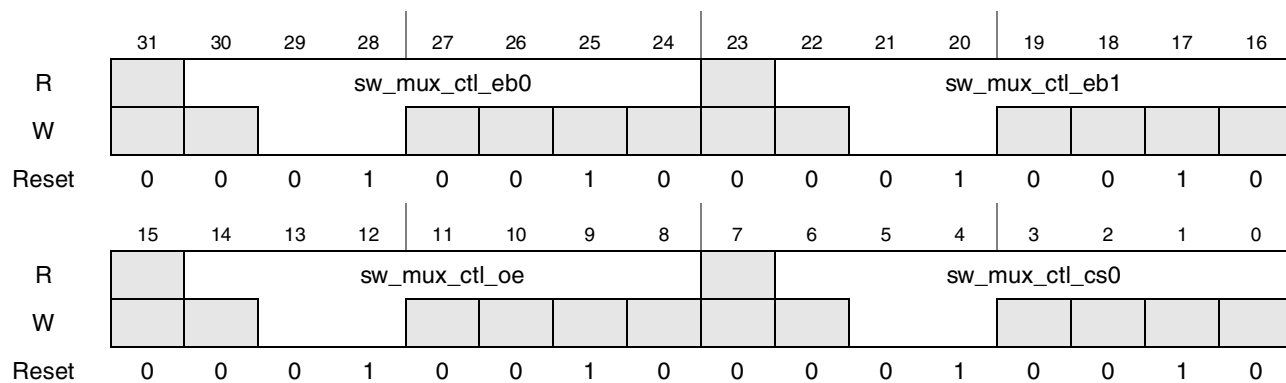
Figure 4-62. Register Description sw_mux_ctl_eb0_eb1_oe_cs0
