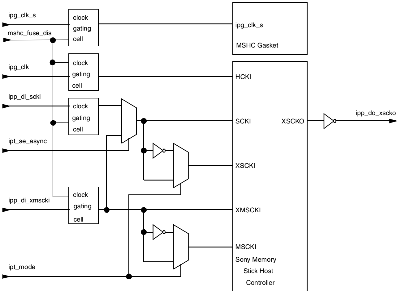
Figure 28-6. MSHC Clock Structure
