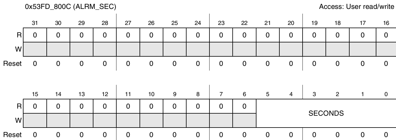
Figure 36-6. RTC Seconds Alarm Register
