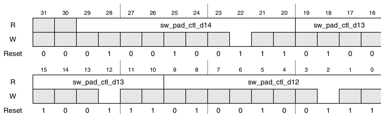
Figure 4-154. Register Description sw_pad_ctl_d14_d13_d12
