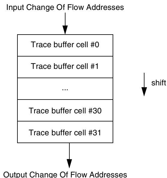
Figure 40-72. Trace Buffer
