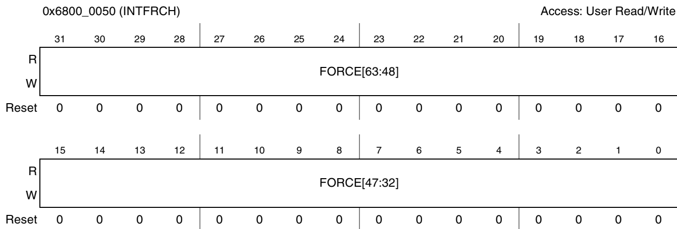
Figure 9-23. INTFRCH Register
