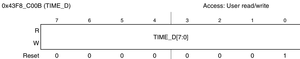
Figure 23-24. TIME_D Register
