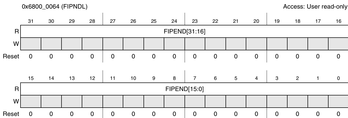
Figure 9-28. FIPNDL Register
