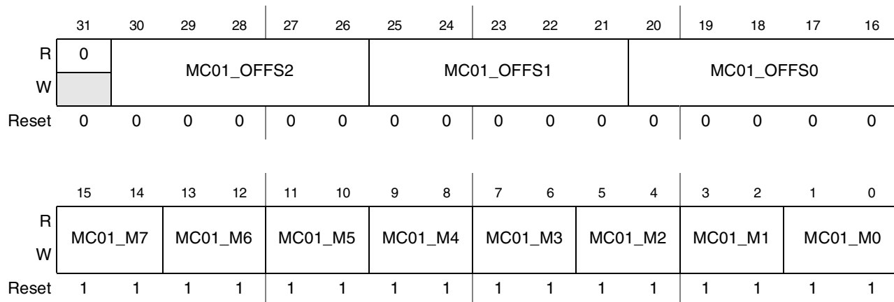
Figure 44-100. DI Display 0 Command Byte 1 Mapping Register (DI_DISP0_CB1_MAP)
