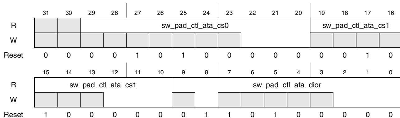
Figure 4-93. Register Description sw_pad_ctl_ata_cs0_ata_cs1_ata_dior
