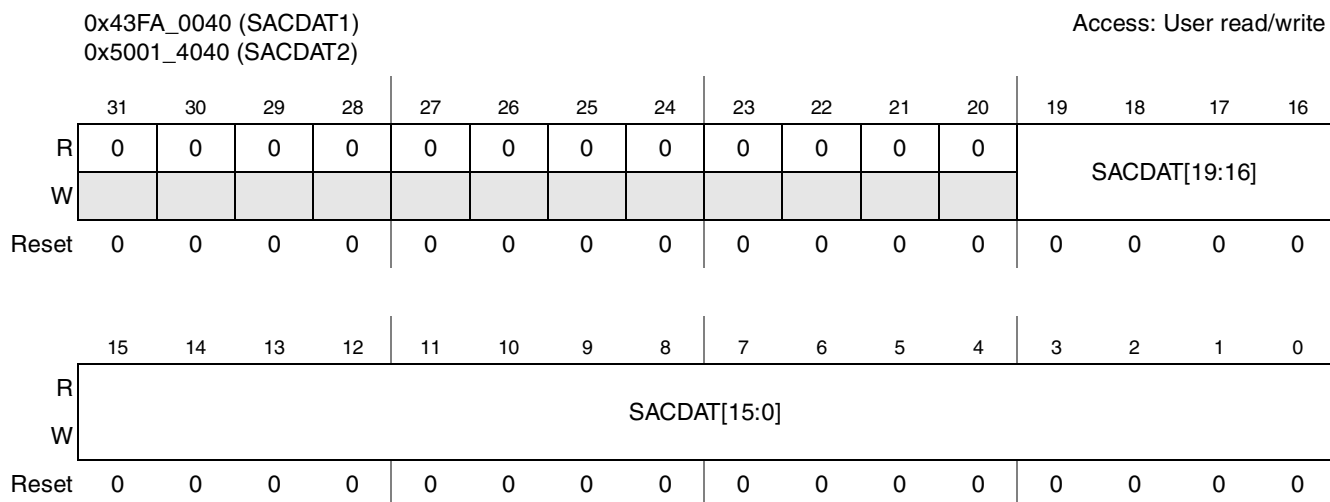
Figure 45-35. SSI AC97 Command Data Register
