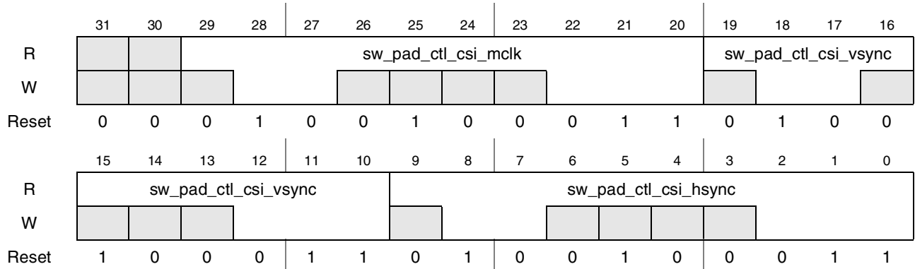
Figure 4-140. Register Description sw_pad_ctl_csi_mclk_csi_vsync_csi_hsync
