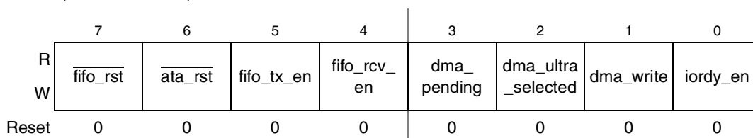
Figure 23-40. ATA_CONTROL Register
