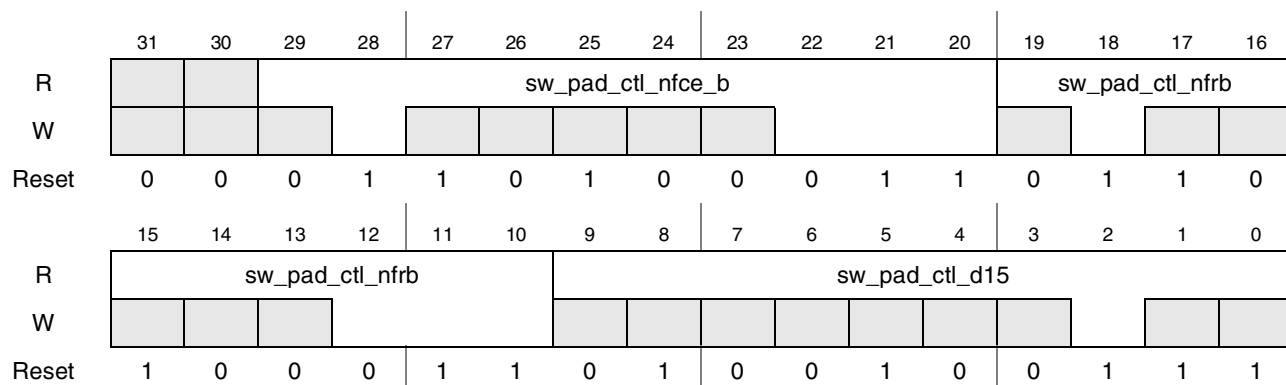
Figure 4-155. Register Description sw_pad_ctl_nfce_b_nfrb_d15
