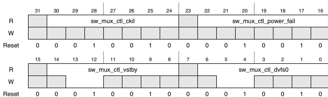
Figure 4-80. Register Description sw_mux_ctl_ckil_power_fail_vstby_dvfs0
