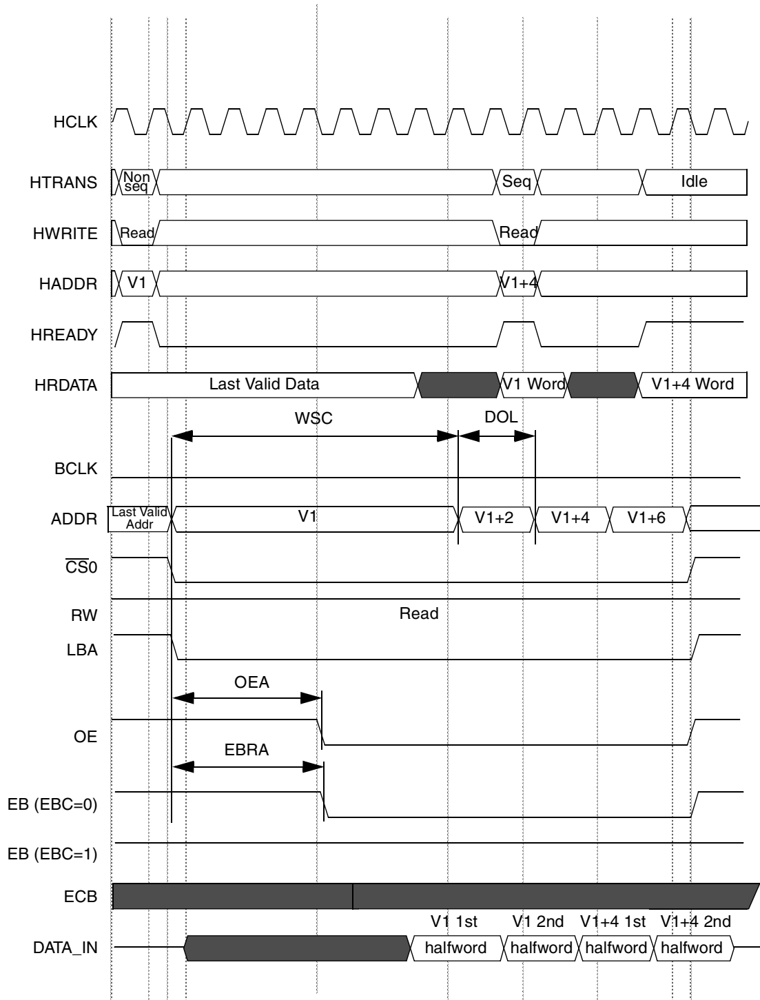
Figure 18-25. Sequential Read Access, WSC=7, OEA=8, PME=1, SYNC=1, DOL=1, EBRA=8
