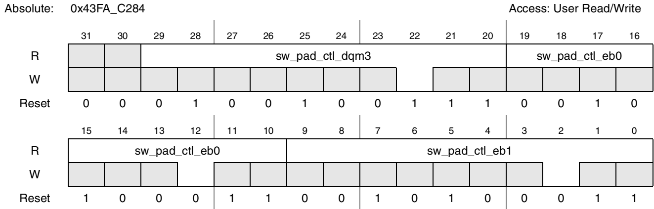
Figure 4-165. Register Description sw_pad_ctl_dqm3_eb0_eb1
