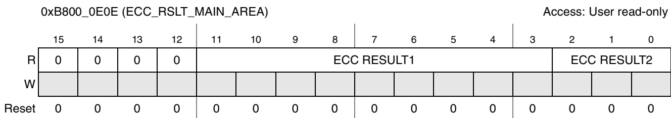
Figure 20-10. ECC_RSLT_MAIN_AREA Register
