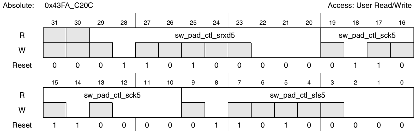
Figure 4-135. Register Description sw_pad_ctl_srx5_sck5_sfs5
