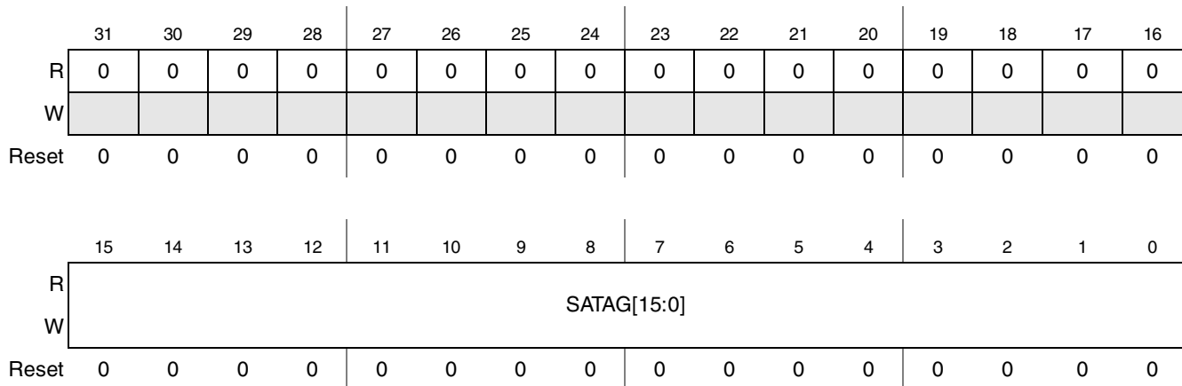
Figure 45-36. SSI AC97 Tag Register
