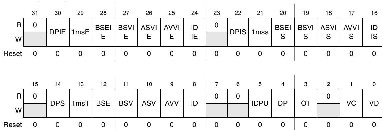
Figure 32-36. OTGSC—OTG Status Control
