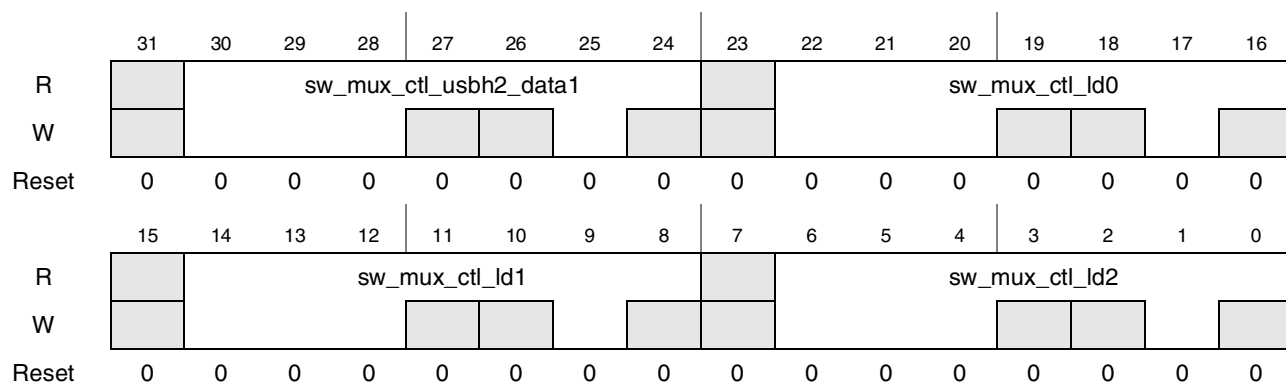
Figure 4-19. Register Description sw_mux_ctl_usbh2_data1_ld0_ld1_ld2
