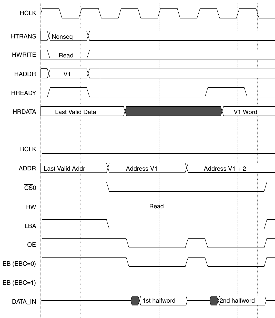
Figure 18-14. Read Access, WSC=1, OEA=1, EBRA=1
