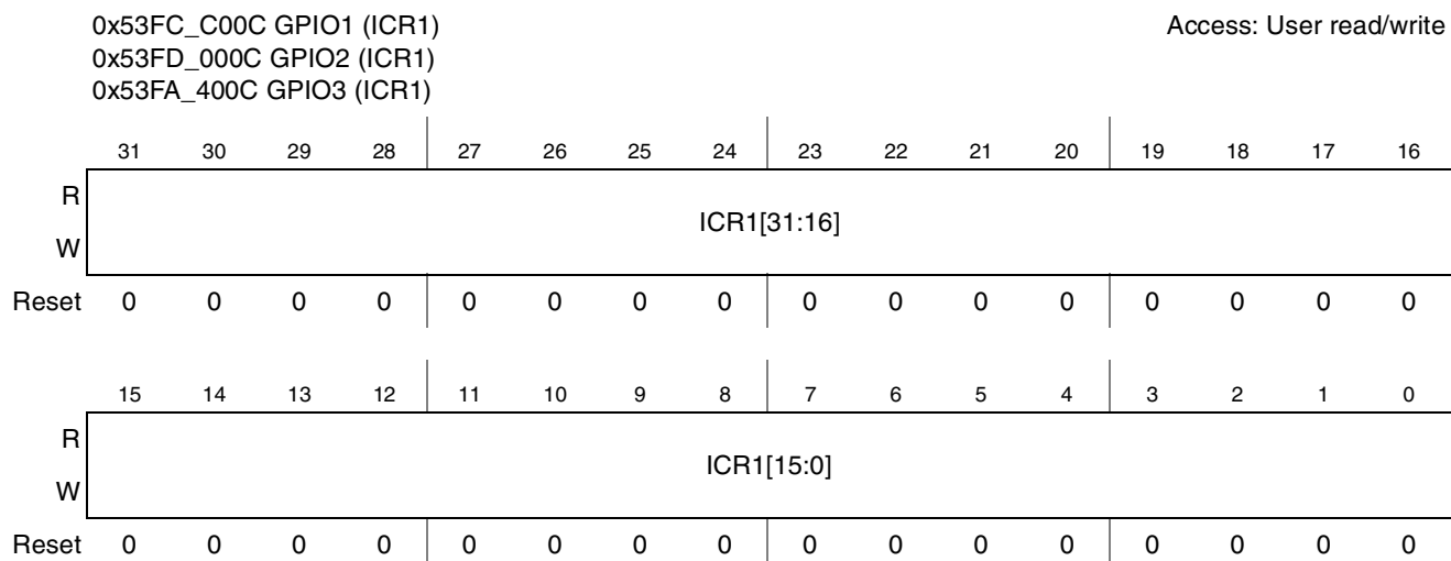
Figure 5-7. GPIO Interrupt Configuration Register1 (ICR1)
