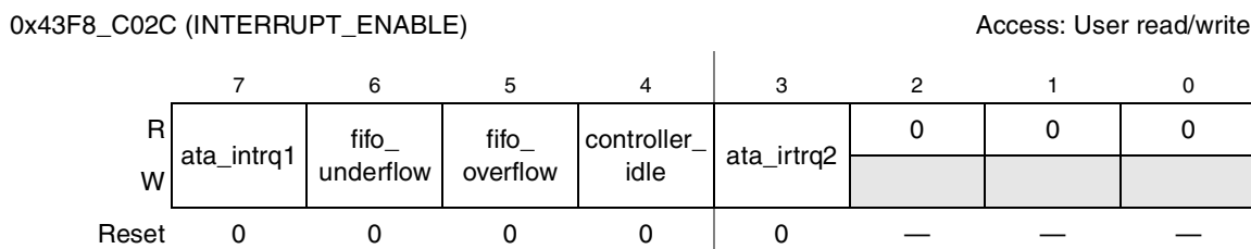
Figure 23-42. INTERRUPT_ENABLE Register
