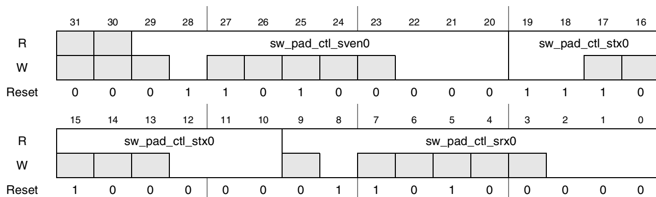
Figure 4-193. Register Description sw_pad_ctl_sven0_stx0_srx0
