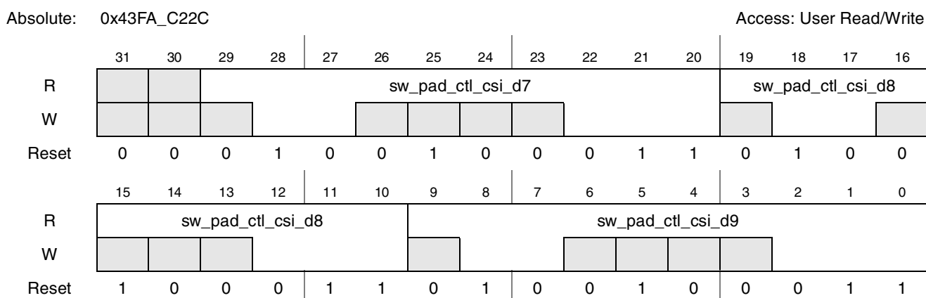
Figure 4-143. Register Description sw_pad_ctl_csi_d7_csi_d8_csi_d9
