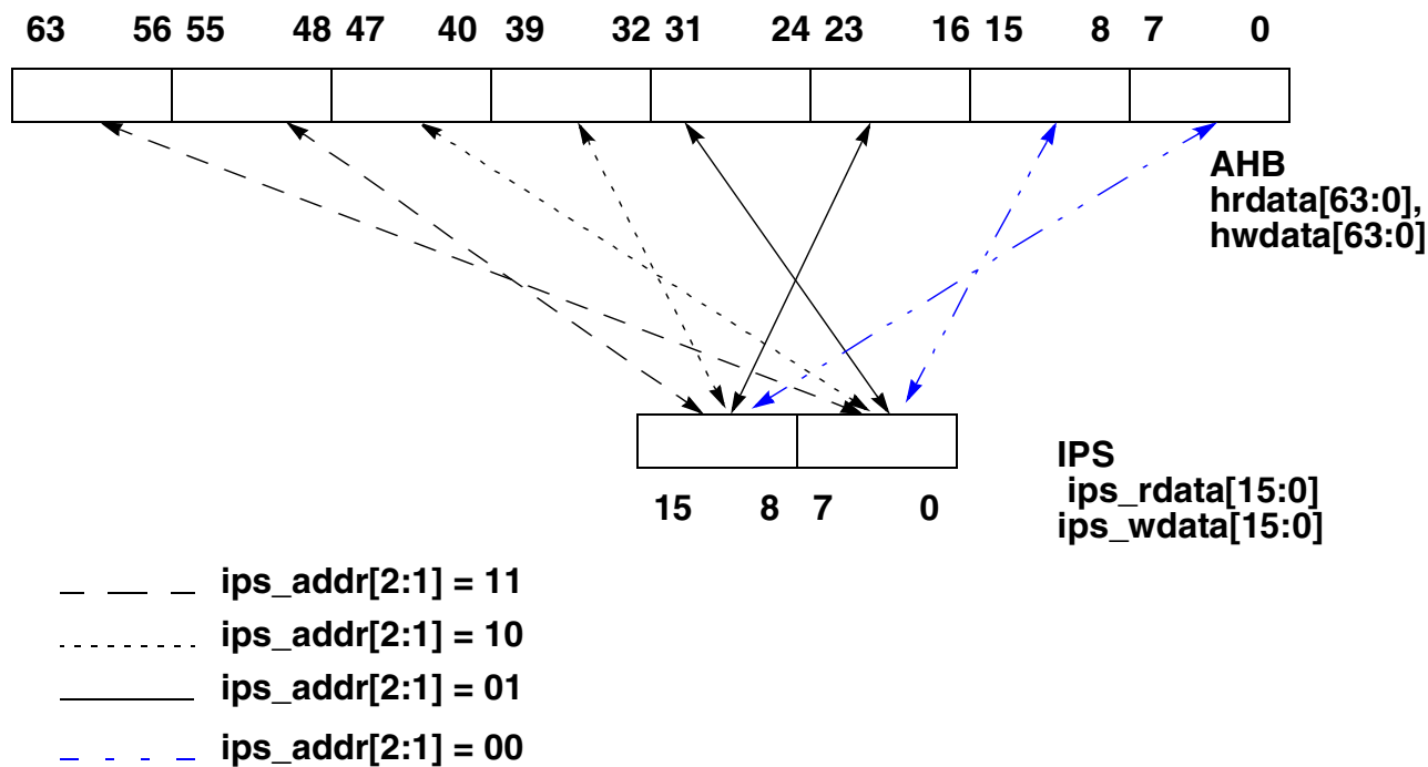
Figure 38-22. Data Bus Byte Lane Mapping for 16-Bit Peripherals, 64-Bit System, aips_byte_config[1:0] = 00
