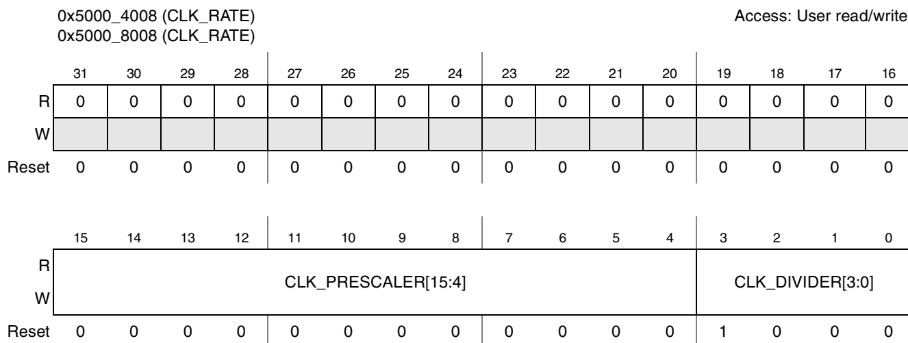
Figure 29-6. SDHC Clock Rate Register
