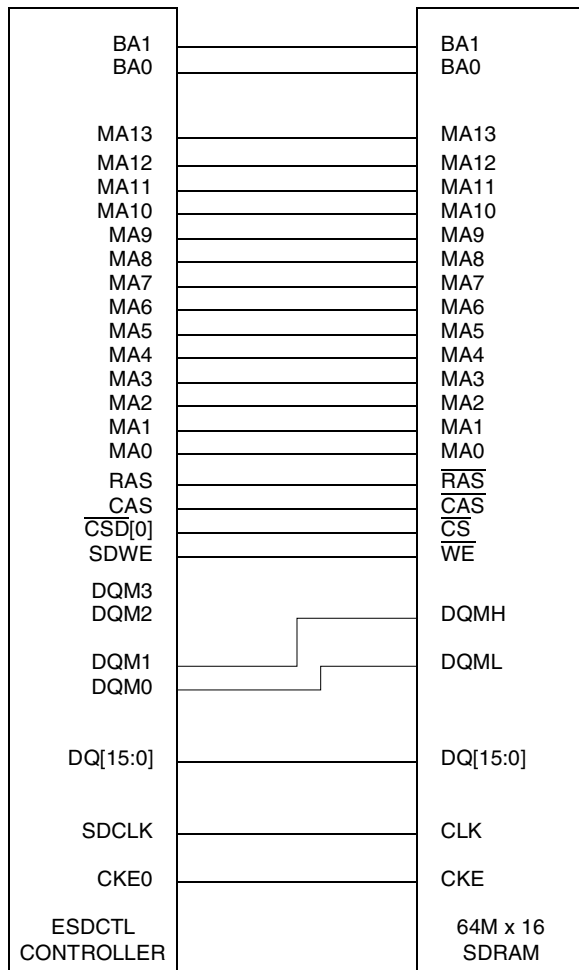
Figure 19-87. Single 1-Gbit (64M x 16) SDRAM Connection Diagram
