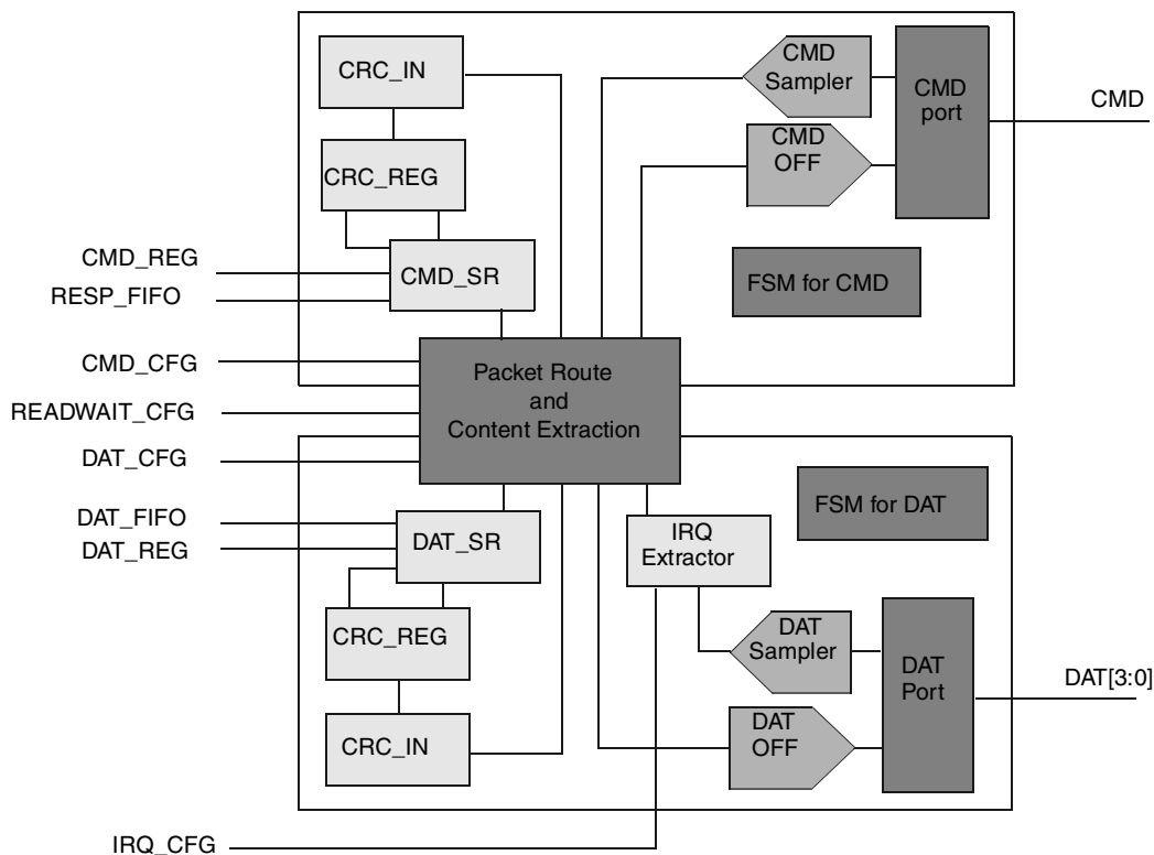
Figure 29-24. Block diagram for Command Interpreter
