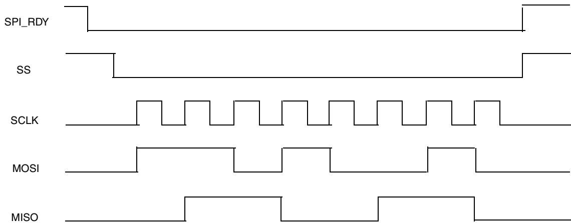
Figure 24-14. Relationship Between a SPI Burst and \overline{\text{SPI\_RDY}}
