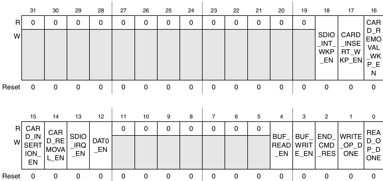
Figure 29-13. SDHC Interrupt Control Register
