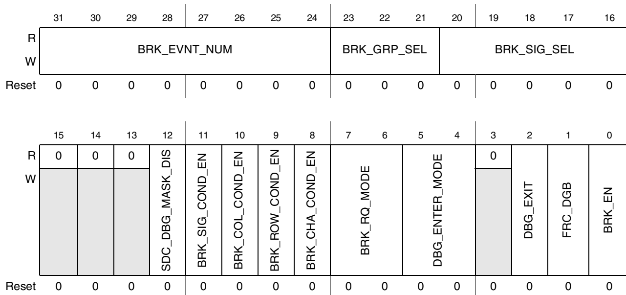
Figure 44-28. IPU Break Control Register 1 (IPU_BRK_CTRL_1)
