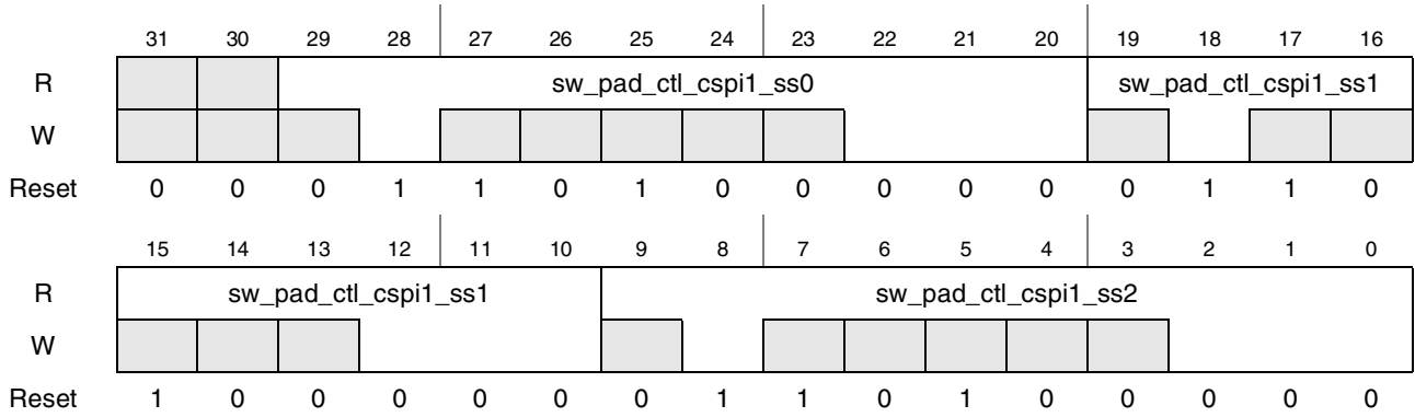
Figure 4-132. Register Description sw_pad_ctl_csipi1_ss0_csipi1_ss1_csipi1_ss2
