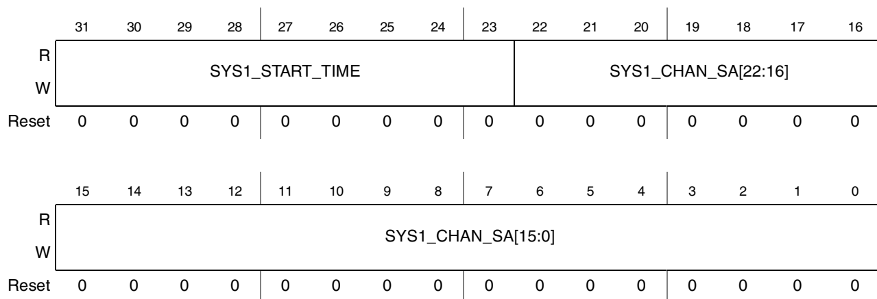
Figure 44-65. ADC System Channel 1 Start Address Register (ADC_SYSCHA1_SA)
