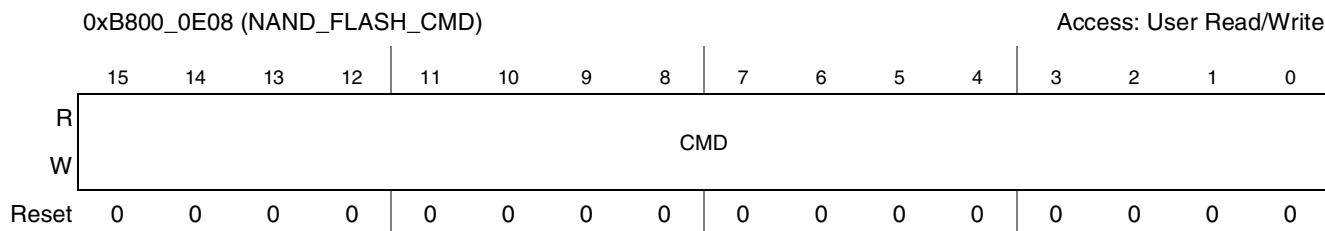
Figure 20-7. NAND_Flash_CMD Register
