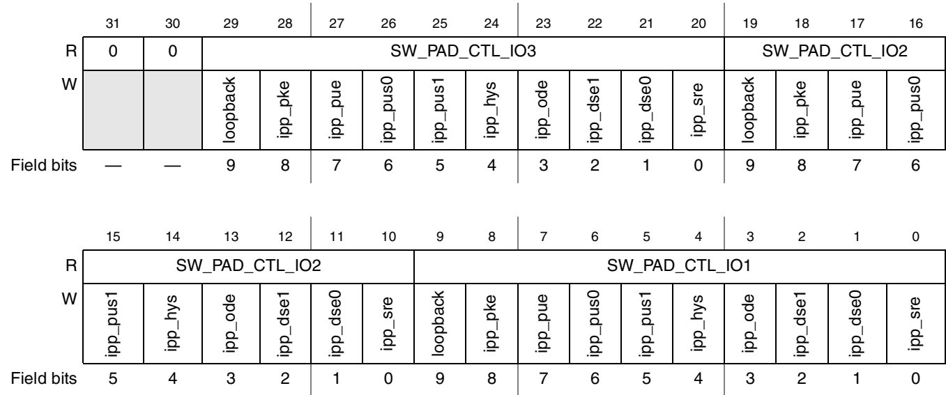
Figure 4-88. SW_PAD_CTL
