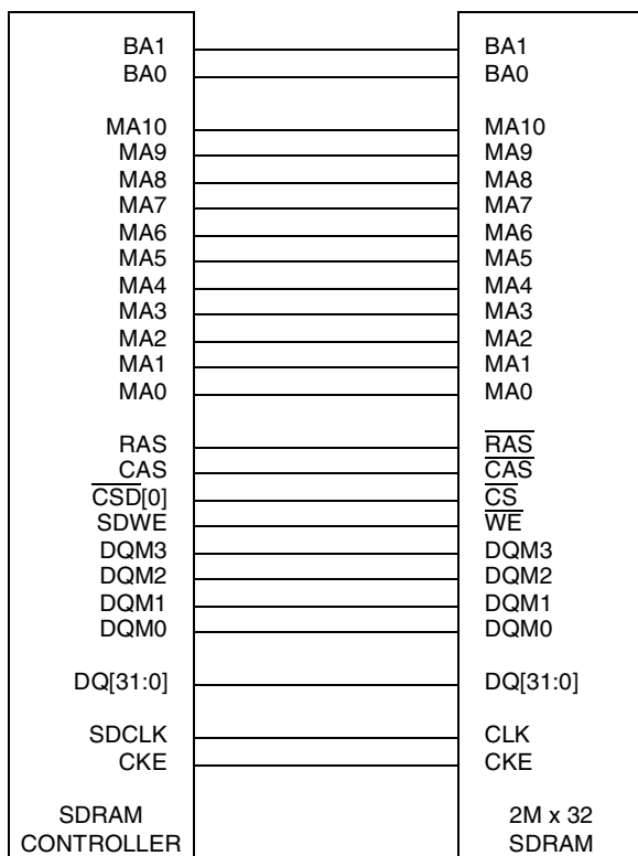
Figure 19-91. Single 64-Mbit (2Mx32) SDRAM Connection Diagram
