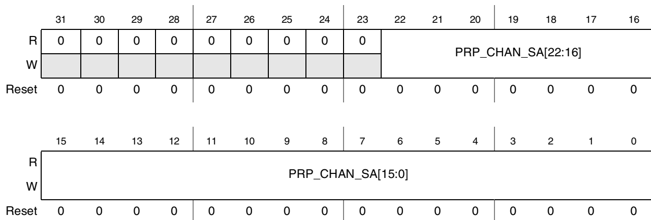
Figure 44-67. ADC Preprocessing Channel Start Address Register (ADC_PRP_CHAN_SA)
