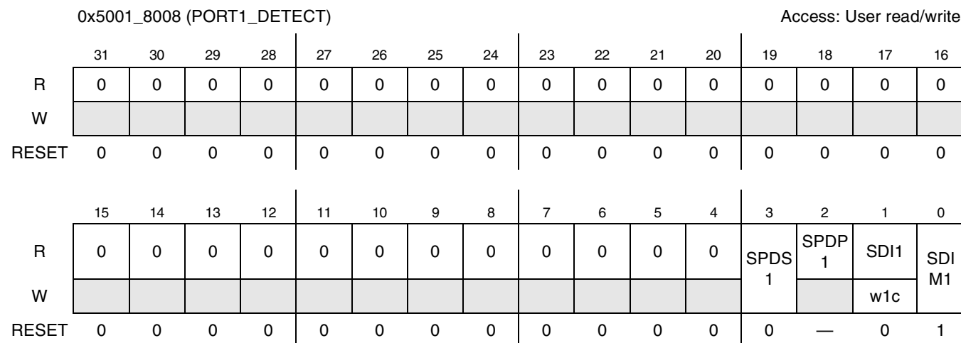
Figure 30-5. SIM Port 1 Detect Register
