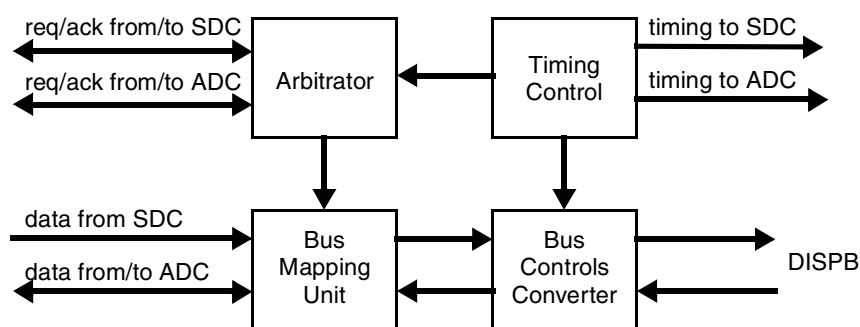
Figure 44-140. DI Block Diagram
