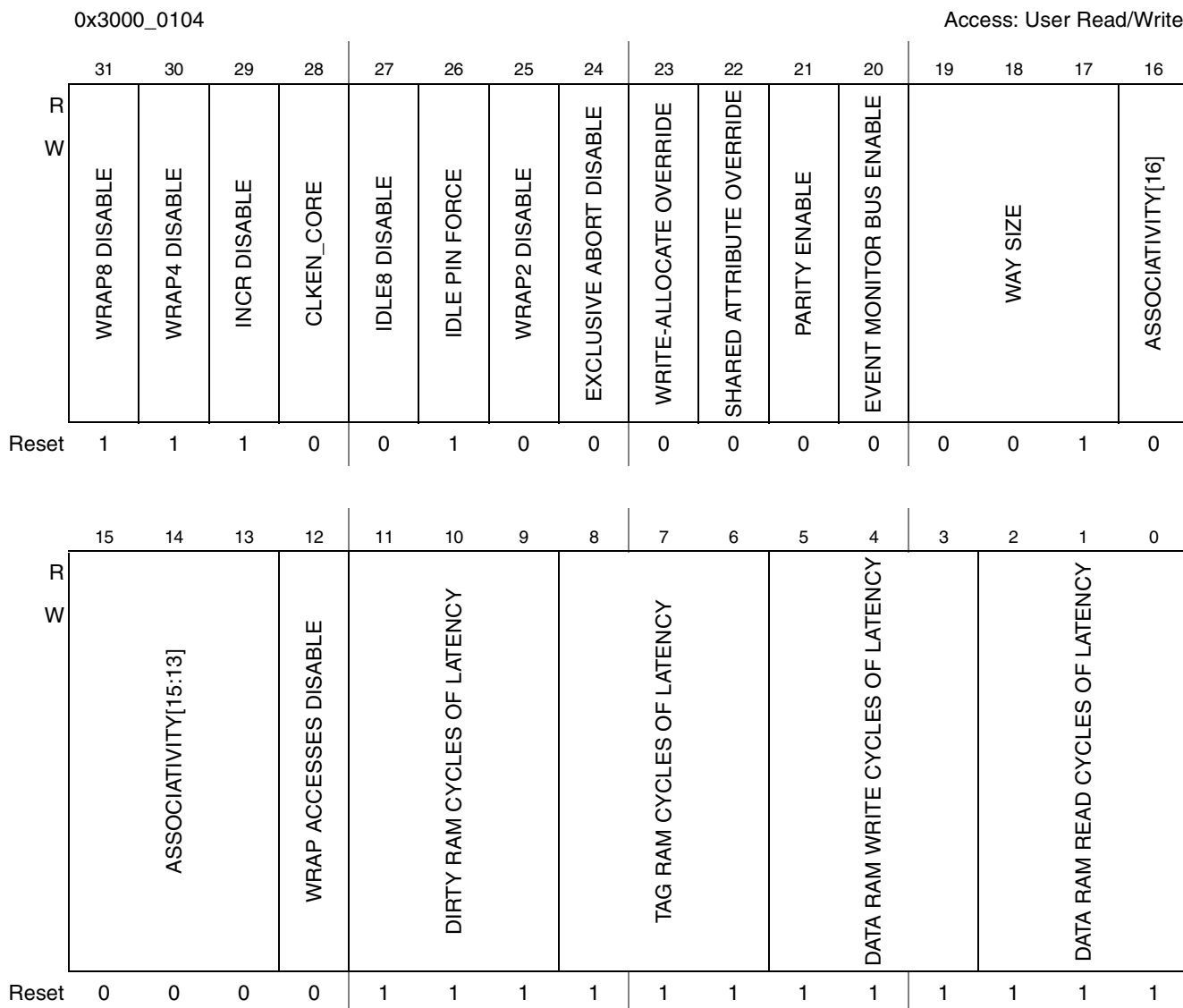
Figure 14-10. L2CC Control Register
