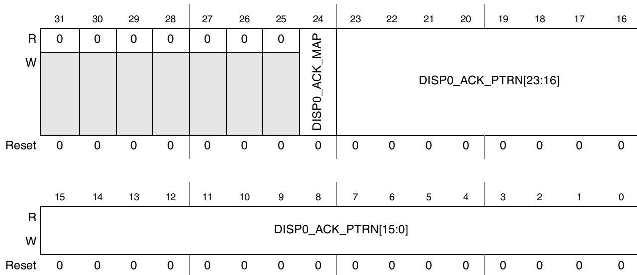
Figure 44-70. ADC Display 0 Read Acknowledge Pattern Register (ADC_DISP0_RD_AP)
