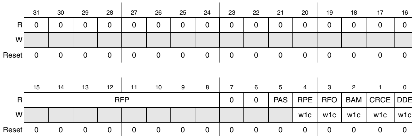
Figure 25-8. FIR Receive Status Register
