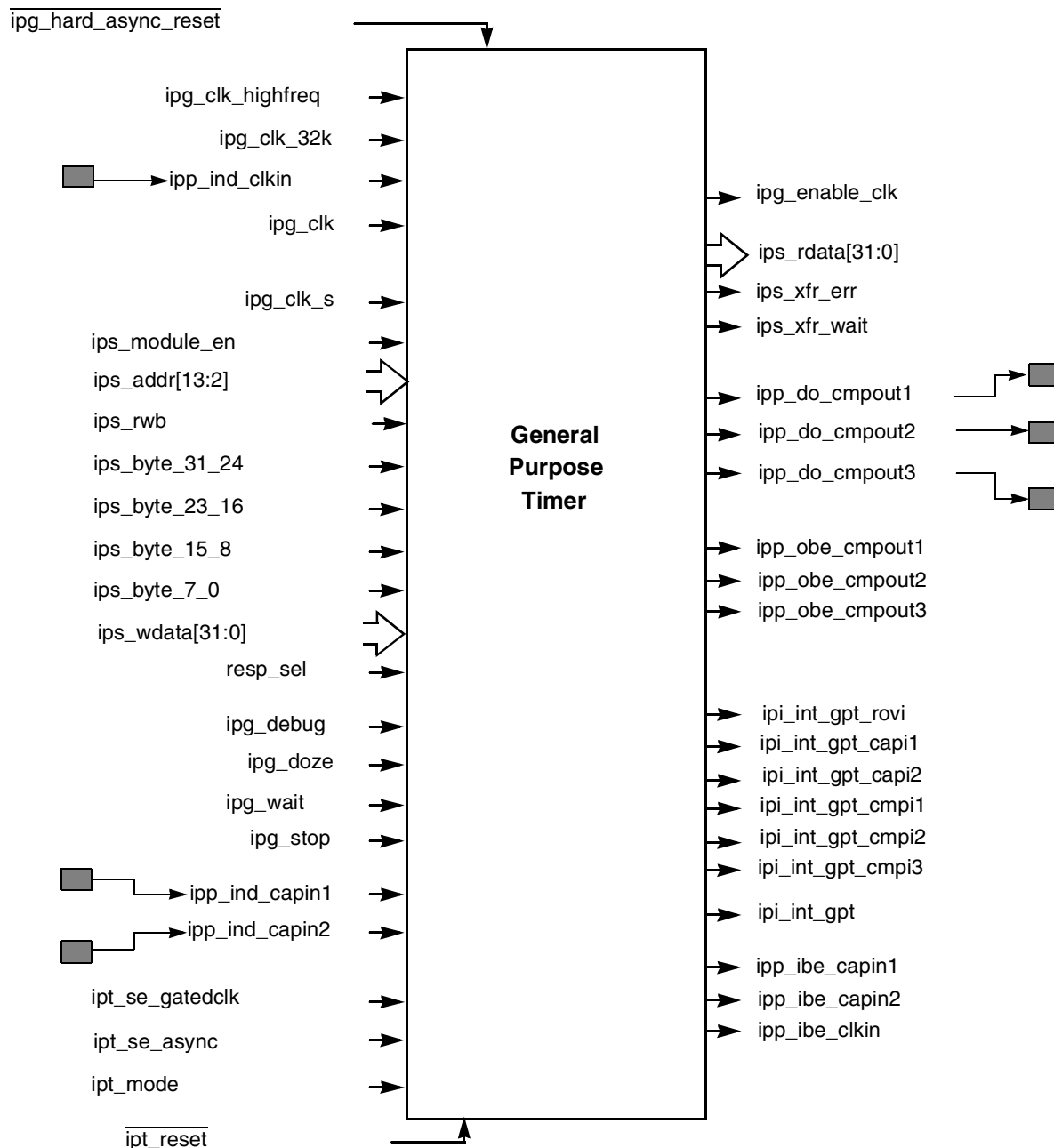
Figure 34-3. GPT Module Signals
