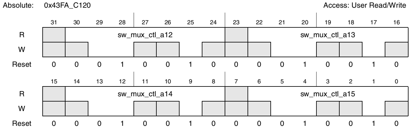
Figure 4-75. Register Description sw_mux_ctl_a12_a13_a14_a15
