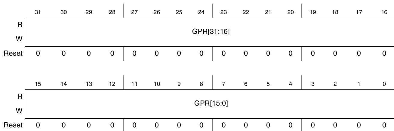
Figure 4-4. General Purpose Register (GPR)
