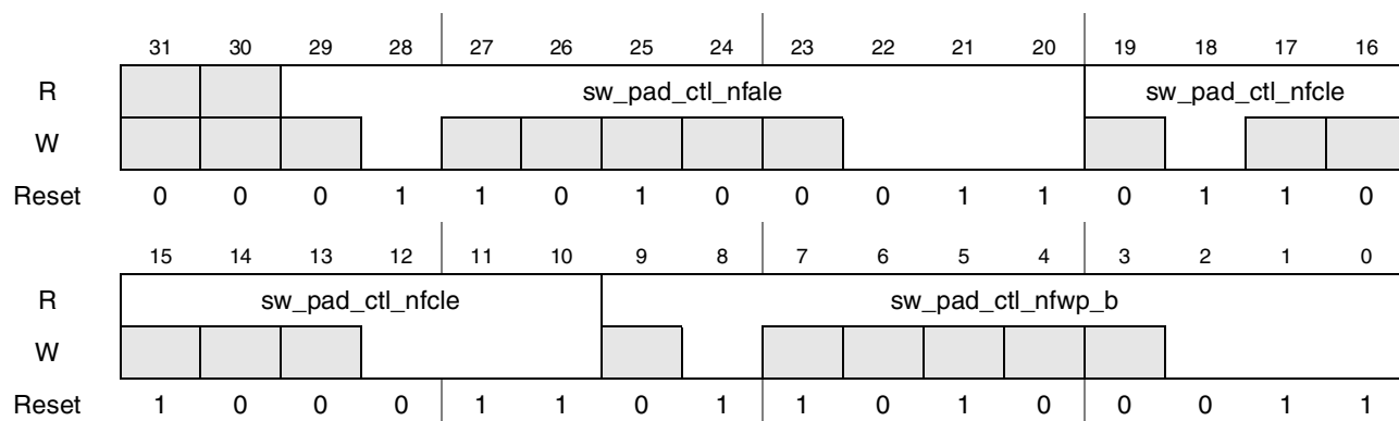
Figure 4-156. Register Description sw_pad_ctl_nfale_nfcle_nfwfp_b
