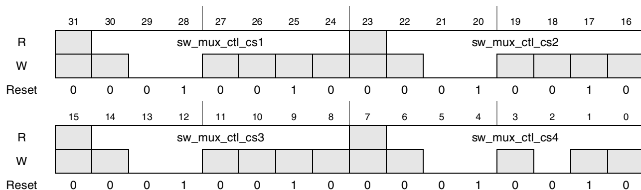
Figure 4-61. Register Description sw_mux_ctl_cs1_cs2_cs3_cs4
