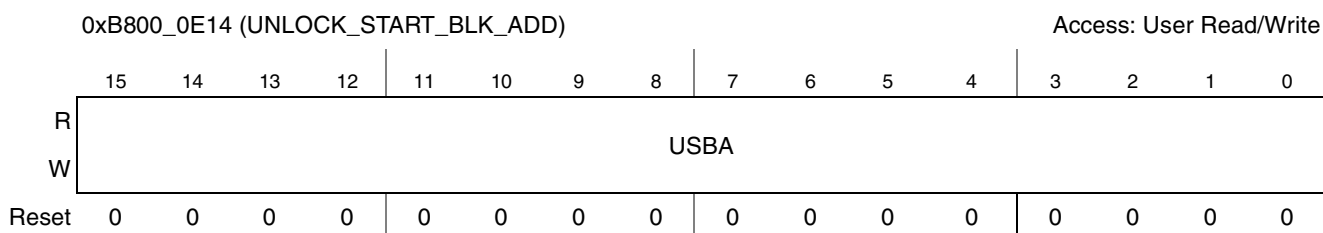
Figure 20-15. Unlock_Start_Blk_Add Register
