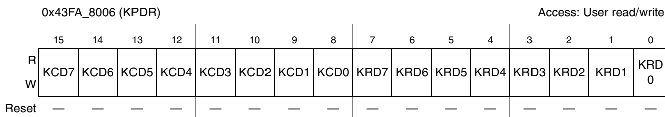
Figure 27-6. KPDR Register
