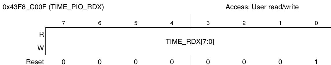
Figure 23-19. TIME_PIO_RDX Register
