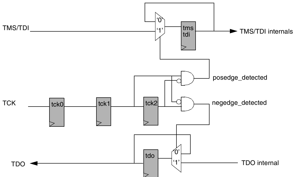
Figure 40-68. OnCE Synchronization Layer
