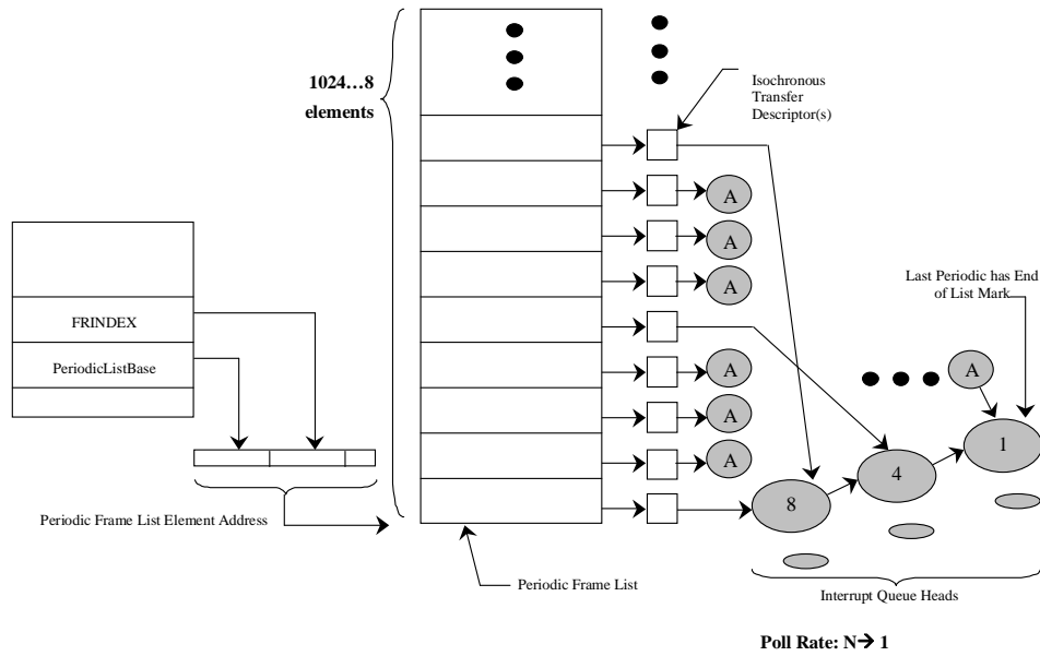
Figure 32-10. Periodic Schedule Organization
