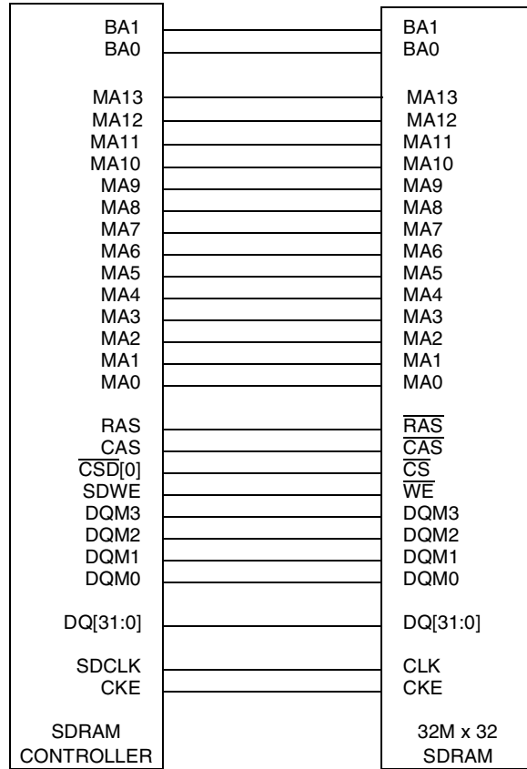
Figure 19-95. Single 1-Gbit (32Mx32) SDRAM Connection Diagram
