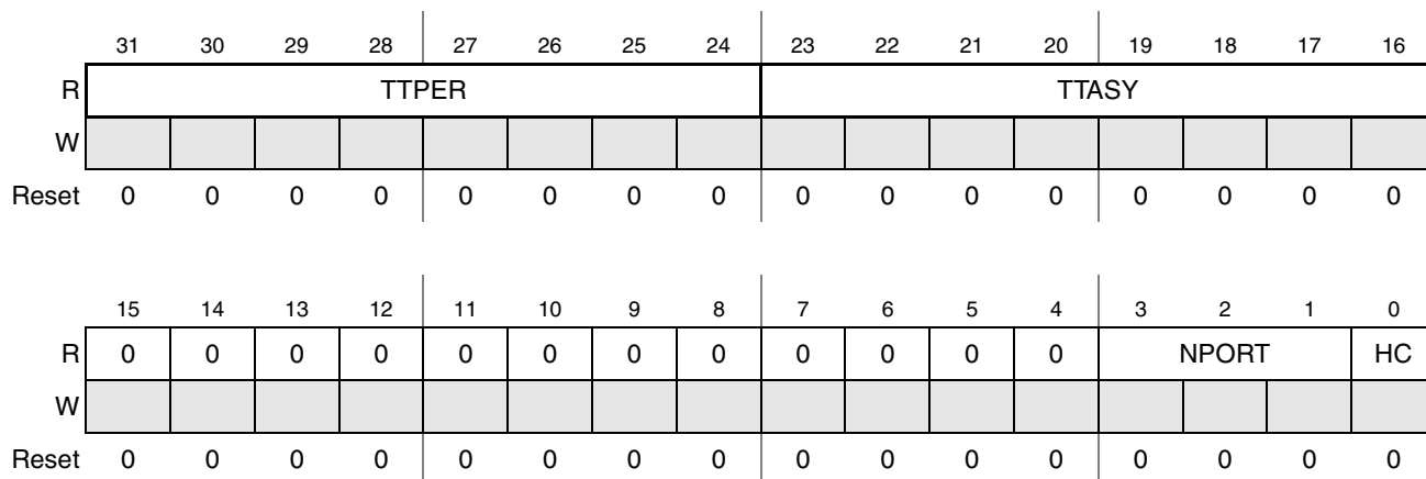
Figure 32-14. HWHOST—Host Hardware Parameters
