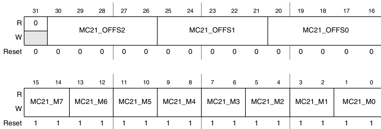
Figure 44-112. DI Display 2 Command Byte 1 Mapping Register (DI_DISP2_CB1_MAP)
