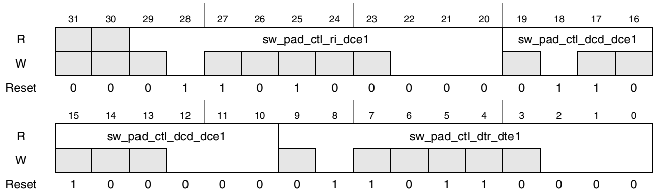
Figure 4-126. Register Description sw_pad_ctl_ri_dce1_dcd_dce1_dtr_dte1
