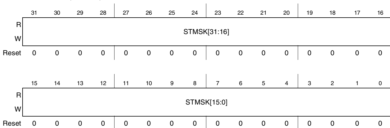
Figure 45-37. SSI Transmit Time Slot Mask Register
