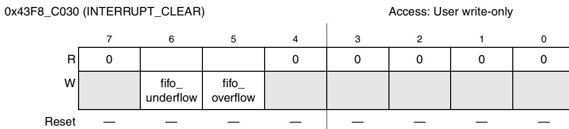
Figure 23-43. INTERRUPT_CLEAR Register
