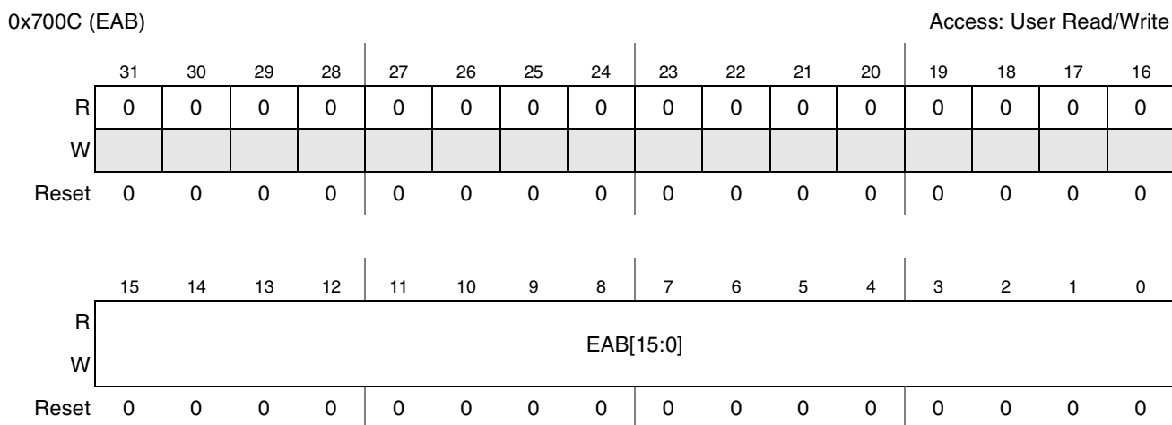
Figure 40-51. OnCE Event Cell Address Register B
