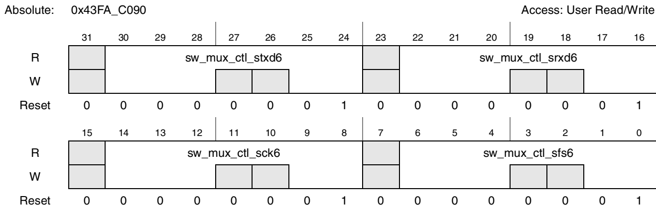
Figure 4-39. Register Description sw_mux_ctl_stxd6_srx6_sck6_sfs6
