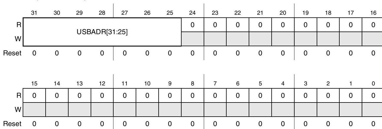
Figure 32-29. DEVICEADDR—Device Controller USB Device Address
