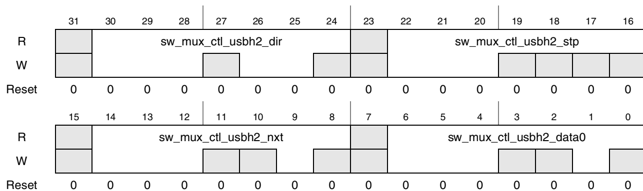
Figure 4-20. Register Description sw_mux_ctl_usbh2_dir_usbh2_stp_usbh2_nxt_usbh2_data0
