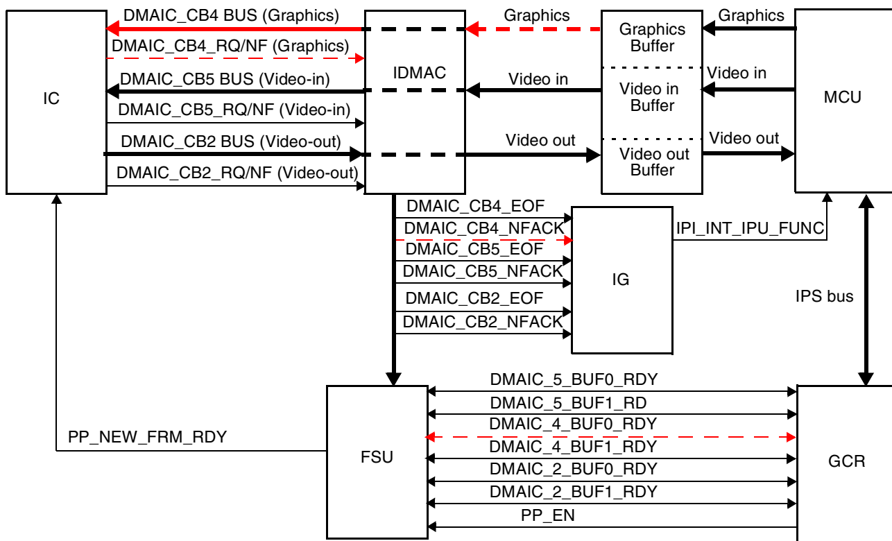
Figure 44-151. Operating Step—First Input Graphics Fetching
