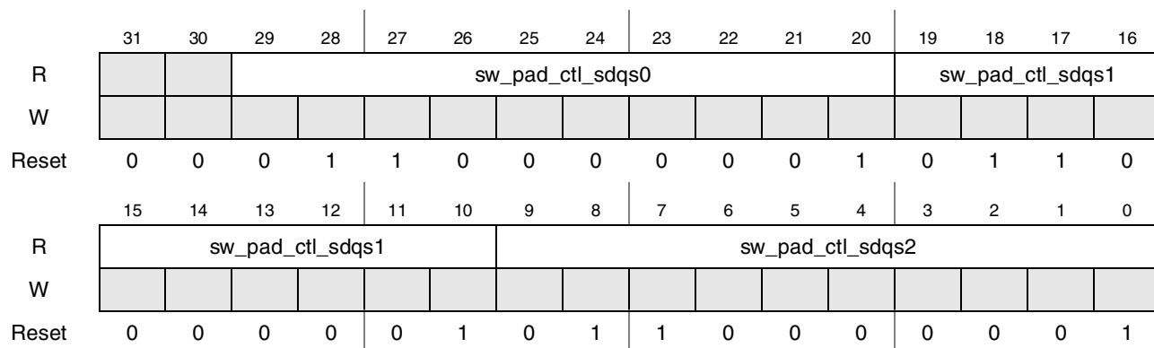
Figure 4-158. Register Description sw_pad_ctl_sdqs0_sdqs1_sdqs2
