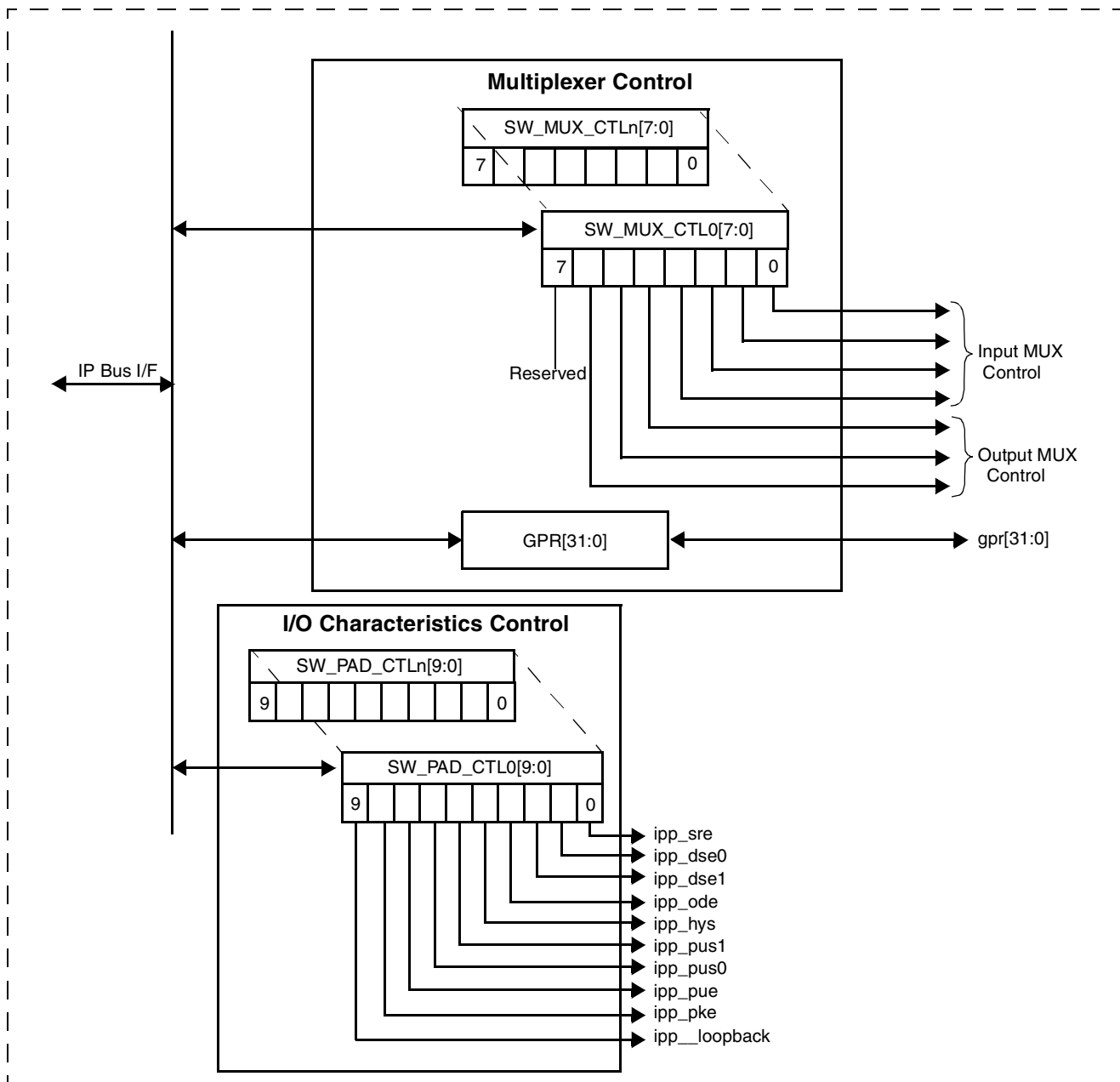
Figure 4-2. IOMUXC Registers
