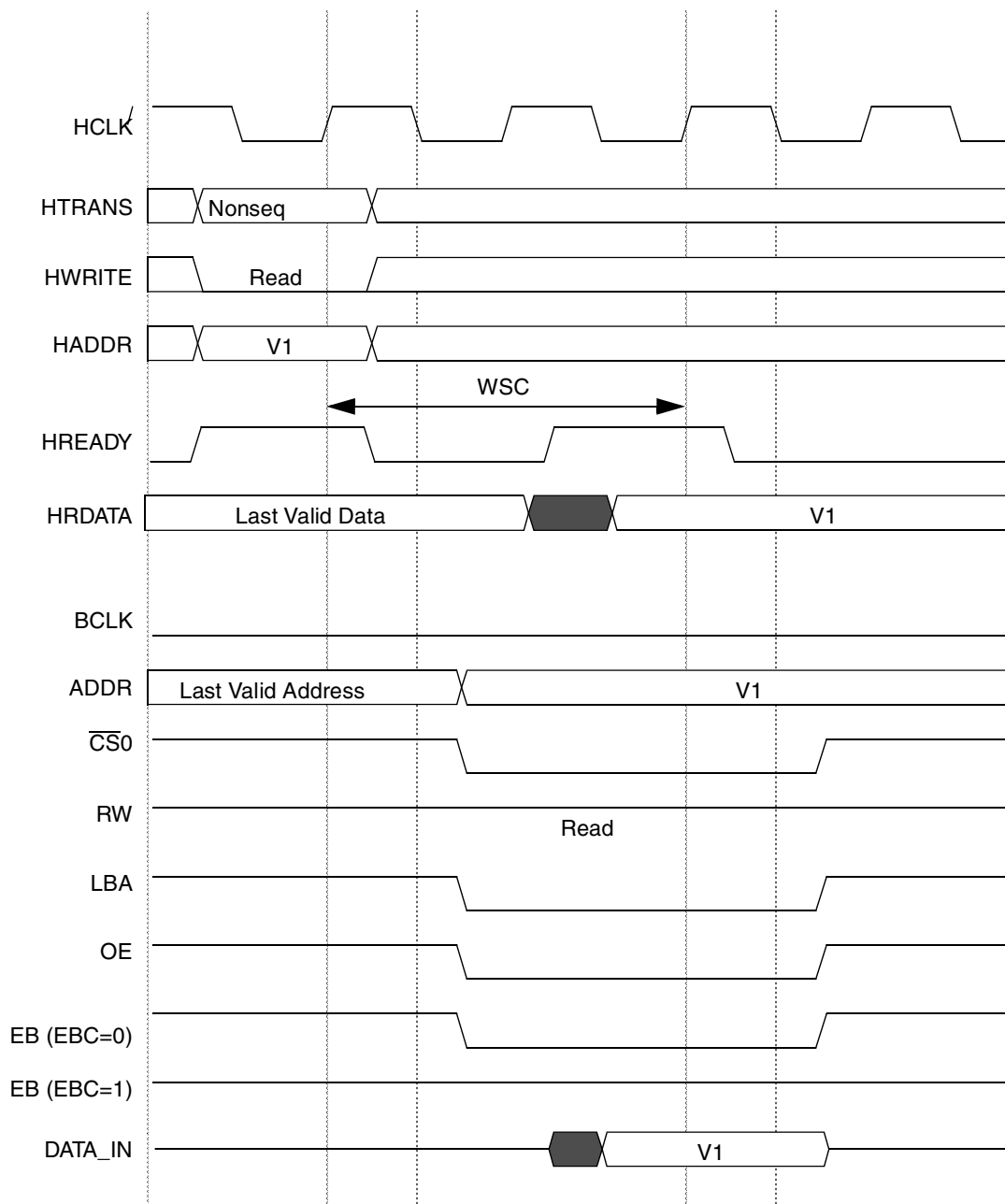
Figure 18-7. Read Access, WSC=1
