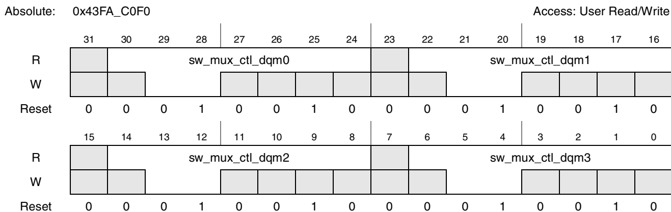
Figure 4-63. Register Description sw_mux_ctl_dqm0_dqm1_dqm2_dqm3
