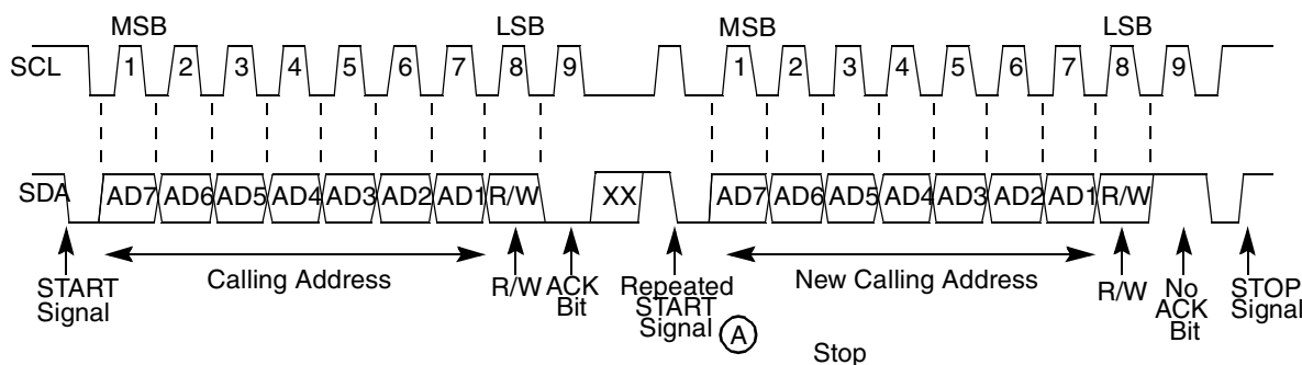
Figure 26-12. Repeated START
