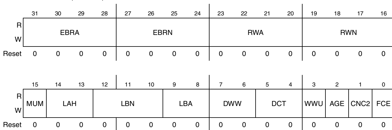
Figure 18-5. Chip Select x Addition Control Register
