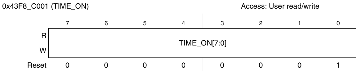
Figure 23-14. TIME_ON Register
