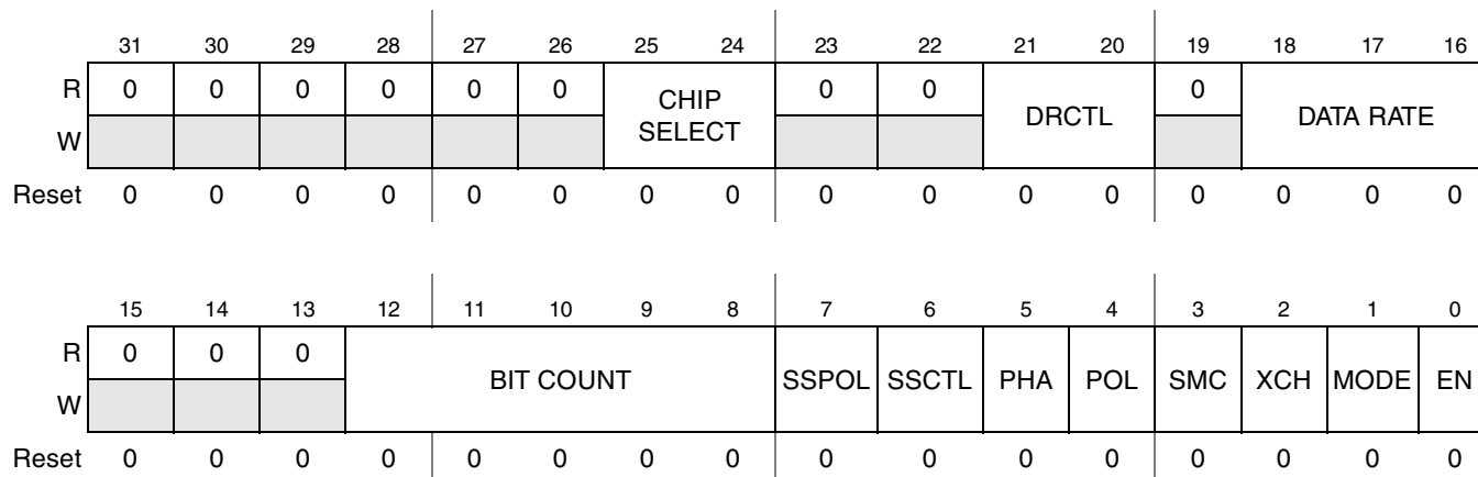
Figure 24-5. CSPI Control Register
