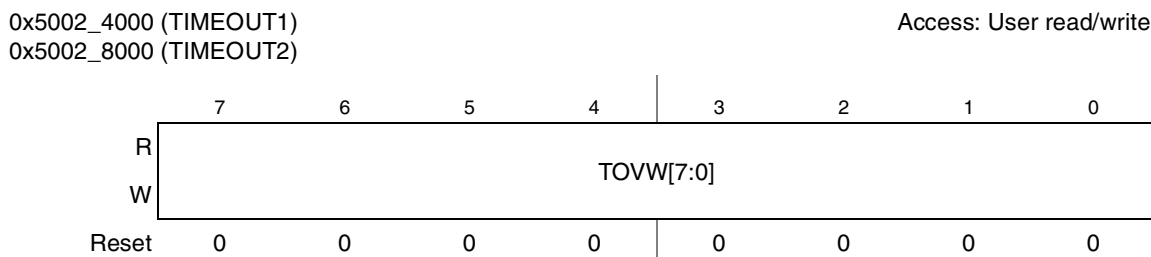
Figure 28-3. Timeout Register
