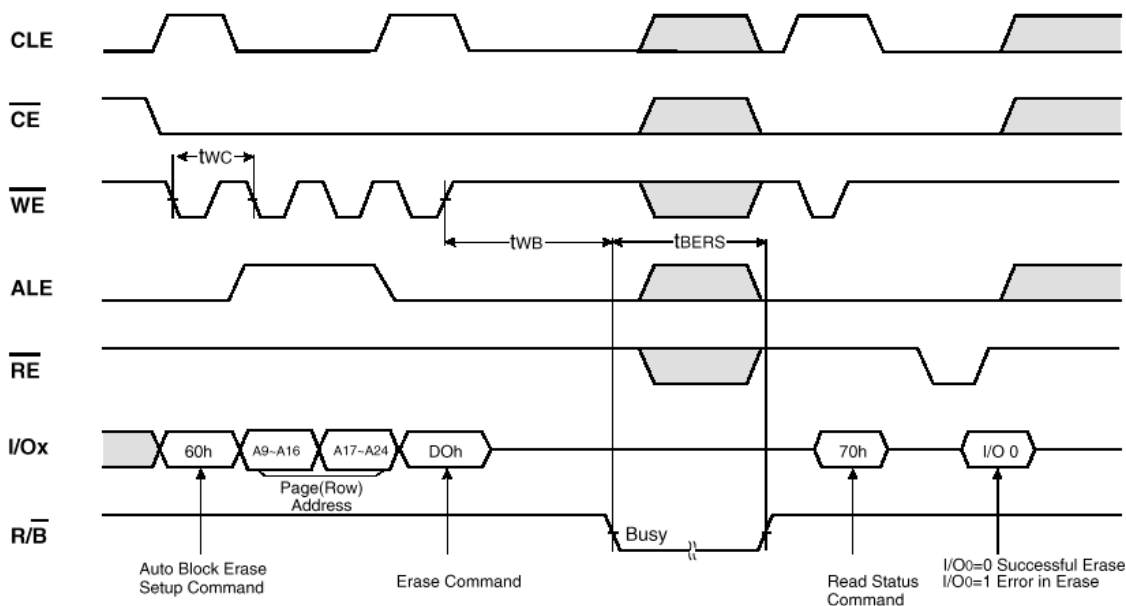
Figure 20-23. Erase Operation
