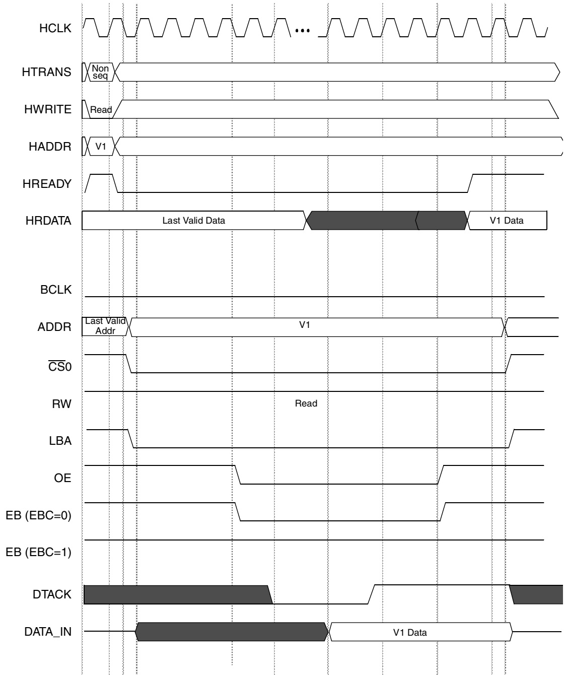
Figure 18-26. Read Access, WSC=3F, OEA=8, OEN=5, EBRA=8, EBRN=5
