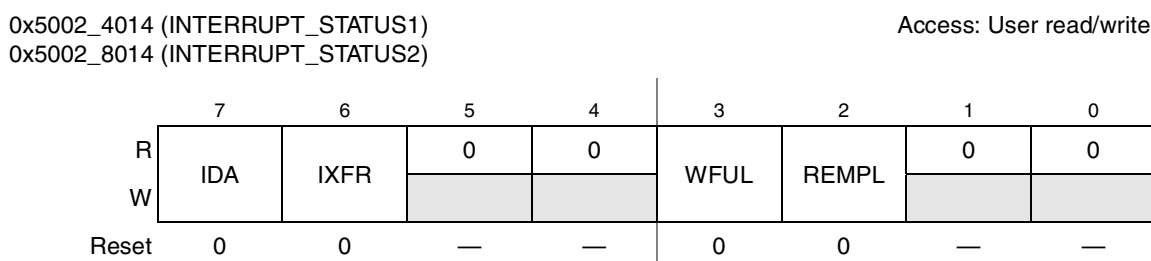
Figure 28-4. Gasket Interrupt Status/Clear Register
