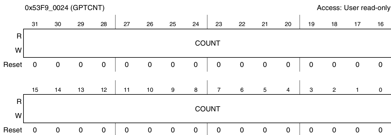
Figure 34-14. GPT Counter Register
