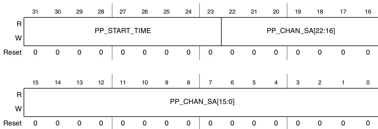
Figure 44-68. ADC Post-Processing Channel Start Address Register (ADC_PPCHAN_SA)
