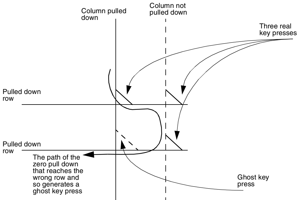
Figure 27-10. Decoding Wrong Three-Key Presses
