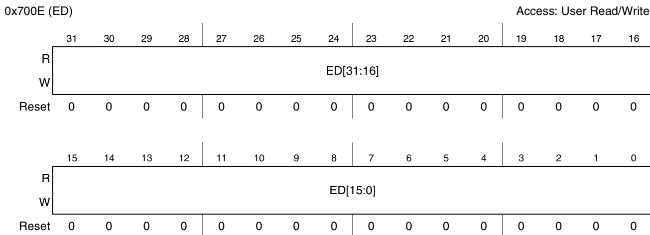
Figure 40-53. OnCE Event Cell Data (ED) Register
