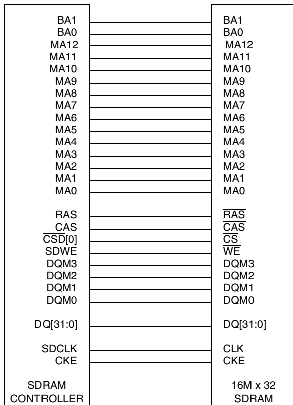
Figure 19-94. Single 512-Mbit (16Mx32) SDRAM Connection Diagram
