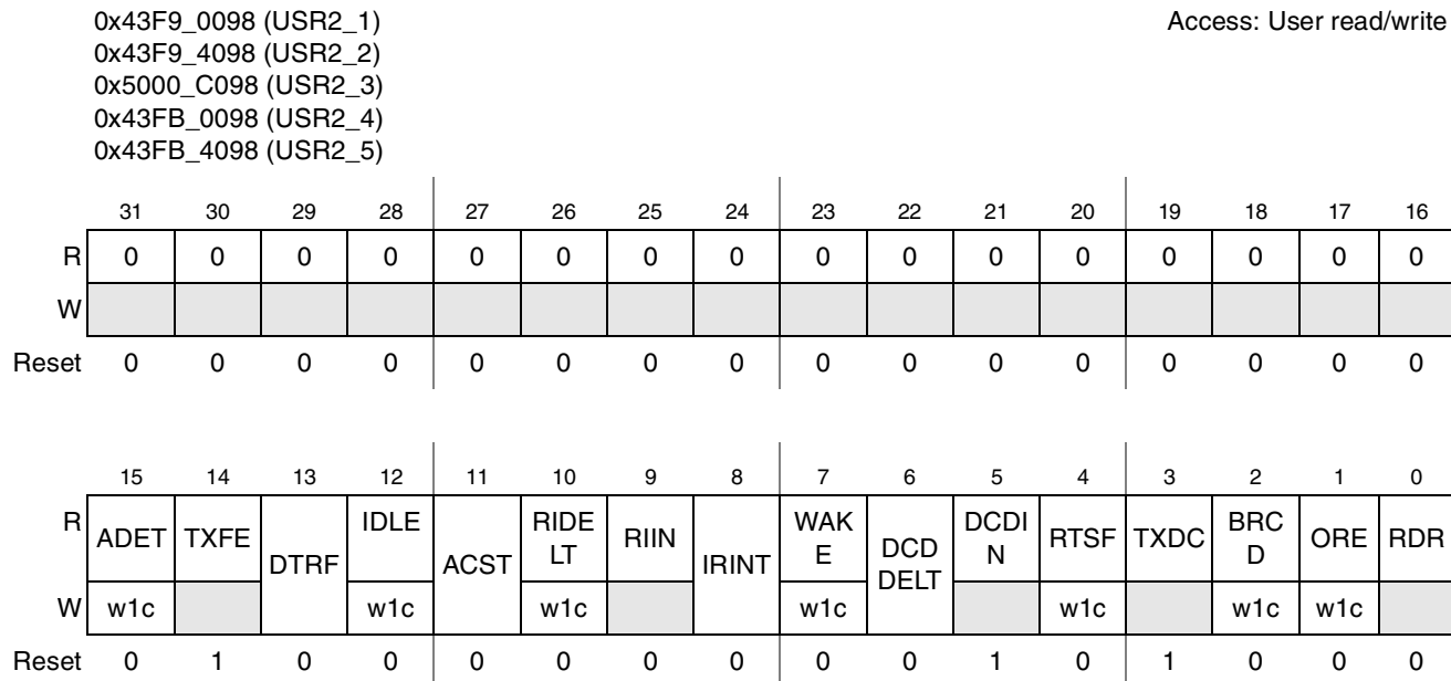
Figure 31-11. UART Status Register 2
