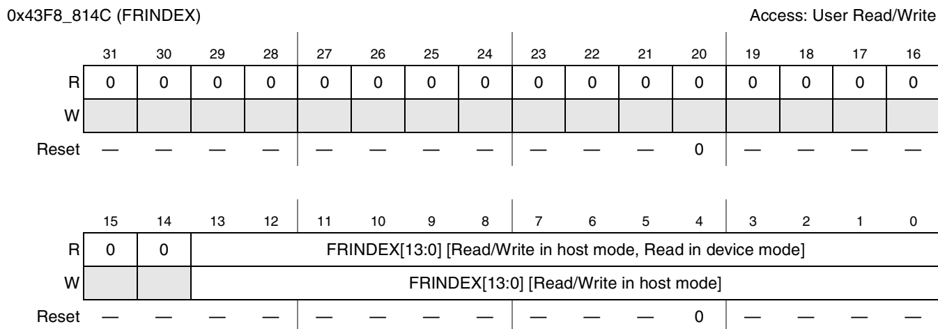
Figure 32-27. FRINDEX—USB Frame Index
