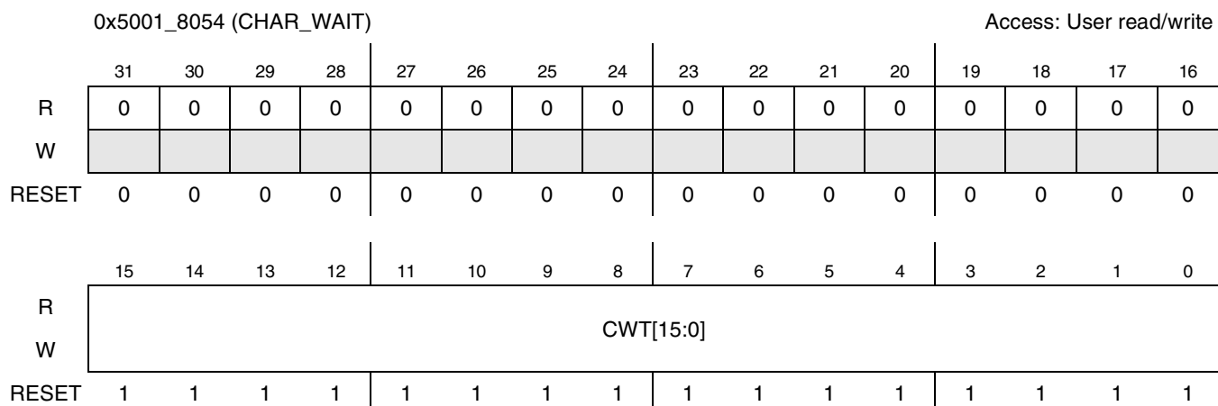
Figure 30-24. SIM Character Wait Time Register
