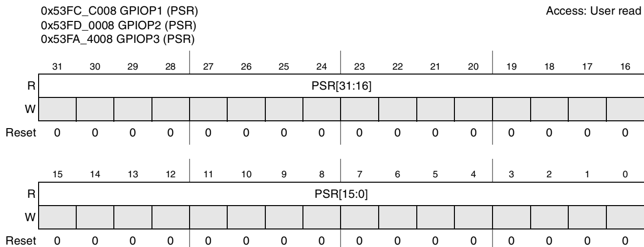
Figure 5-6. GPIO Pad Status Register (PSR)
