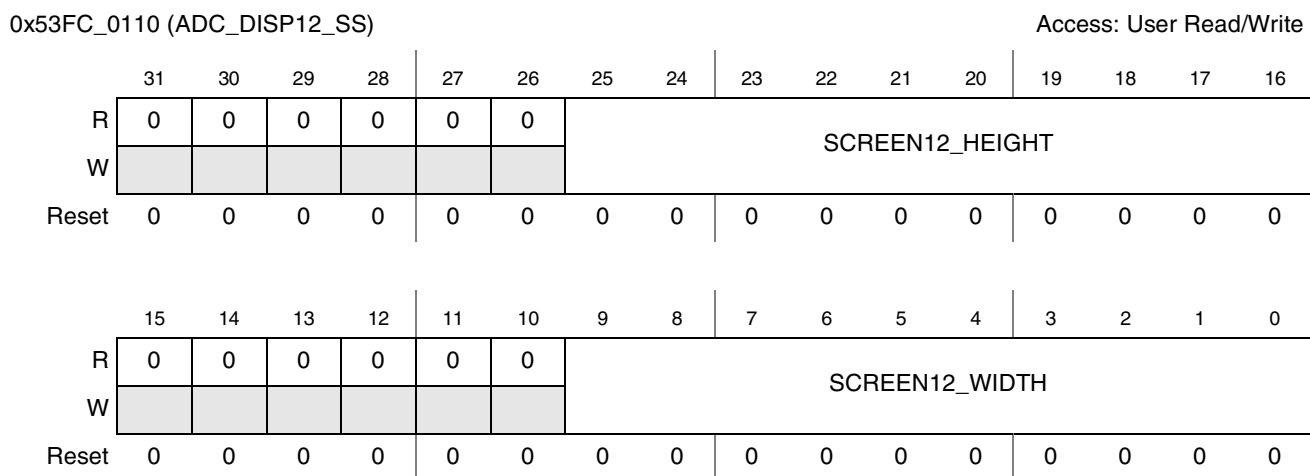
Figure 44-76. ADC Displays 1 or 2 Screen Size Register (ADC_DISP12_SS)
