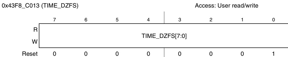
Figure 23-32. TIME_DZFS Register
