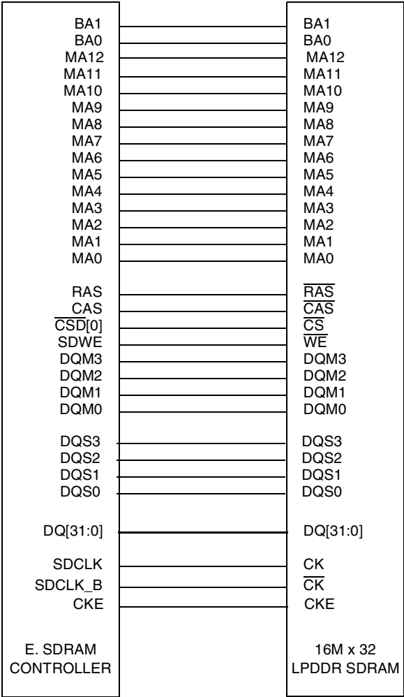
Figure 19-97. Single 512-Mbit (16Mx32) LPDDR SDRAM Connection Diagram
