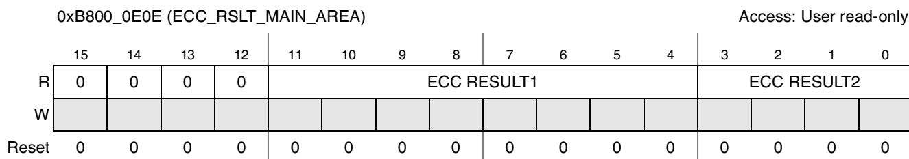
Figure 20-11. ECC_RSLT_MAIN_AREA Register
