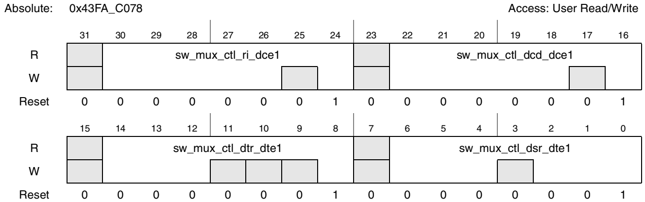
Figure 4-33. Register Description sw_mux_ctl_ri_dce1_dcd_dce1_dtr_dte1_dsr_dte1
