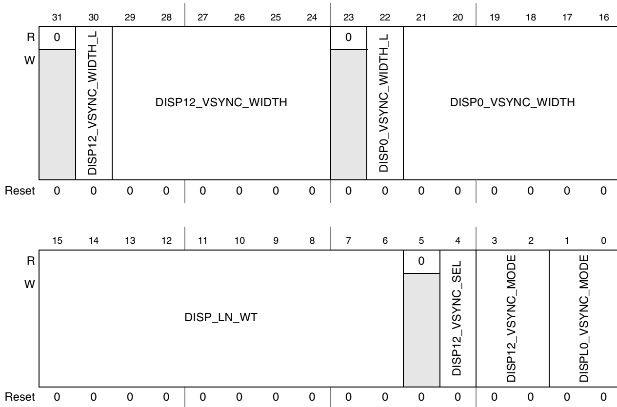
Figure 44-80. ADC Displays Vertical Synchronization Register (ADC_DISP_VSYNC)
