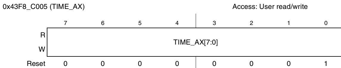
Figure 23-18. TIME_AX Register
