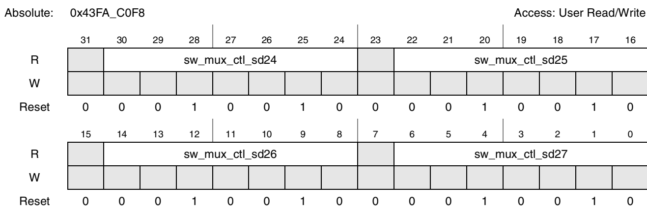
Figure 4-65. Register Description sw_mux_ctl_sd24_sd25_sd26_sd27
