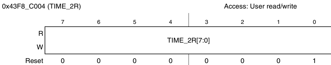
Figure 23-17. TIME_2R Register
