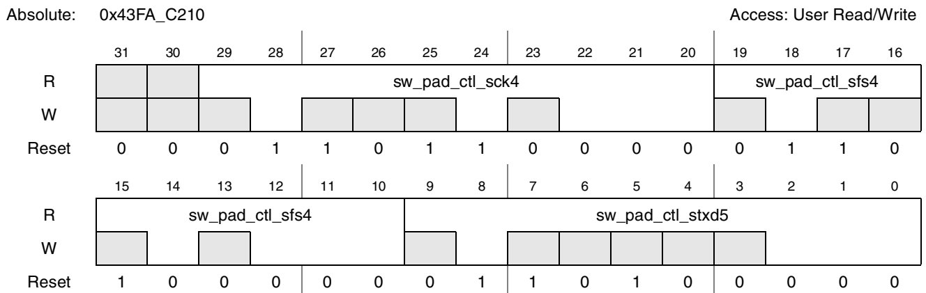
Figure 4-136. Register Description sw_pad_ctl_sck4_sfs4_stxd5
