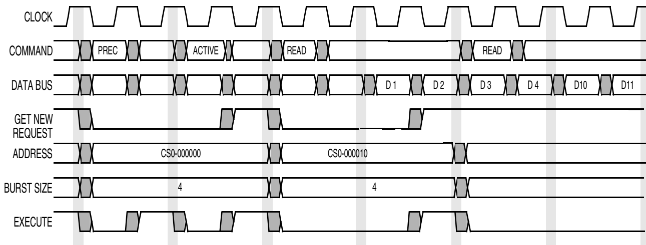
Figure 19-31. SDR Simple Read after Read Latency Hiding Timing Diagram
