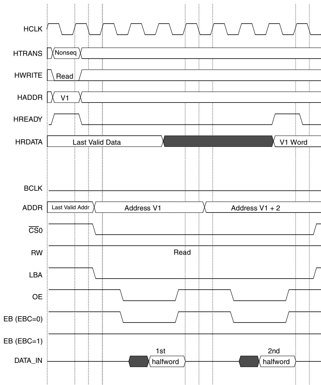
Figure 18-21. Read Access, WSC=3, OEA=2, OEN=2, EBRA=2, EBRN=2
