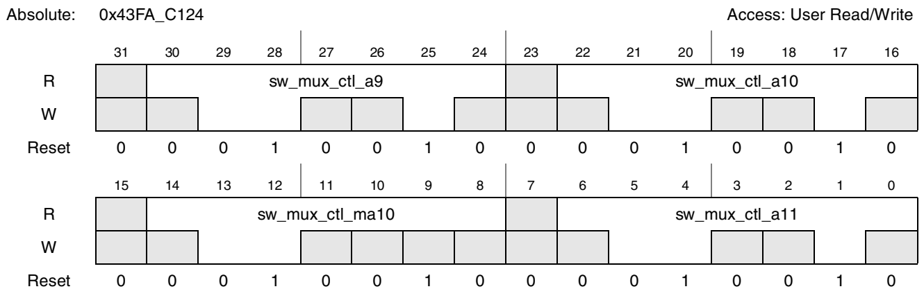
Figure 4-76. Register Description sw_mux_ctl_a9_a10_ma10_a11
