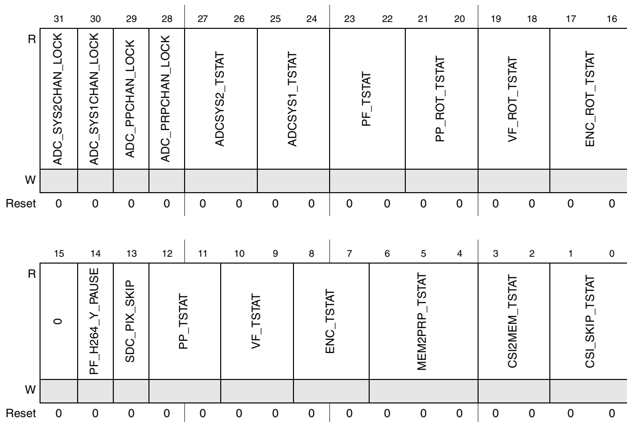
Figure 44-15. IPU Tasks Status Register (IPU_TASKS_STAT)
