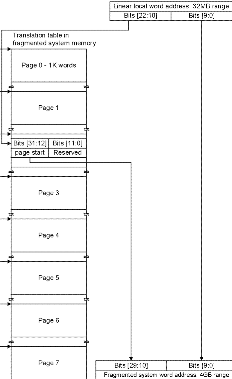
Figure 46-3. MMU Address Translation
