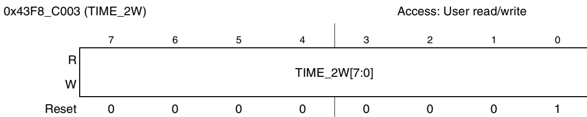
Figure 23-16. TIME_2W Register
