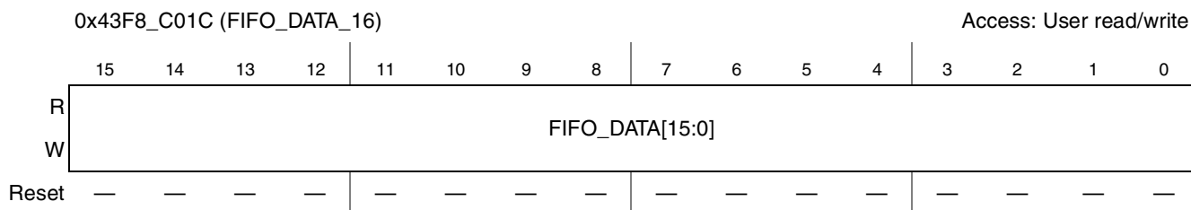
Figure 23-37. FIFO_DATA Register In 16-bit Mode
