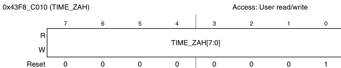
Figure 23-29. TIME_ZAH Register
