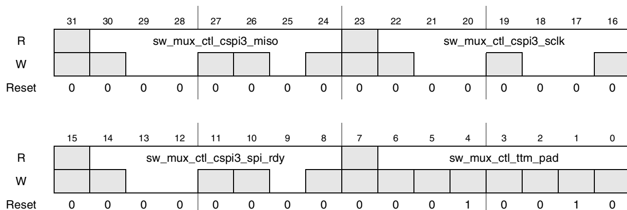
Figure 4-6. Register Description sw_mux_ctl_csipi3_miso_csipi3_sclk_csipi3_spi_rdy_ttm_pad
