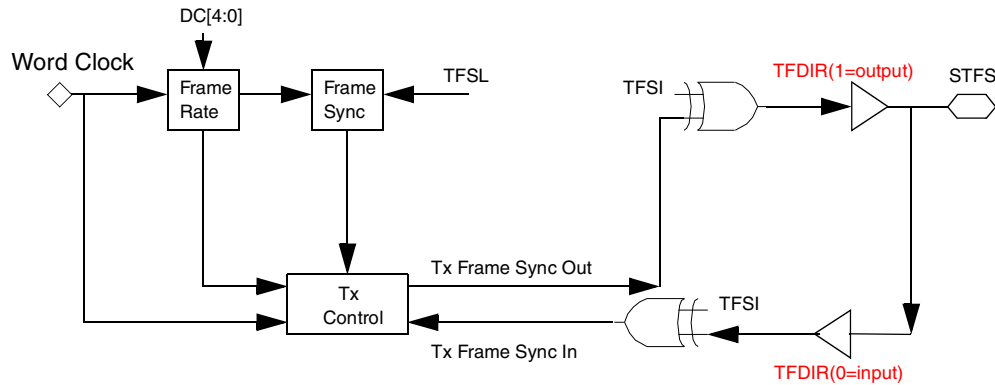
Figure 45-41. SSI Transmit Frame Sync Generator Block Diagram
