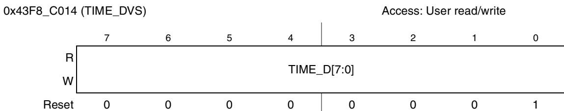
Figure 23-33. TIME_DVS Register
