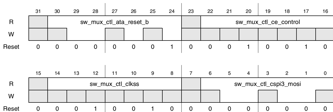
Figure 4-7. Register Description sw_mux_ctl_ata_reset_b_ce_control_clkss_csipi3_mosi
