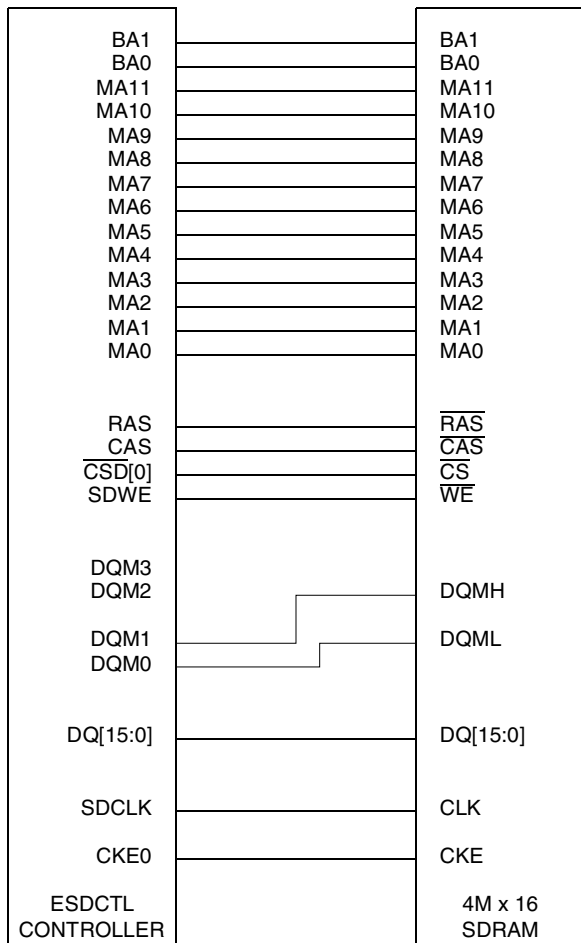
Figure 19-83. Single 64 Mbit (4M x 16) SDRAM Connection Diagram
