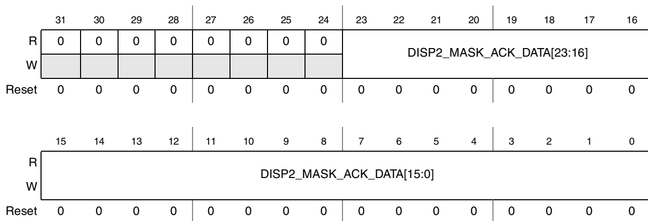
Figure 44-79. ADC Display 2 Read Mask Register (ADC_DISP2_RDM)
