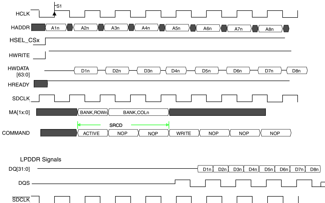
Figure 19-60. AHB 32-Bit Write to LPDDR: Off-Page Burst Write Timing Diagram (32-Bit Memory)
