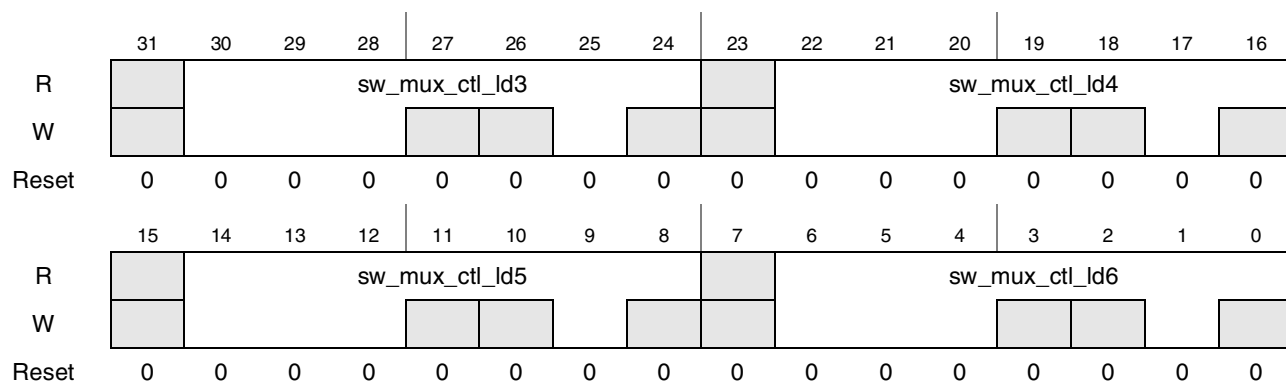
Figure 4-18. Register Description sw_mux_ctl_ld3_ld4_ld5_ld6
