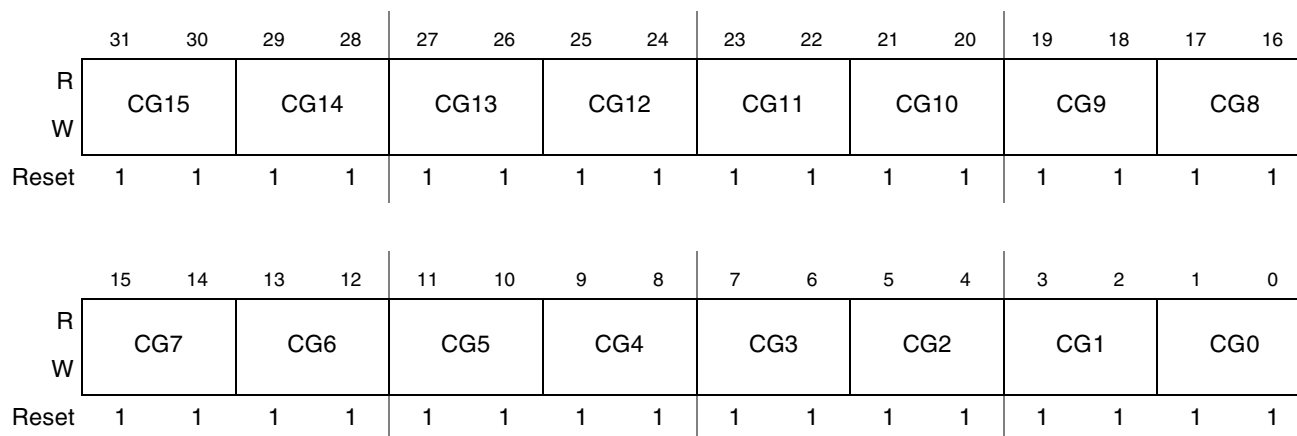
Figure 3-11. Clock Gating Registers (CGR0–CGR2)
