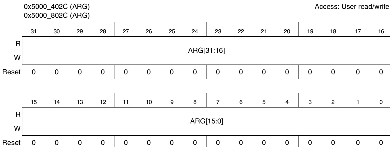
Figure 29-15. SDHC Command Argument Register
