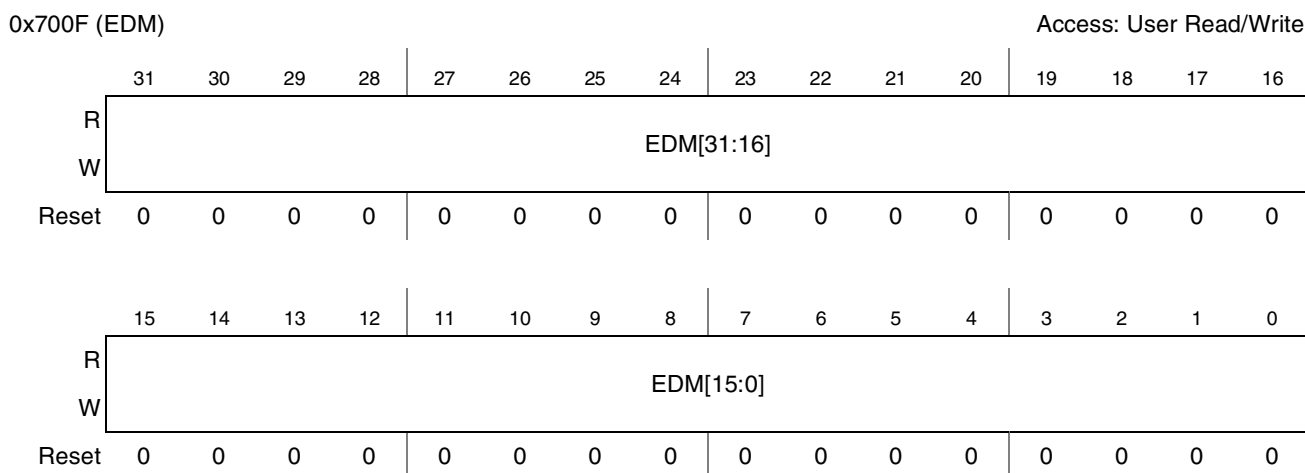
Figure 40-54. OnCE Event Cell Data Mask (EDM) Register
