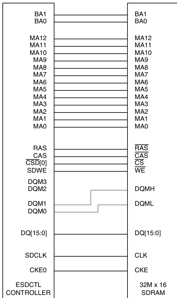
Figure 19-86. Single 512 Mbit (32M x 16) SDRAM Connection Diagram
