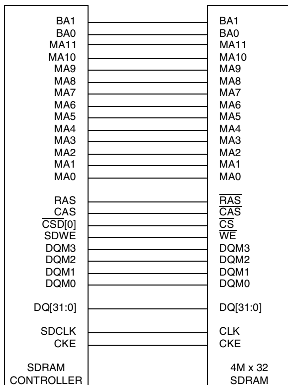
Figure 19-92. Single 128-Mbit (4Mx32) SDRAM Connection Diagram
