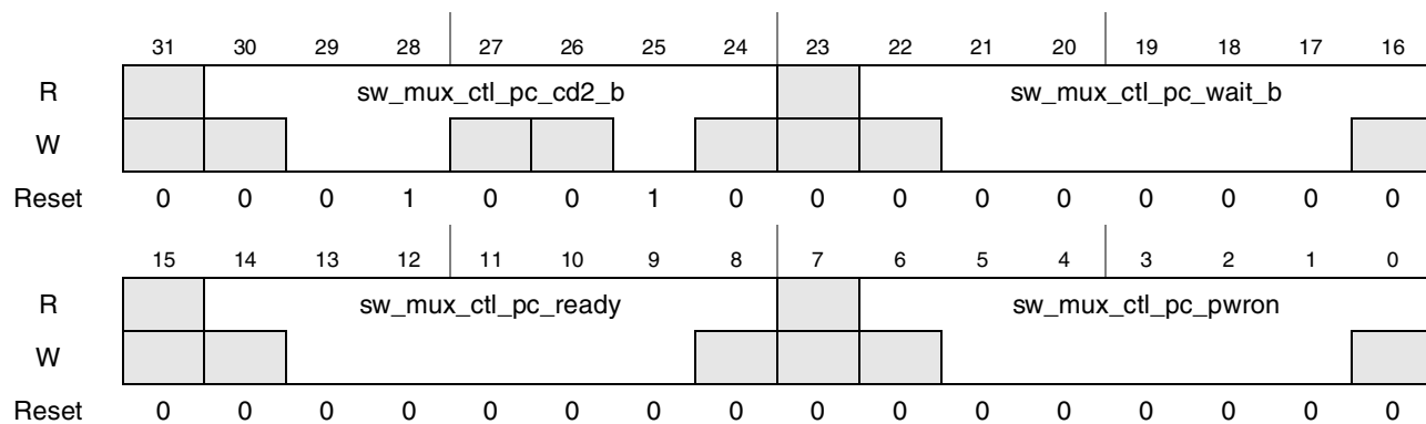
Figure 4-50. Register Description sw_mux_ctl_pc_cd2_b_pc_wait_b_pc_ready_pc_pwrn
