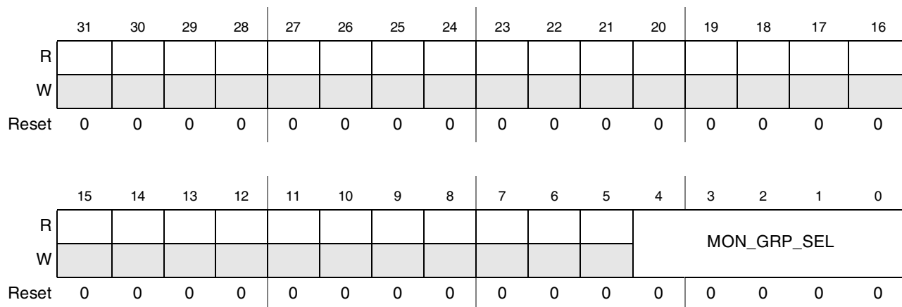
Figure 44-31. IPU Diagnostic Bus Control Register (IPU_DIAGB_CTRL)
