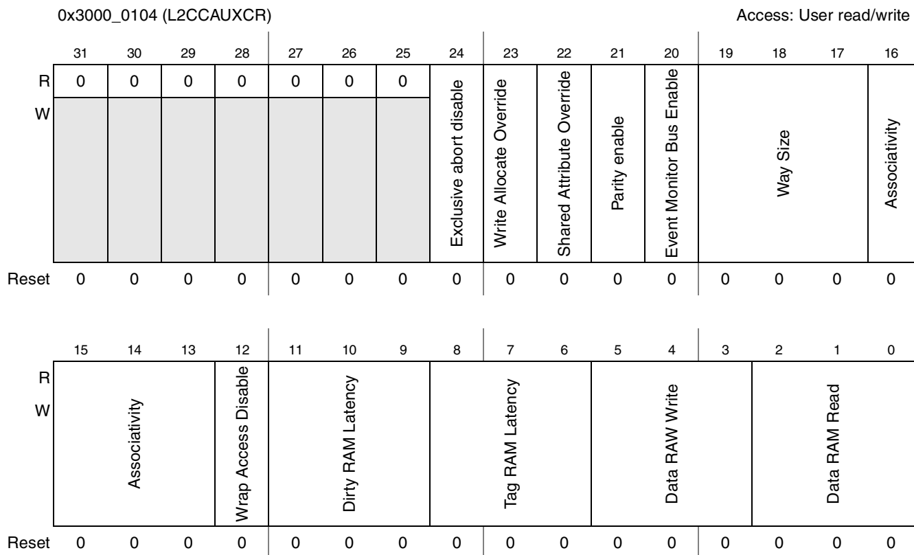
Figure 14-18. L2CC Auxiliary Control Register 2 (L2CCAUXCR)
