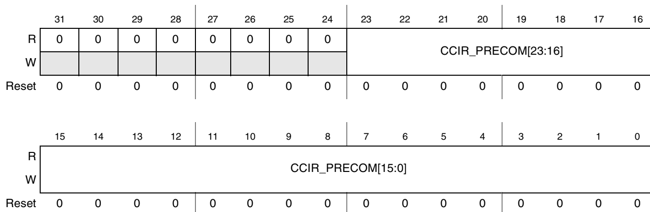
Figure 44-39. CSI CCIR Code Register 3 (CSI_CCIR_CODE_3)
