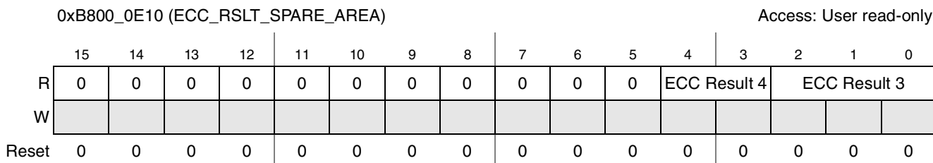
Figure 20-12. ECC_Rslt_Spare_Area Register
