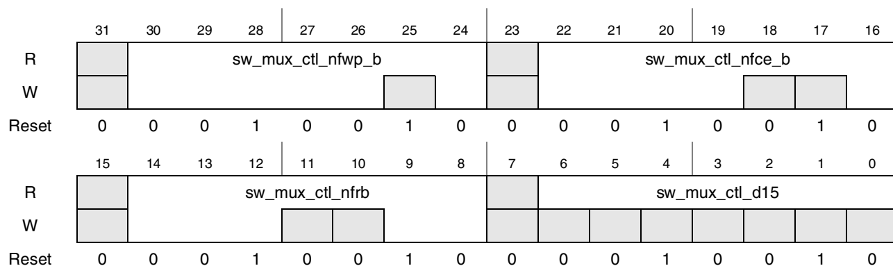
Figure 4-55. Register Description sw_mux_ctl_nfwf_b_nfce_b_nfrb_d15
