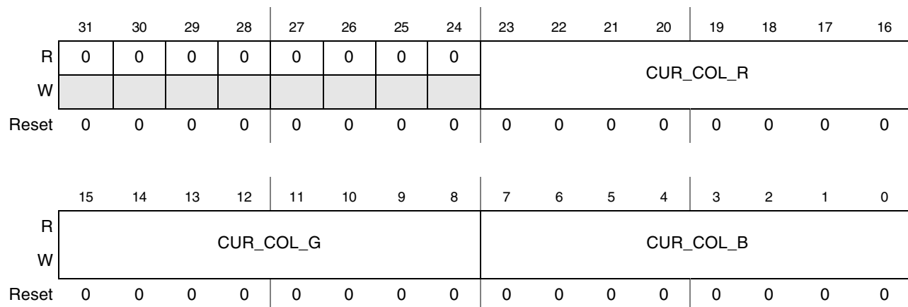
Figure 44-59. SDC Color Cursor Mapping Register (SDC_CUR_MAP)
