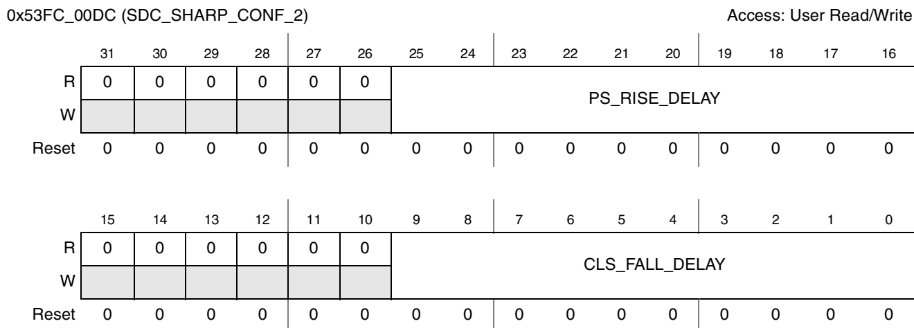
Figure 44-63. SDC Sharp Configuration Register 2 (SDC_SHARP_CONF_2)
