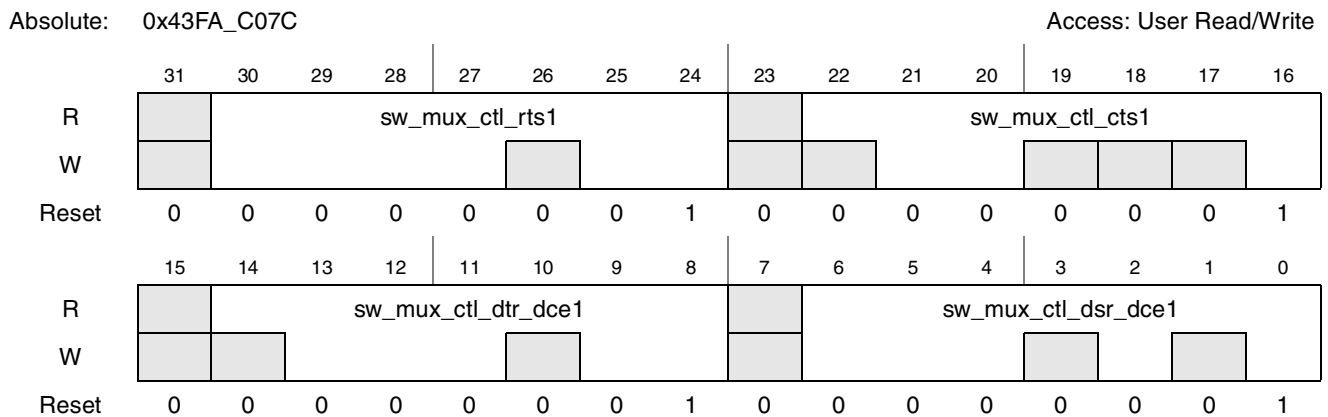
Figure 4-34. Register Description sw_mux_ctl_rts1_cts1_dtr_dce1_dsr_dce1
