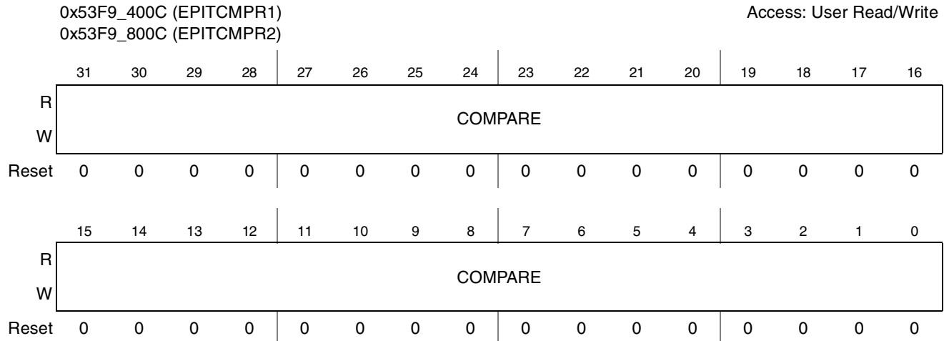
Figure 33-7. EPITC Compare Register (EPITCCMPR)
