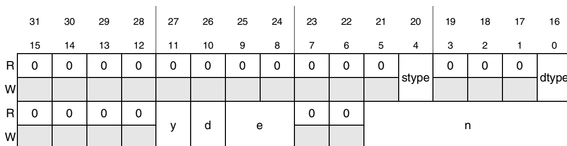
Figure 40-60. MS Structure
