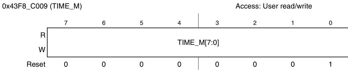
Figure 23-22. TIME_M Register
