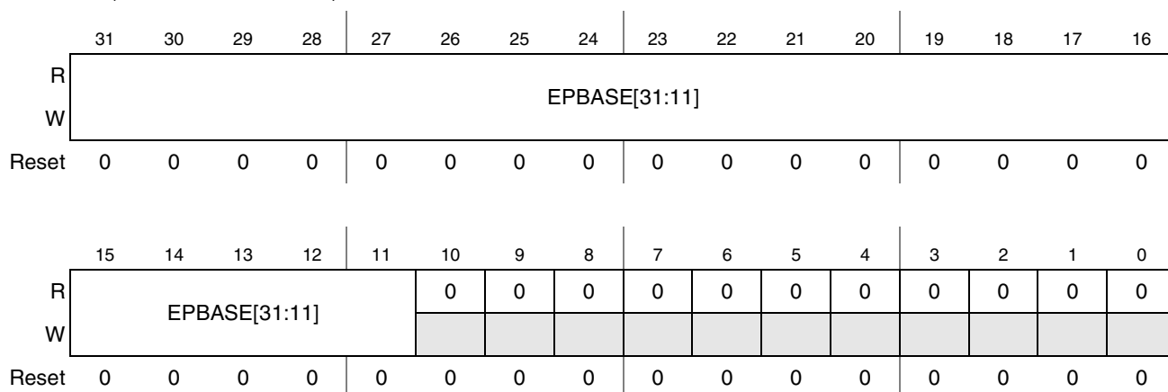
Figure 32-31. ENDPOINTLISTADDR—Device Controller Endpoint List Address
