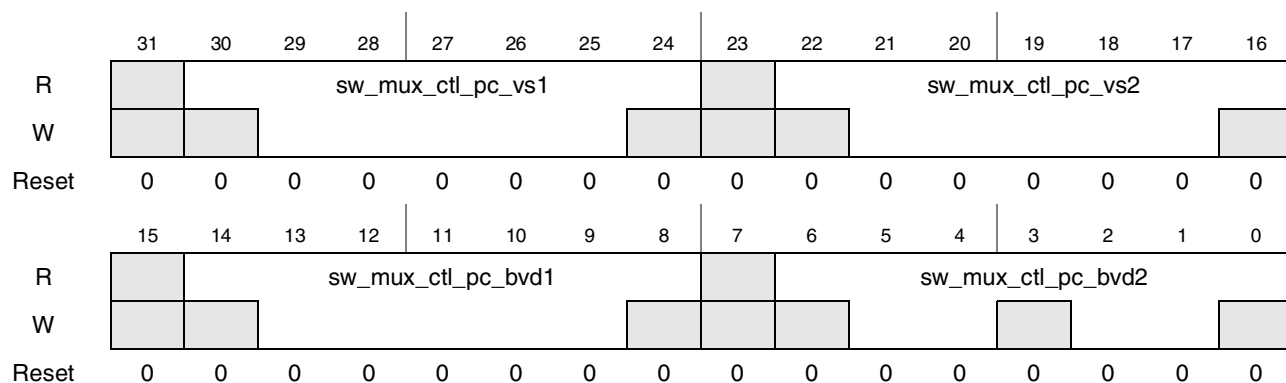
Figure 4-49. Register Description sw_mux_ctl_pc_vs1_pc_vs2_pc_bvd1_pc_bvd2
