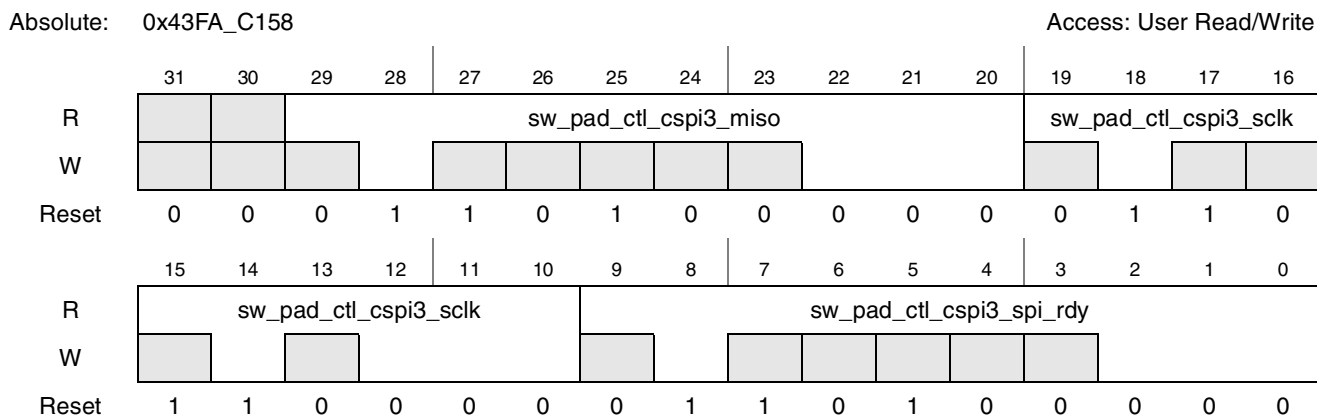
Figure 4-90. Register Description sw_pad_ctl_cspi3_miso_cspi3_sclk_cspi3_spi_rdy
