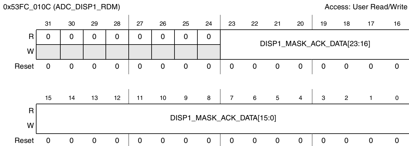
Figure 44-75. ADC Display 1 Read Mask Register (ADC_DISP1_RDM)
