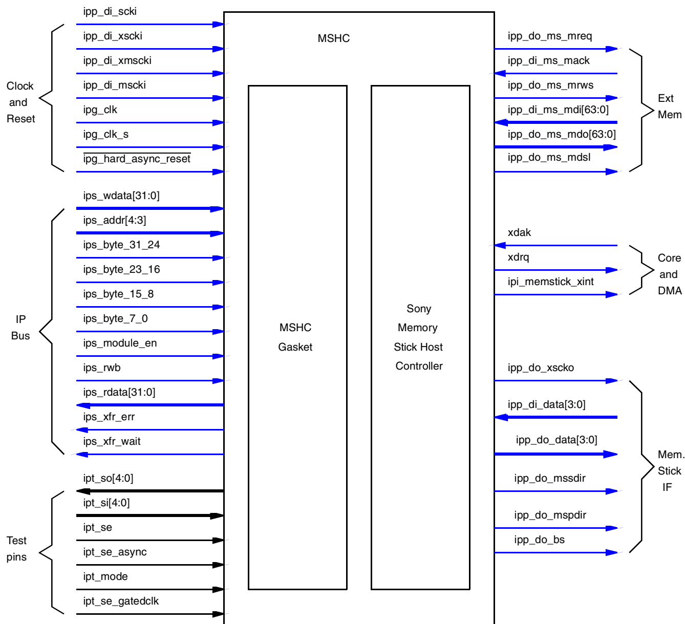
Figure 28-1. Applications Processor Memory Stick Controller Block Diagram
