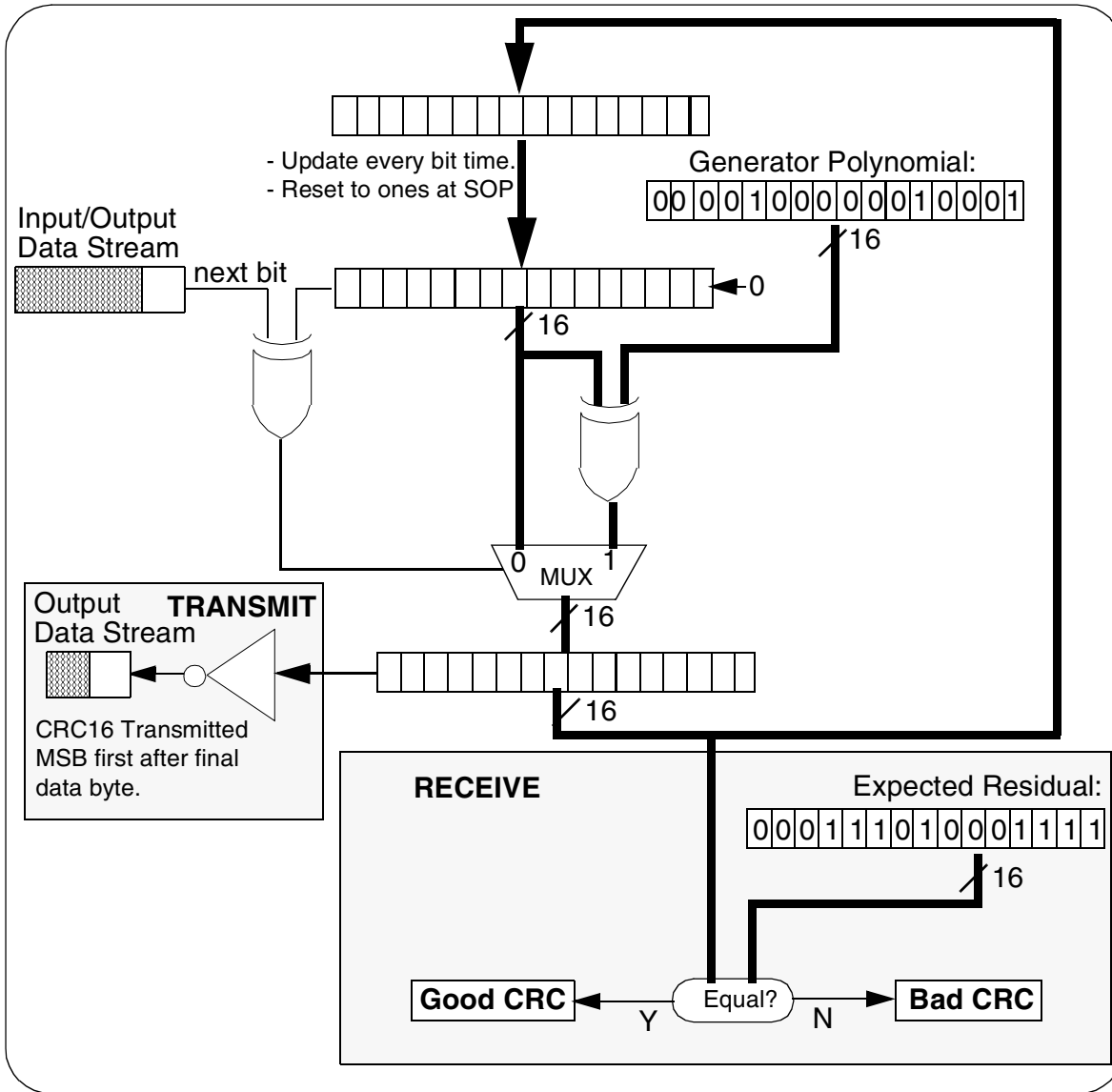
Figure 30-48. CRC Block Diagram
