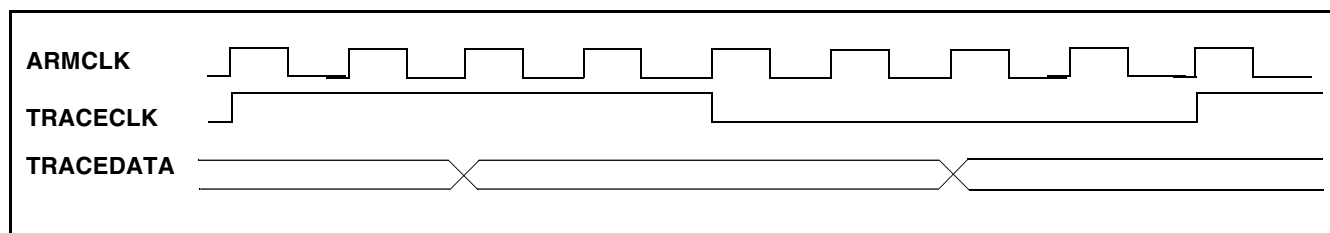
Figure 6-4. 1:4 Port Mode
