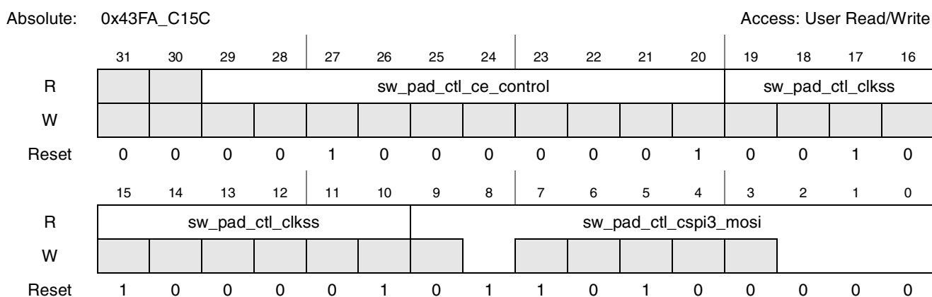
Figure 4-91. Register Description sw_pad_ctl_ce_control_clkss_cspi3_mosi
