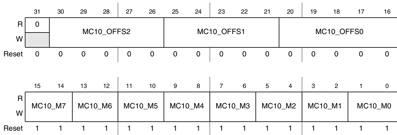
Figure 44-105. DI Display 1 Command Byte 0 Mapping Register (DI_DISP1_CB0_MAP)
