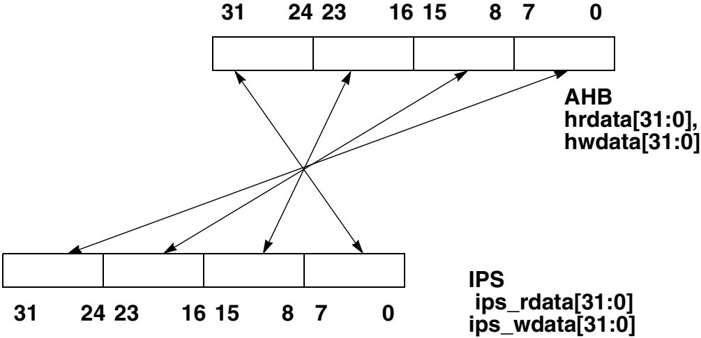
Figure 38-18. Data Bus Byte Lane Mapping for 32-Bit Peripherals, 32-Bit System, aips_byte_config[1:0] = 00
