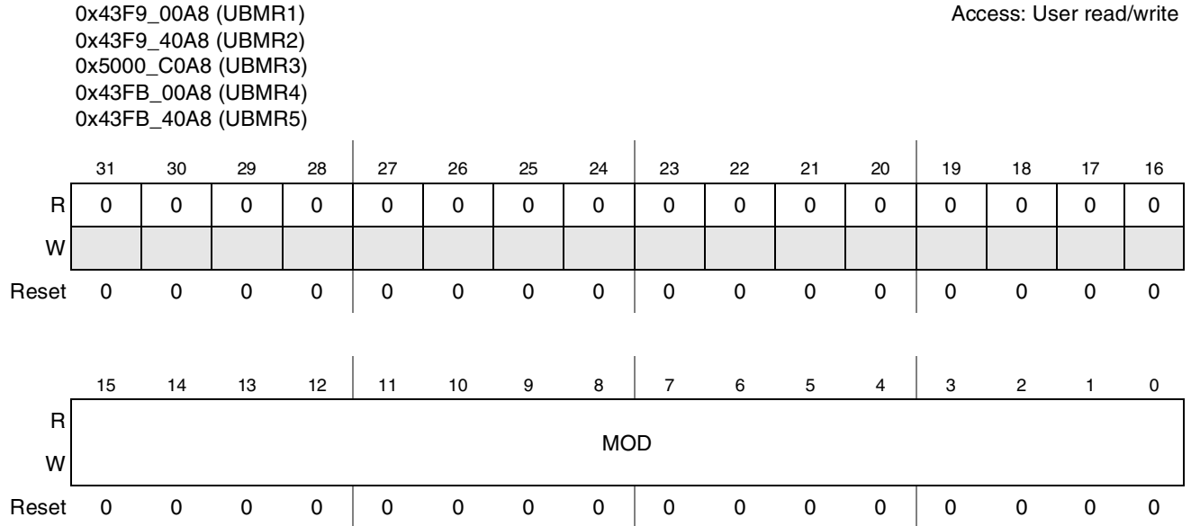
Figure 31-15. UART BRM Modulator Register
