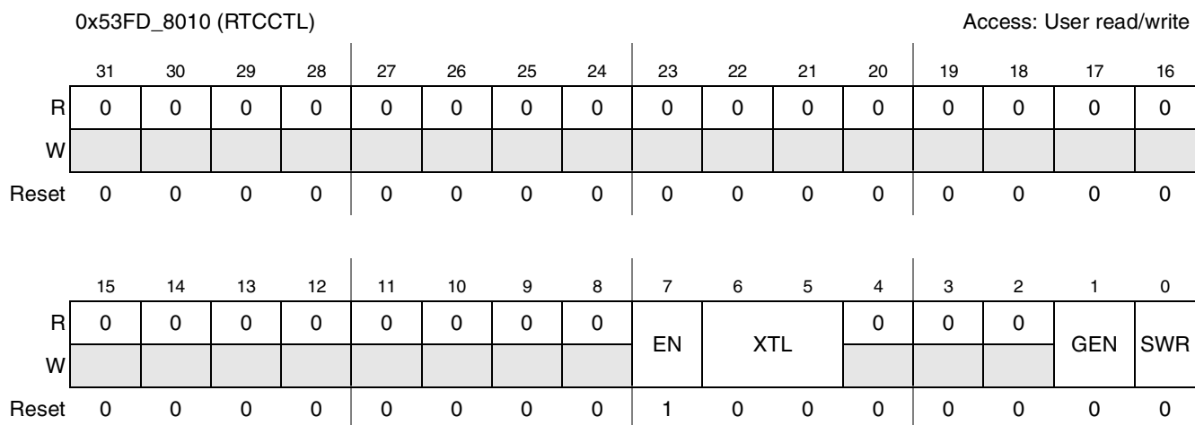
Figure 36-7. RTC Control Register
