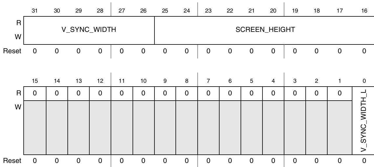
Figure 44-61. SDC Vertical Configuration Register (SDC_VER_CONF)
