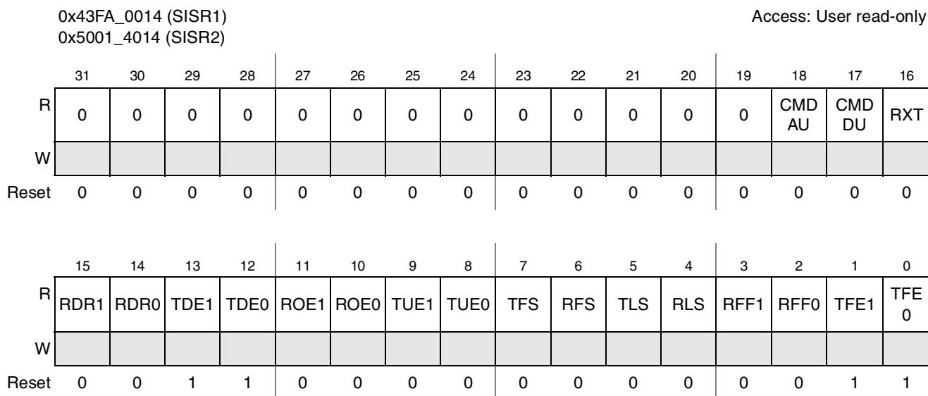
Figure 45-26. SSI Interrupt Status Register
