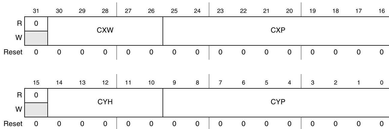
Figure 44-57. SDC Cursor Position Register (SDC_CUR_POS)
