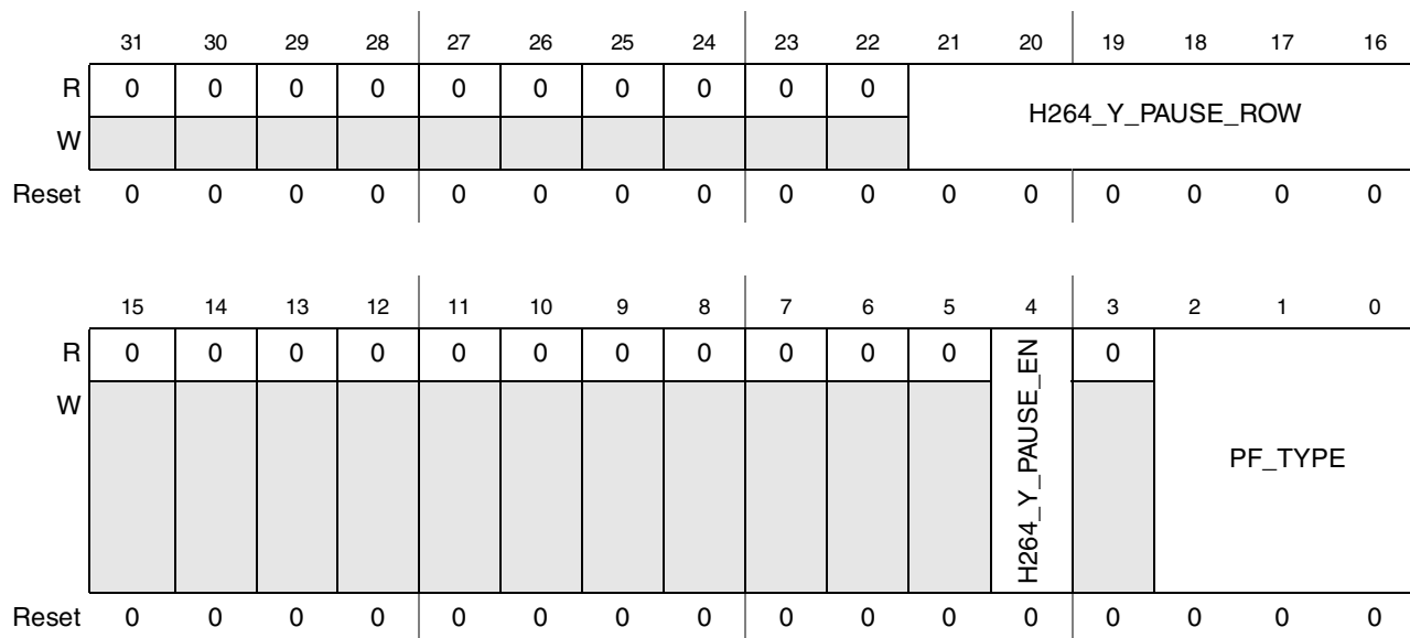
Figure 44-48. PF Configuration Register (PF_CONF)
