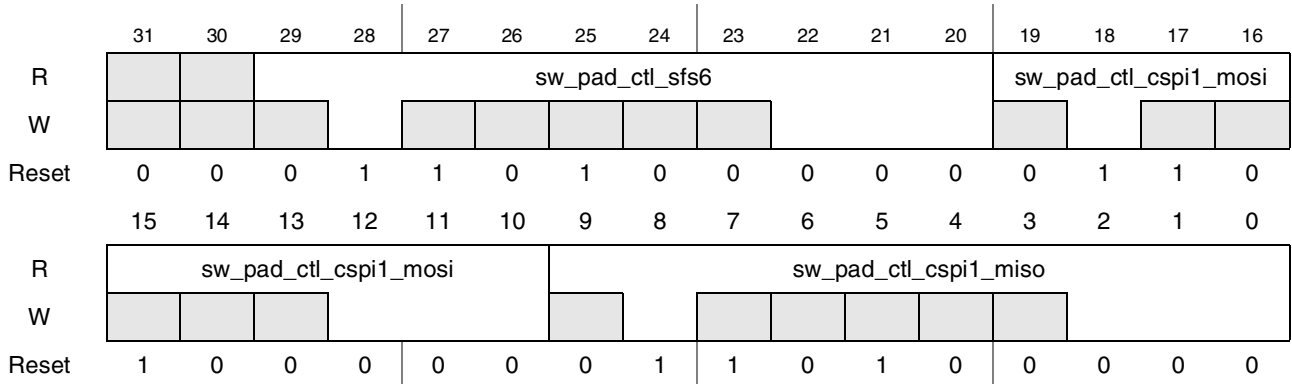
Figure 4-133. Register Description sw_pad_ctl_sfs6_csipi1_mosi_csipi1_miso
