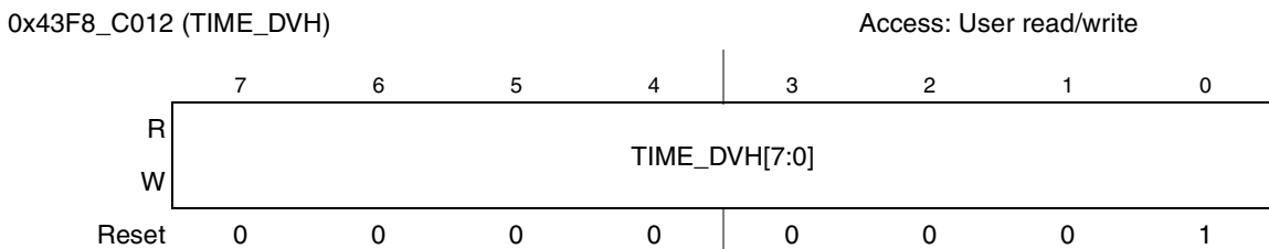
Figure 23-31. TIME_DVH Register
