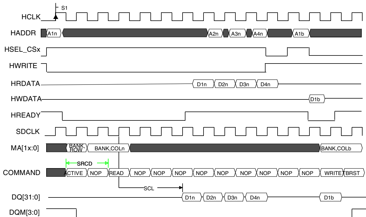
Figure 19-68. SDR Burst Read Followed by On-Page Write Timing Diagram
