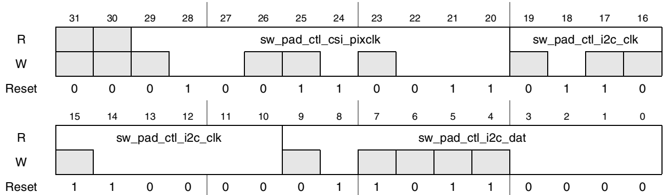
Figure 4-139. Register Description sw_pad_ctl_csi_pixclk_i2c_clk_i2c_dat
