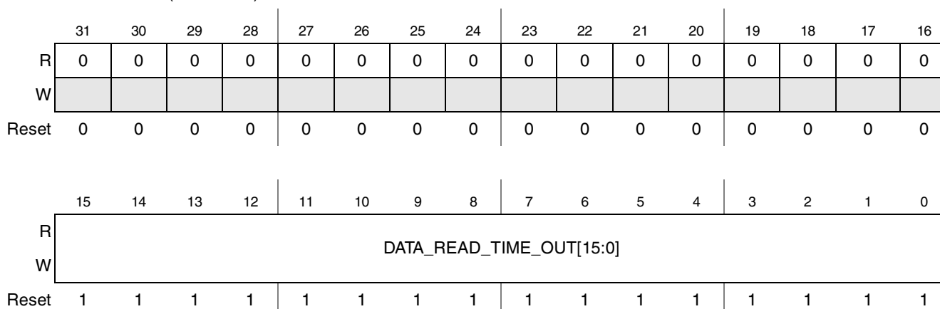
Figure 29-9. SDHC Read Time Out Register
