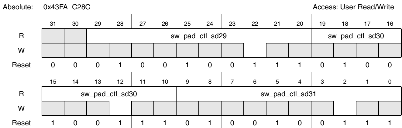
Figure 4-167. Register Description sw_pad_ctl_sd29_sd30_sd31
