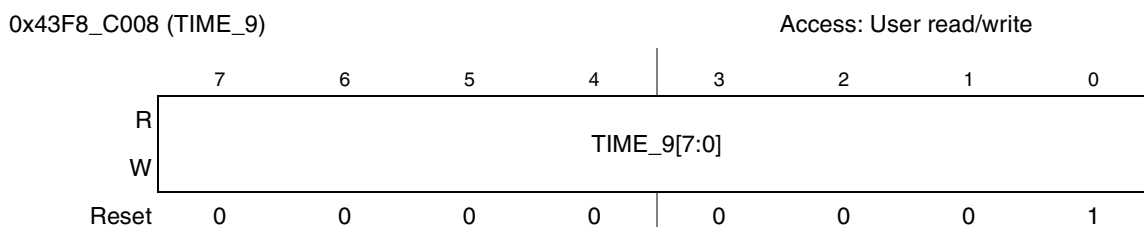
Figure 23-21. TIME_9 Register
