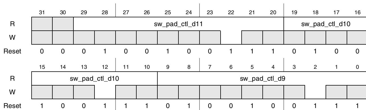
Figure 4-153. Register Description sw_pad_ctl_d11_d10_d9
