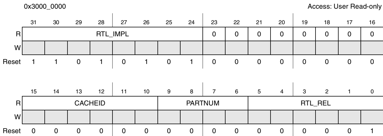
Figure 14-7. ID Register
