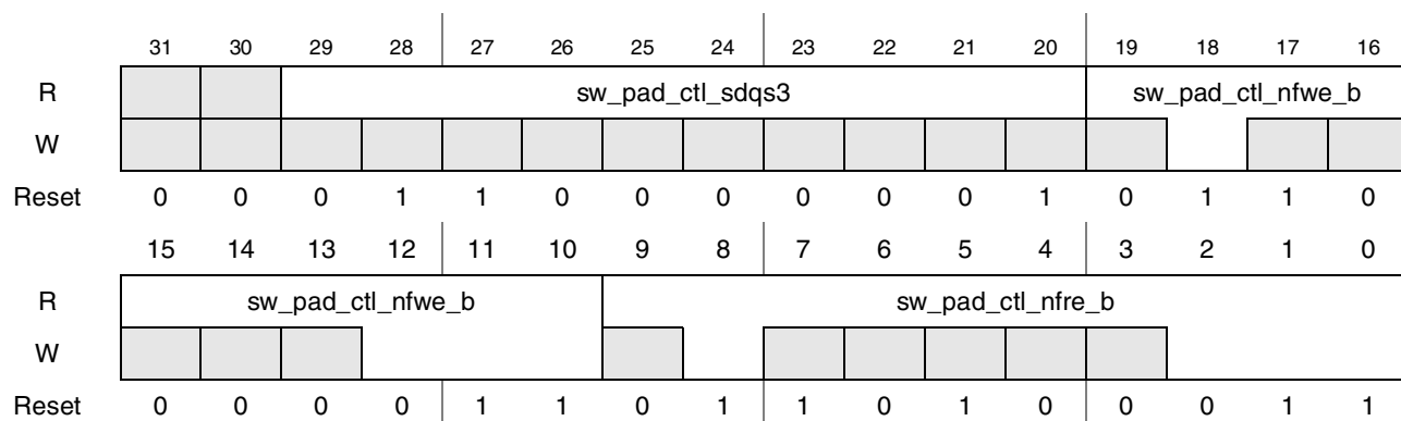
Figure 4-157. Register Description sw_pad_ctl_sdqs3_nfwe_b_nfre_b
