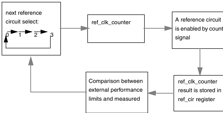
Figure 3-36. FSM Control Loop
