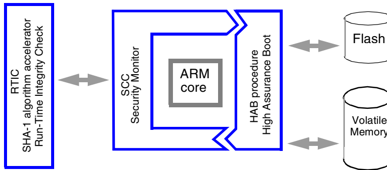
Figure 1-9. Boot Components
