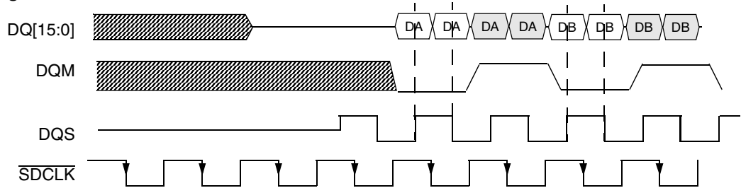
Figure 19-57. LPDDR Off-Page Write Followed by On-Page Write Timing Diagram
