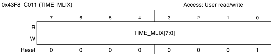
Figure 23-30. TIME_MLIX Register
