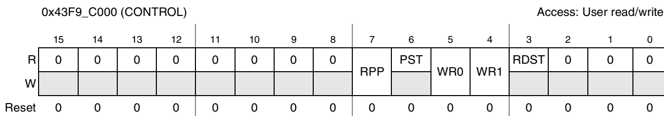
Figure 22-4. Control Register
