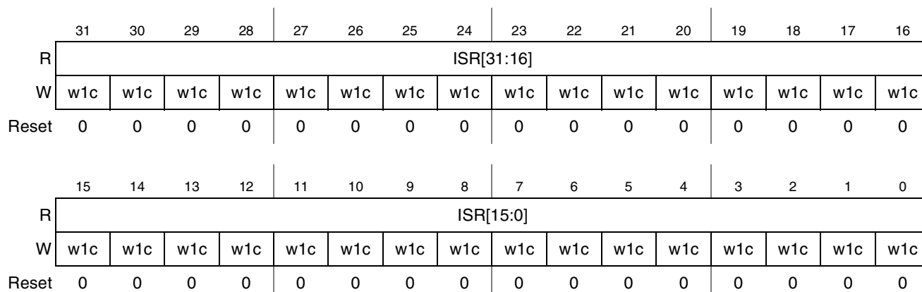
Figure 5-10. GPIO Interrupt Status Register (ISR)
