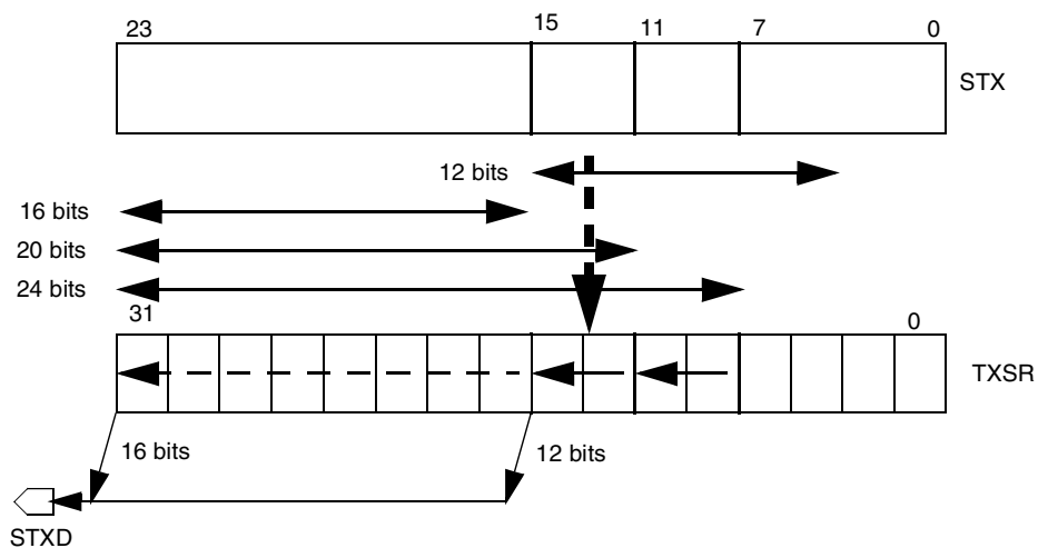
Figure 45-14. Transmit Data Path (TXBIT0=0, TSHFD=0) (MSB Alignment)
