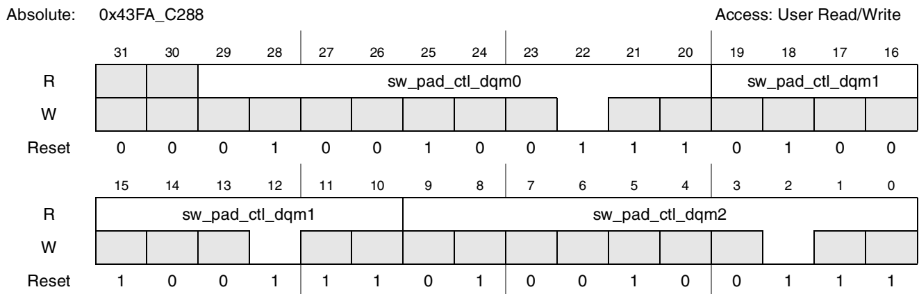
Figure 4-166. Register description sw_pad_ctl_dqm0_dqm1_dqm2
