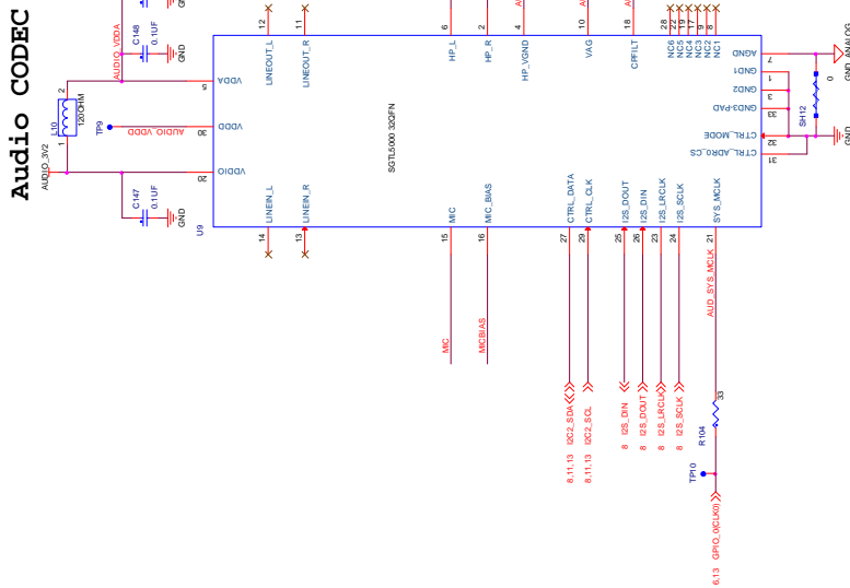
Figure 50. MX53 AUDIO
