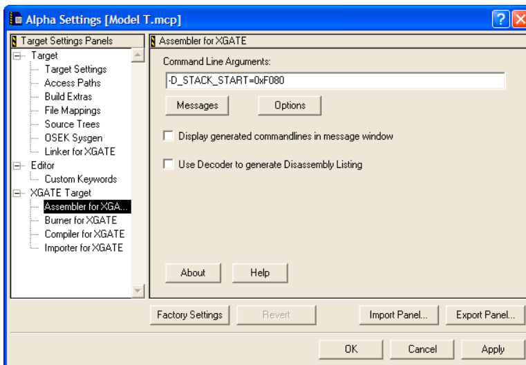
Figure 1.36 Assembler for XGATE Preference Panel
