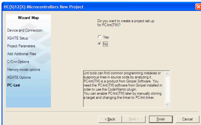
Figure 1.7 PC-Lint Page
