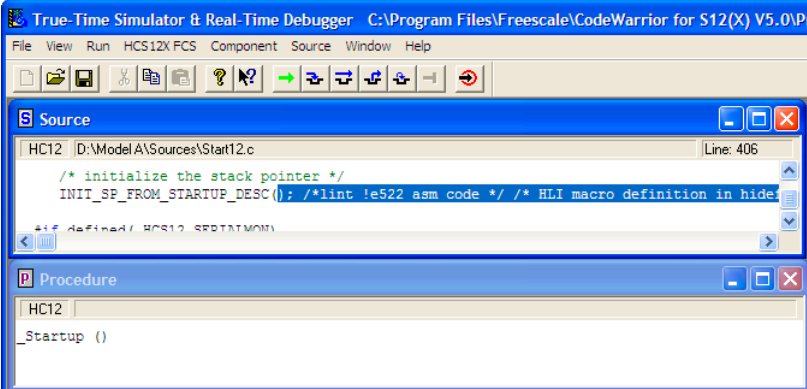
Figure 1.33 Simulator Startup
