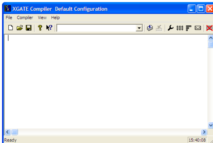
Figure 1.21 XGATE Compiler
