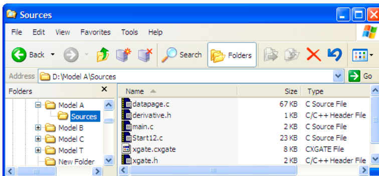
Figure 1.25 Project Files
