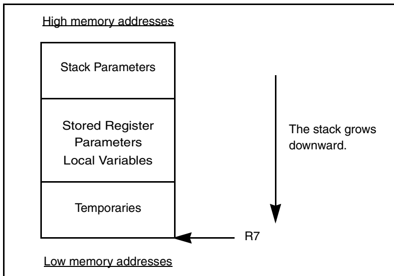
Figure 10.1 Normal Function Stack Frame
