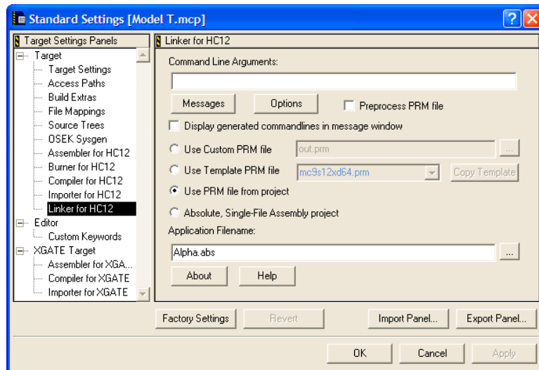
Figure 1.17 Linker for HC12 Preference Panel
