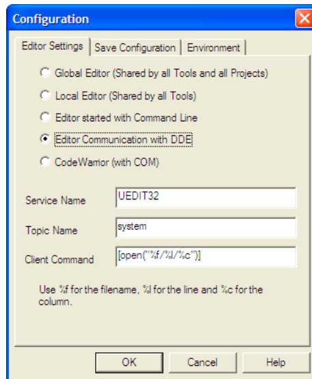
Figure 2.13 Editor Started with DDE (UltraEdit-32)
