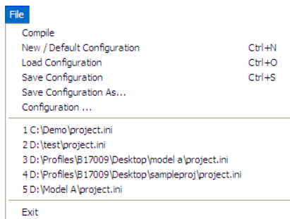
Figure 2.8 File Menu
