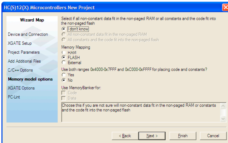
Figure 1.5 Memory Model Options Page
