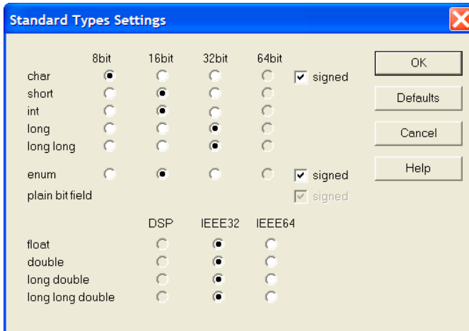
Figure 5.3 Standard Types Settings Dialog Box
