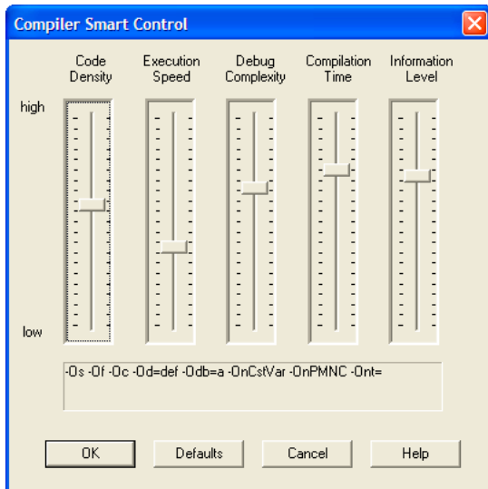
Figure 2.22 Compiler Smart Control Dialog Box
