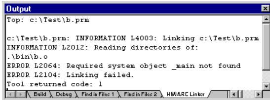
Figure 1.42 Visual Output Window
