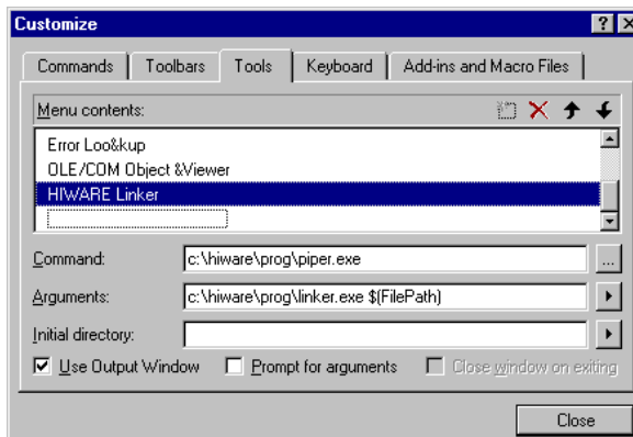
Figure 1.41 Customize Dialog Box
