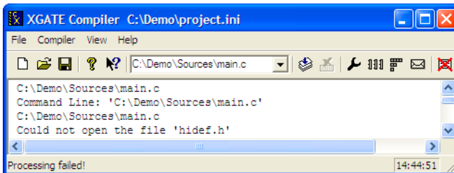
Figure 2.2 Main Window
