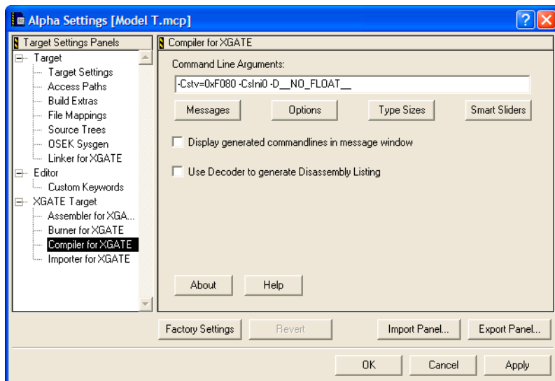
Figure 1.38 Compiler for XGATE Preference Panel
