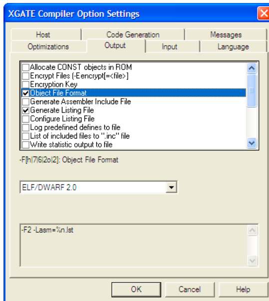
Figure 1.24 Compiler Option Settings Dialog Box
