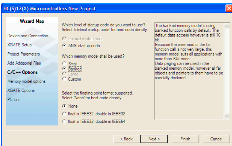
Figure 1.4 C/C++ Options Page
