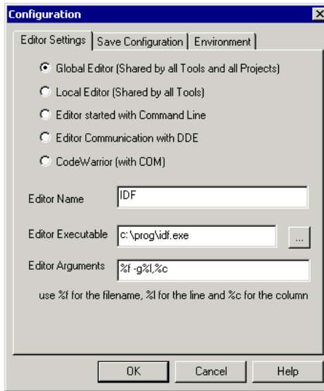
Figure 2.9 Global Editor Configuration
