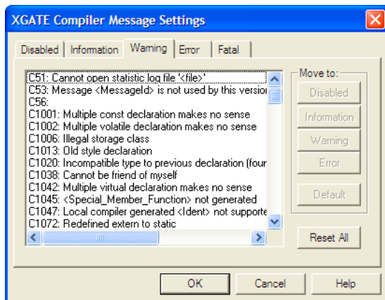
Figure 5.2 XGATE Compiler Message Settings Dialog Box
