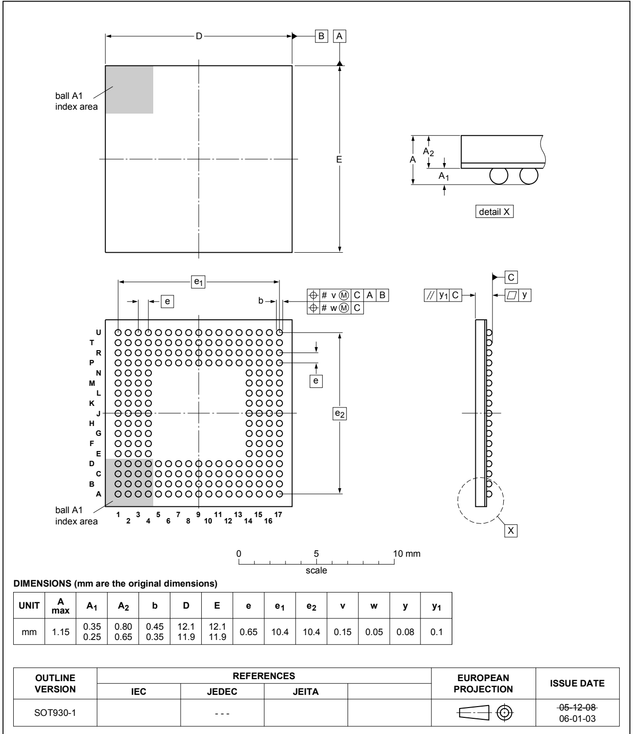
Fig. 1. Package outline TFBGA208 (SOT930-1)
