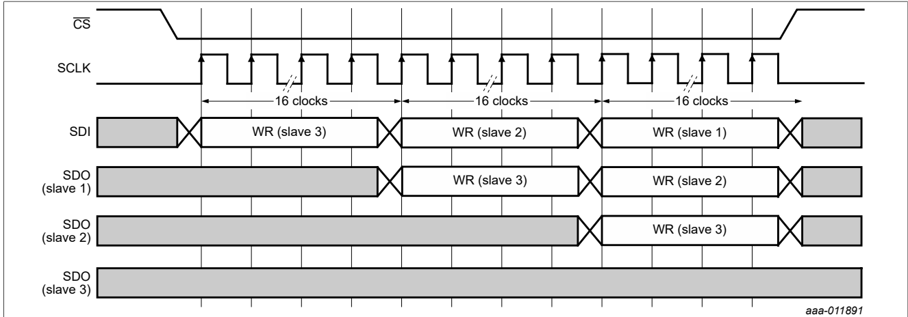
Figure 14. Write access
