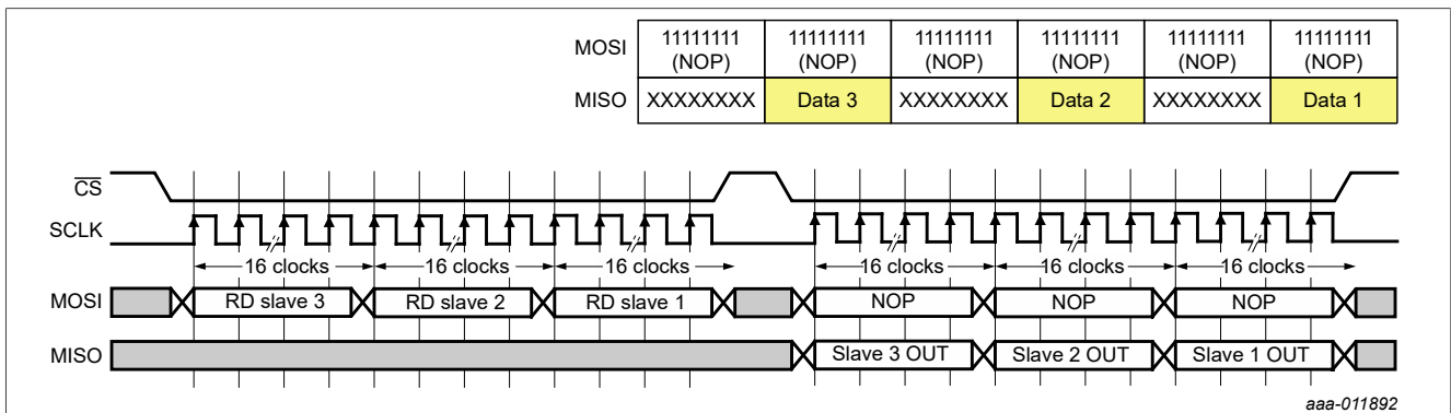
Figure 15. Read access
