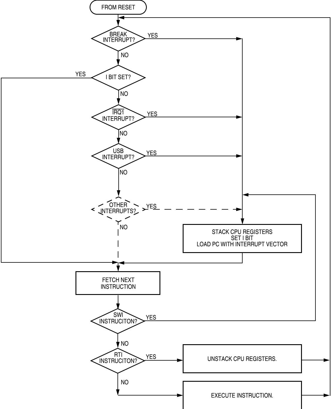
Figure 7-8. Interrupt Processing
