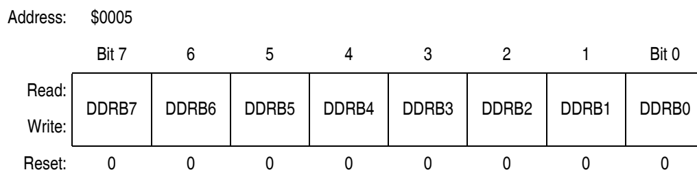
Figure 12-5. Data Direction Register B (DDRB)
