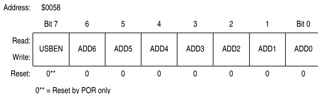
Figure 9-6. USB HUB Address Register (HADDR)
