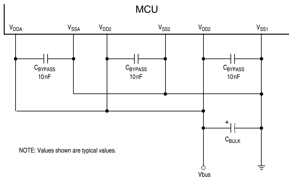
Figure 1-3. Power Supply Bypassing
