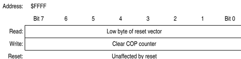
Figure 13-3. COP Control Register (COPCTL)
