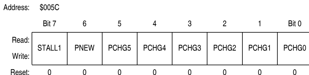
Figure 9-9. USB HUB Control Register 1 (HCR1)
