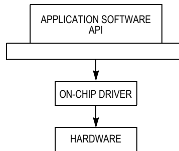
Figure 3. Software Structure
