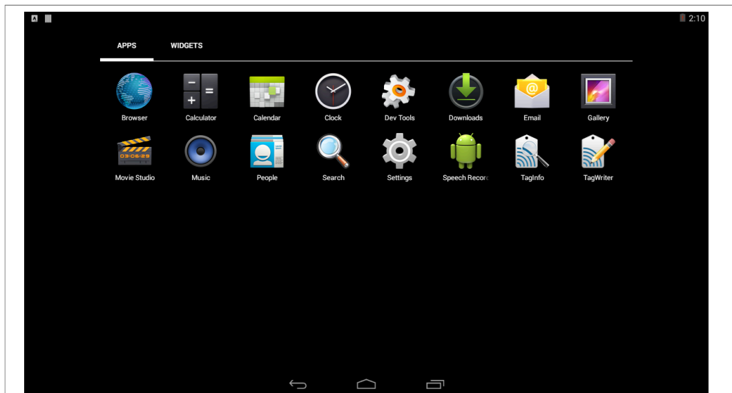
Figure 13. Android applications
